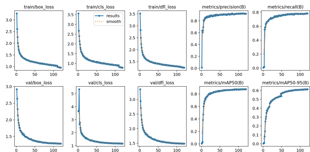
Figure 6. Convergence curves of YOLOv8n-improved.
