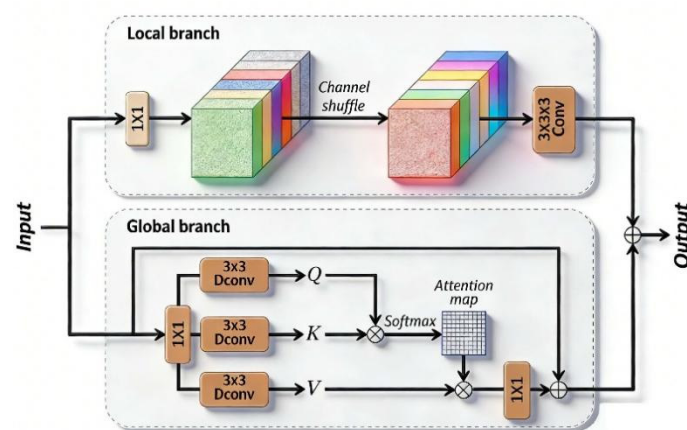
Figure 3. Structure of the convolution–attention fusion module.
