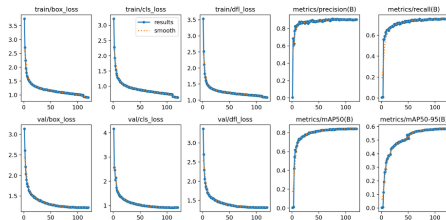
Figure 5. Convergence curves of YOLOv8n.
