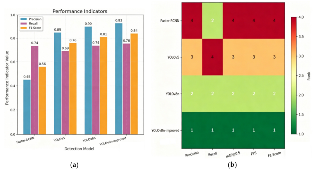
Figure 7. Comparison of results between the improved YOLOv8n and other models: (a) Performance evaluation comparison; (b) Ranking comparison results.
