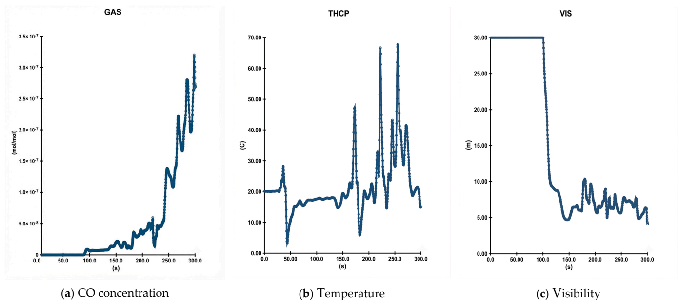
Figure 11. Line chart of fire data change over time at exit Node 15.
