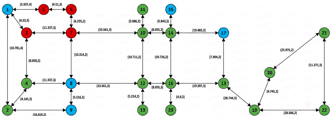
Figure 10. The topology diagram when the burning time t = 300 s.
