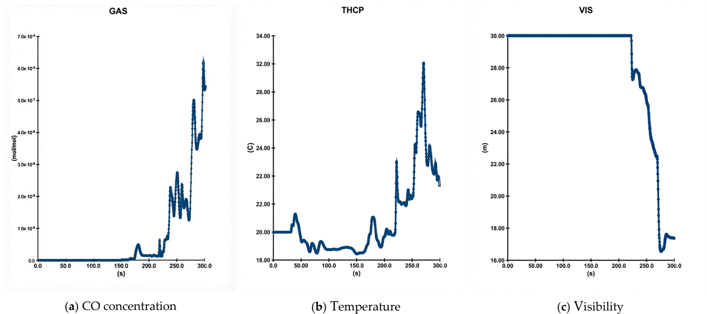
Figure 12. Manner line chart of fire data change over time at exit Node 23.
