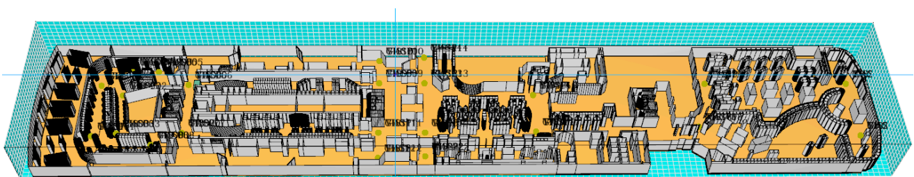
Figure 8. Fire simulation model of the bottom deck.
