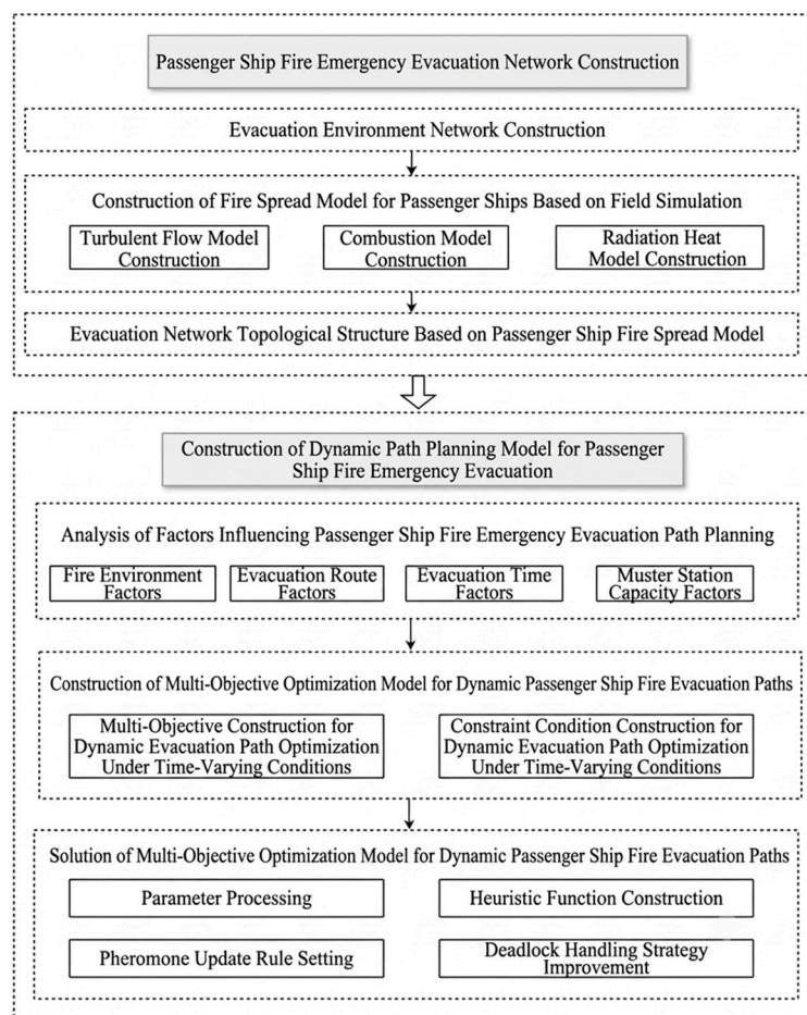
Figure 1. Technical roadmap.
