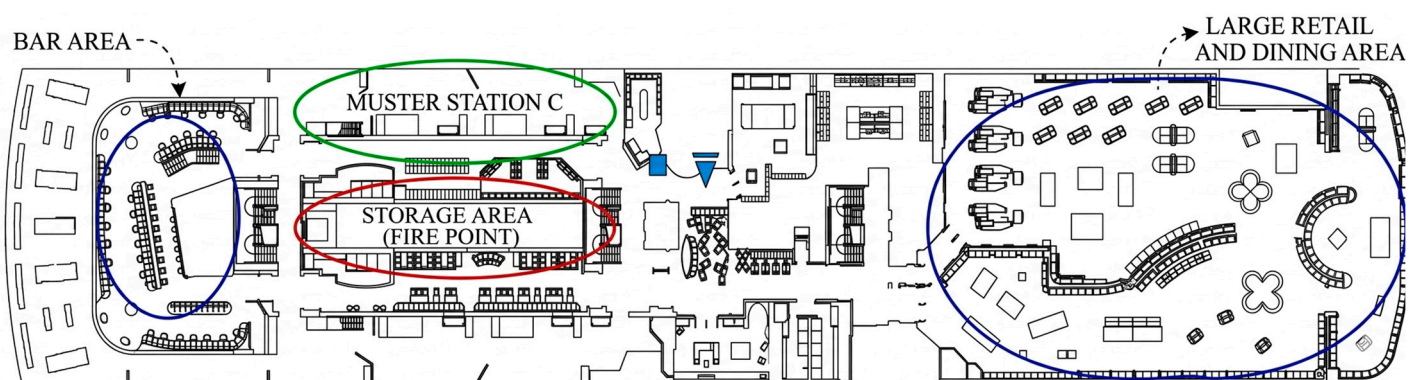
Figure 6. CAD drawing of the bottom deck.
