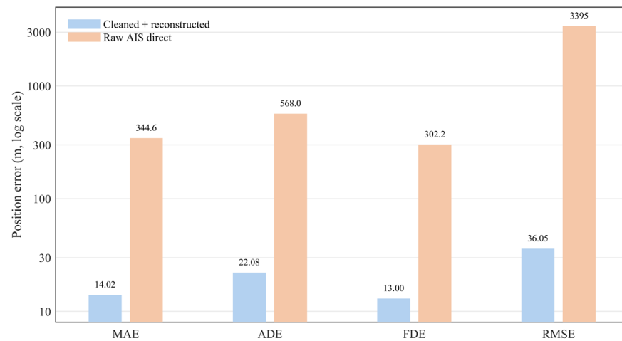
Figure 6. Preprocessing ablation study: comparison between raw-AIS direct training and the complete AIS preprocessing pipeline.
