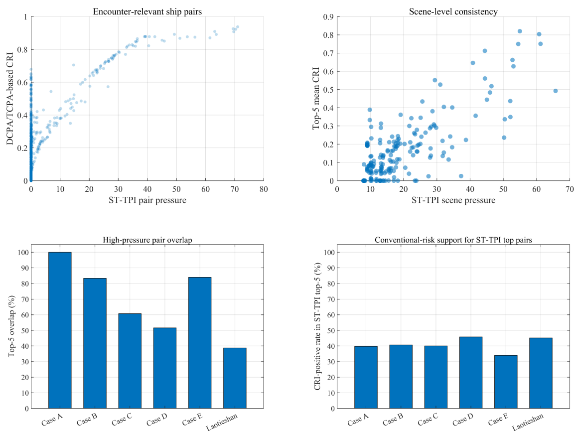
Figure 19. Consistency between ST-TPI and conventional encounter-risk indicators.
