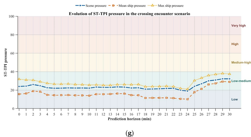
Figure 13. Predictive ST-TPI assessment results in the crossing encounter scenario. (a) A 5 min pressure snapshot; (b) 10 min pressure snapshot; (c) 15 min pressure snapshot; (d) 20 min pressure snapshot; (e) 25 min pressure snapshot; (f) 30 min pressure snapshot; (g) pressure-evolution curve.
