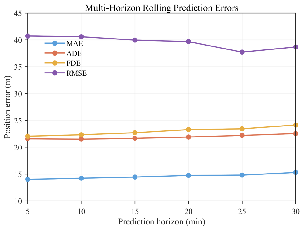
Figure 8. Variation in LSTM prediction errors under different observation-updated rolling evaluation horizons.
