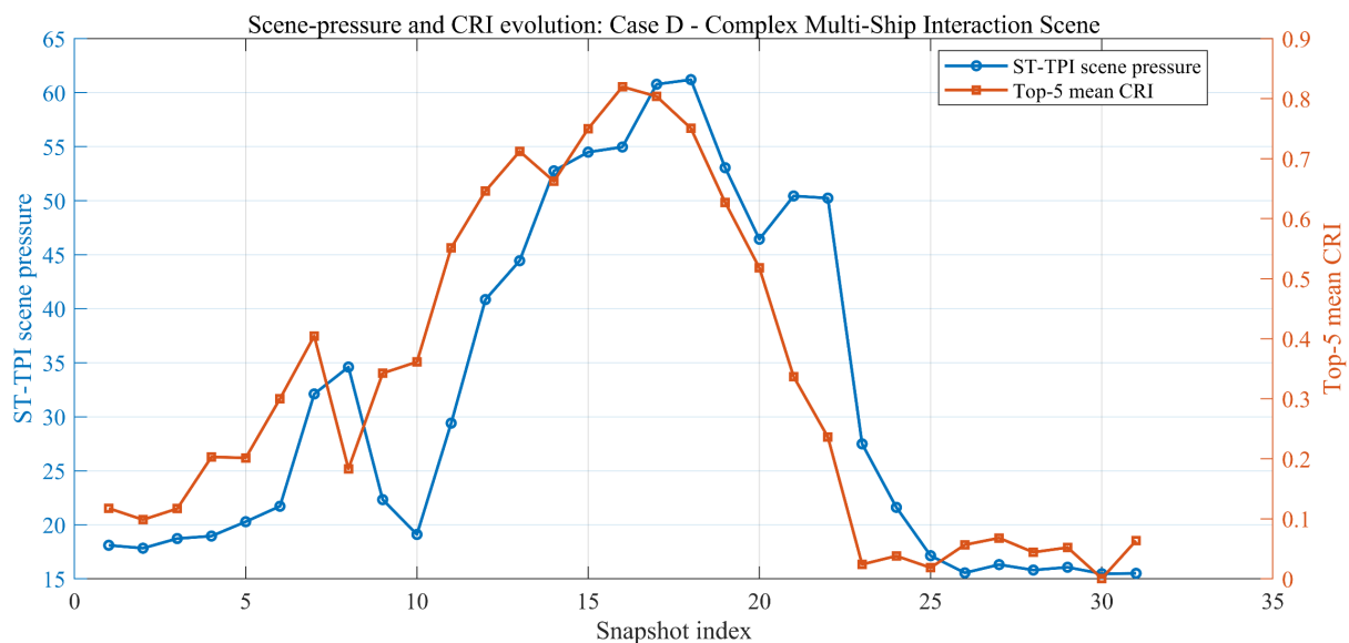
Figure 20. Time-series comparison between ST-TPI scene pressure and top-5 mean CRI in the complex multi-ship interaction scenario.
