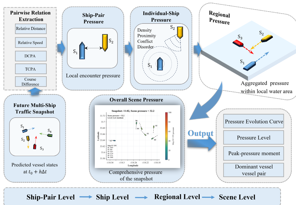
Figure 5. ST-TPI-based multi-level traffic pressure evaluation framework.
