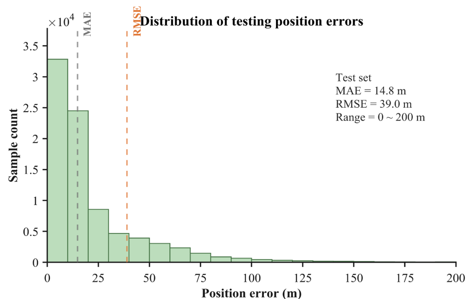
Figure 9. Distribution of position prediction errors on the testing subset.
