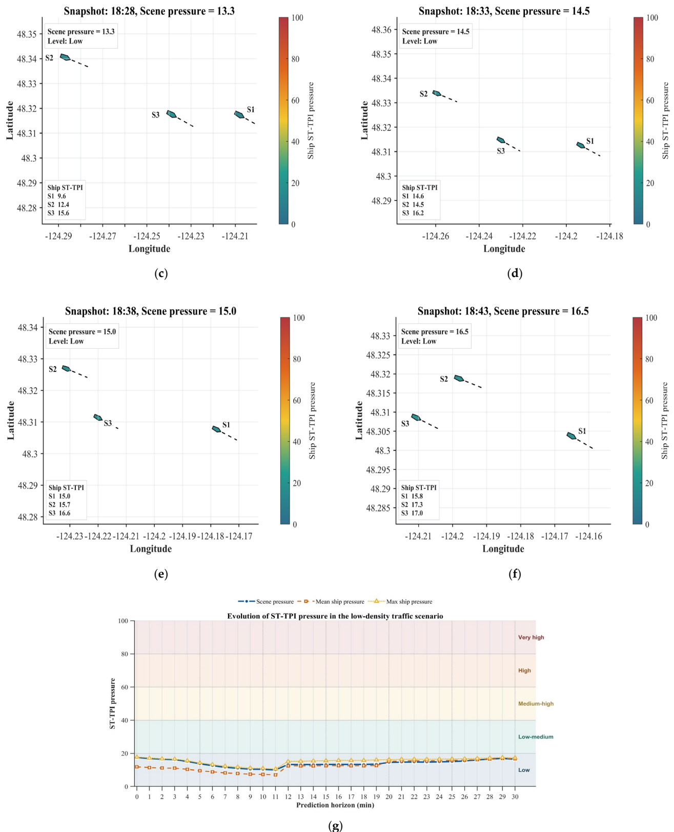
Figure 11. Predictive ST-TPI assessment results in the low-density traffic scenario. (a) A 5 min pressure snapshot; (b) 10 min pressure snapshot; (c) 15 min pressure snapshot; (d) 20 min pressure snapshot; (e) 25 min pressure snapshot; (f) 30 min pressure snapshot; (g) pressure-evolution curve.
