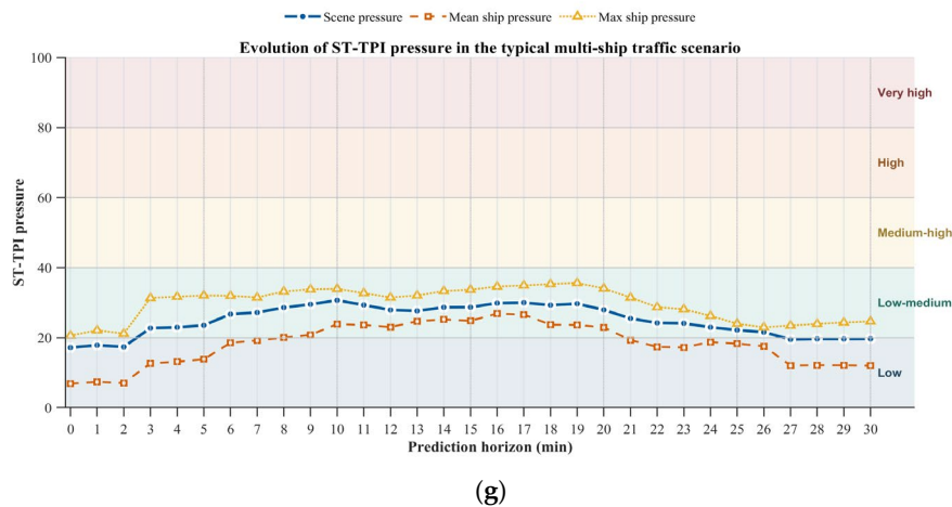
Figure 16. Predictive ST-TPI assessment results in the Laotieshan Channel real-waterway case. (a) A 5 min pressure snapshot; (b) 10 min pressure snapshot; (c) 15 min pressure snapshot; (d) 20 min pressure snapshot; (e) 25 min pressure snapshot; (f) 30 min pressure snapshot; (g) pressure-evolution curve.
