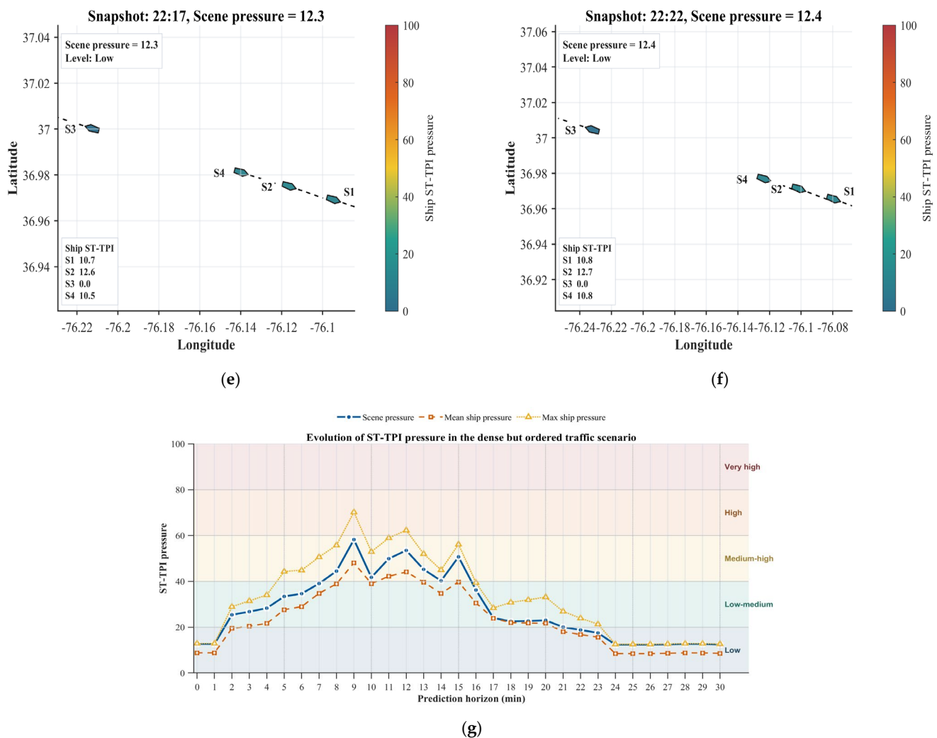
Figure 12. Predictive ST-TPI assessment results in the dense but ordered traffic scenario. (a) 5 min pressure snapshot; (b) 10 min pressure snapshot; (c) 15 min pressure snapshot; (d) 20 min pressure snapshot; (e) 25 min pressure snapshot; (f) 30 min pressure snapshot; (g) pressure-evolution curve.
