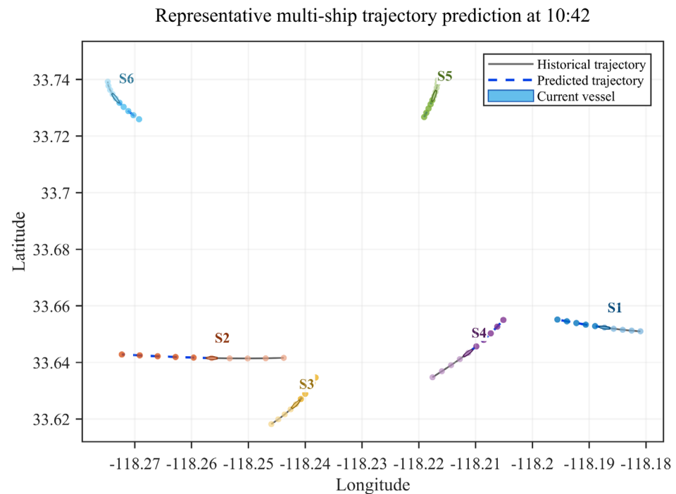
Figure 10. Visualization of representative multi-ship trajectory prediction at the 15 min horizon.
