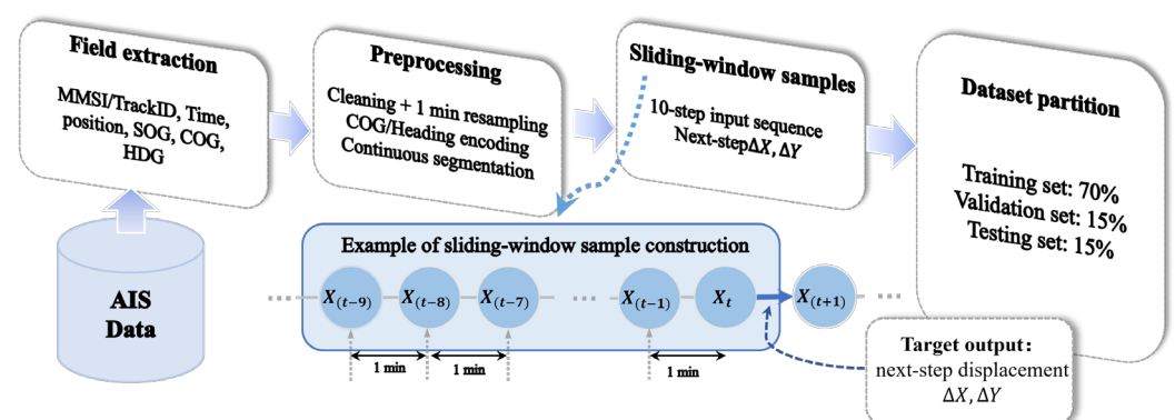
Figure 3. Workflow of AIS data preprocessing and continuous trajectory sample construction.
