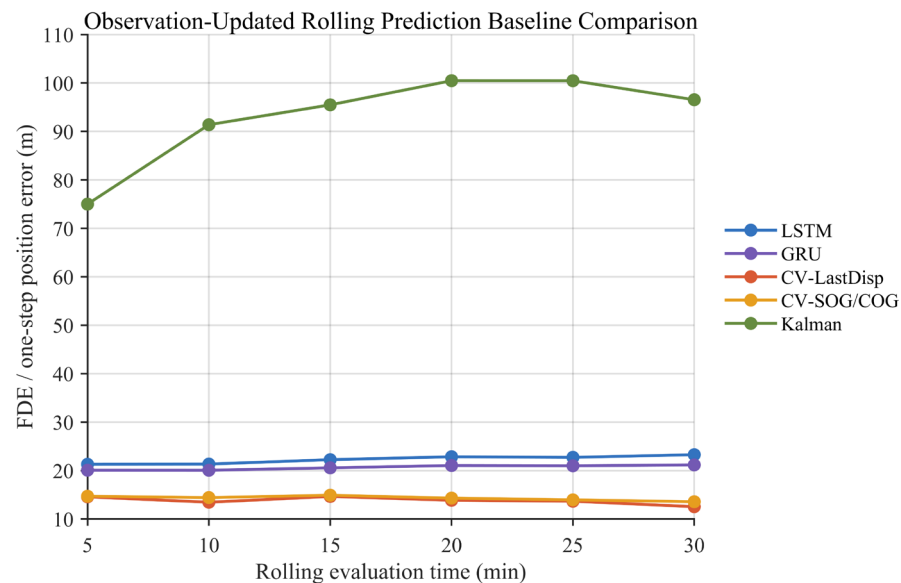
Figure 7. FDE comparison of different short-term prediction methods under observation-updated rolling evaluation.
