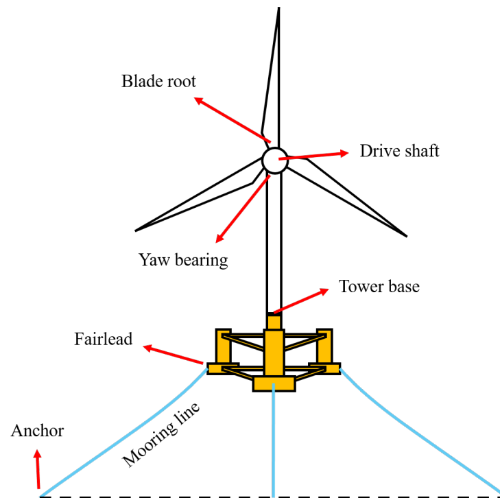
Figure 3. Turbine components and locations for fatigue analysis.
