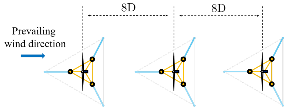
Figure 1. The top view of the FOWF for fatigue load analysis. The wind turbines in this figure are at the installation locations, i.e., the locations for the no-wind case.
