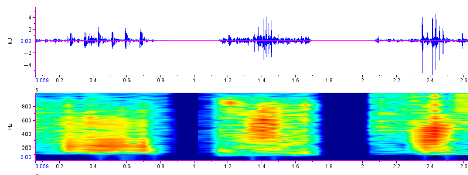
Figure 4. From left to right: waveform (top) and spectrogram (bottom) of one FPT sound from fuzzy cluster groups A, B, and C. The waveform shows amplitude over time; the spectrogram displays time (X), frequency (Y), and colour-coded amplitude (warm = higher energy, cool = lower). Analysis parameters: Hanning window, FFT size 512, frequency resolution 46.8 Hz.
