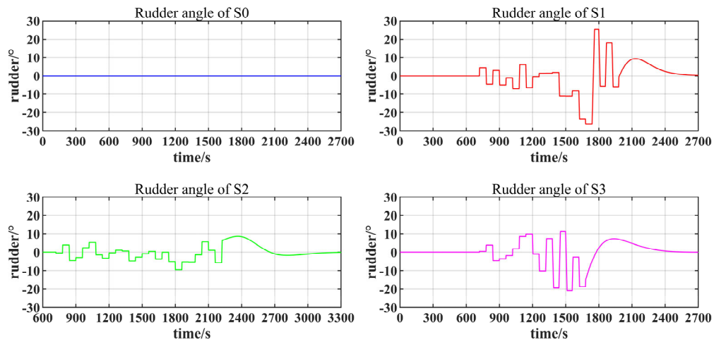
Figure 12. Rudder angle curves of each ship.
