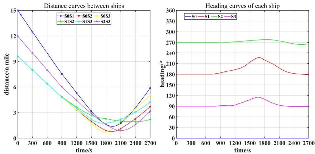
Figure 11. Curves of inter-ship distances and heading variations.
