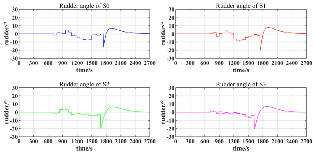
Figure 8. Rudder angle curves of each ship.
