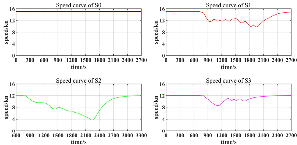
Figure 13. Speed curves of each ship.
