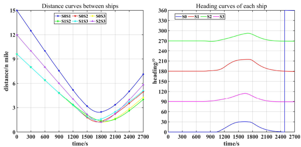
Figure 7. Curves of inter-ship distances and heading variations.
