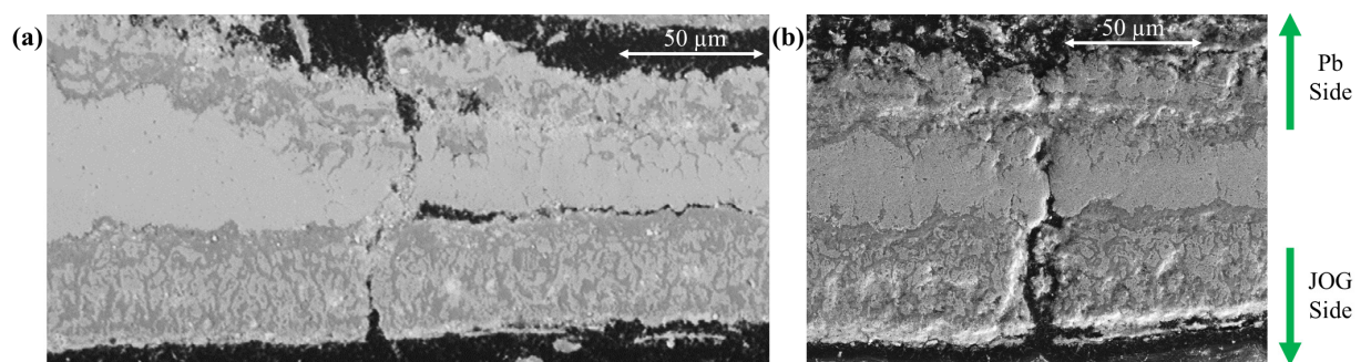
Figure 10. (a,b) Cross-section SEM images of two different notches that had cladding breaches with line fractures after 168 h exposure at 900^\circ\text{C} .
