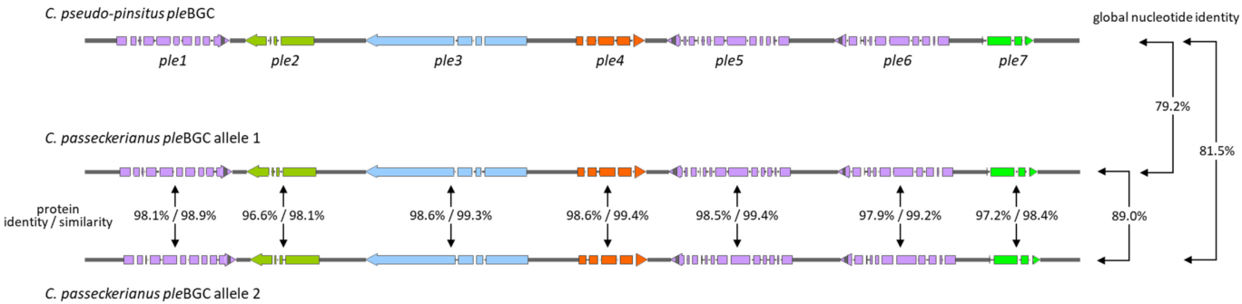
Figure 6. Pleuromutilin biosynthetic gene clusters ( pleBGCs ). Introns are illustrated as interruptions in the genes. Nucleotide identities and protein similarities/identities are indicated.
