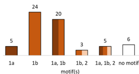
Figure 5. Number of predicted terpene synthases in C. passeckerianus with conserved motifs. 1a: class I motif DDXX(D/E); 1b: class I motif (N/D)DXX(S/T)XXE; 2: class II motif DXDD.
