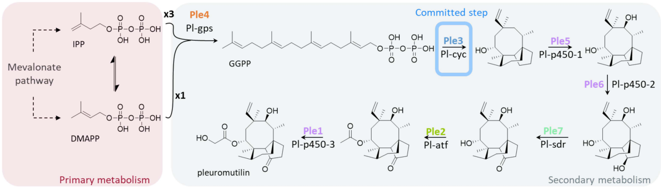
Figure 7. Pleuromutilin biosynthesis according to [16,17]. IPP: isopentenyl pyrophosphate; DMAPP: dimethylallyl diphosphate.
