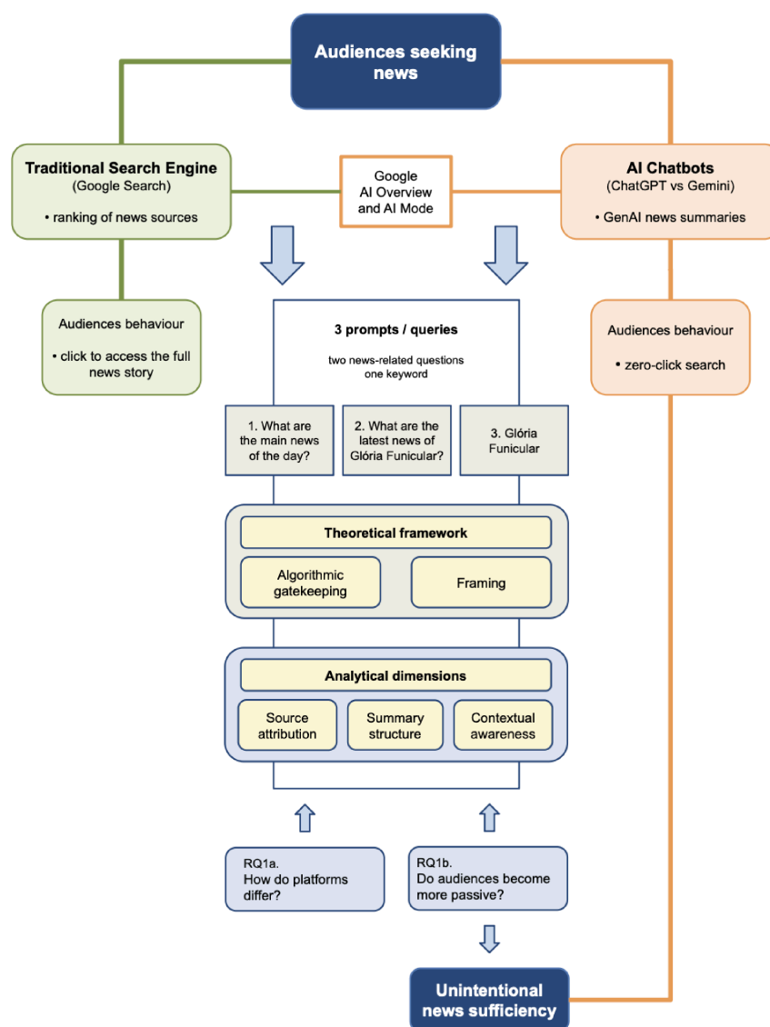
Figure 1. Analytical framework.
