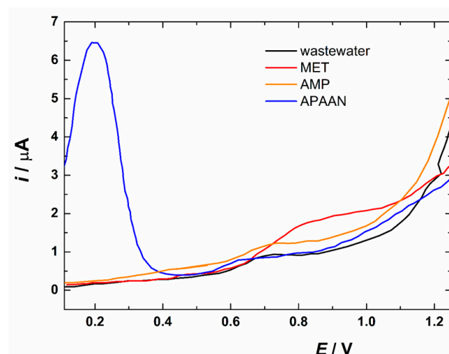
Figure 5. SWV response of filtered wastewater spiked with APAAN, AMP, and MET at a concentration of 1.5 \text{ mg L}^{-1} . The black curve shows the baseline response (non-spiked filtered wastewater). All conditions of SWV are the same as for MET detection in 3DP cell under the flow conditions ( 3.5 \text{ mL s}^{-1} ).
