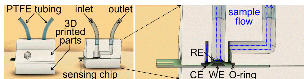
Figure 1. (left) Full and cross-sectional image of the cell designed and 3DP in this work. (right) Details of the channels and the screen-printed chip.
