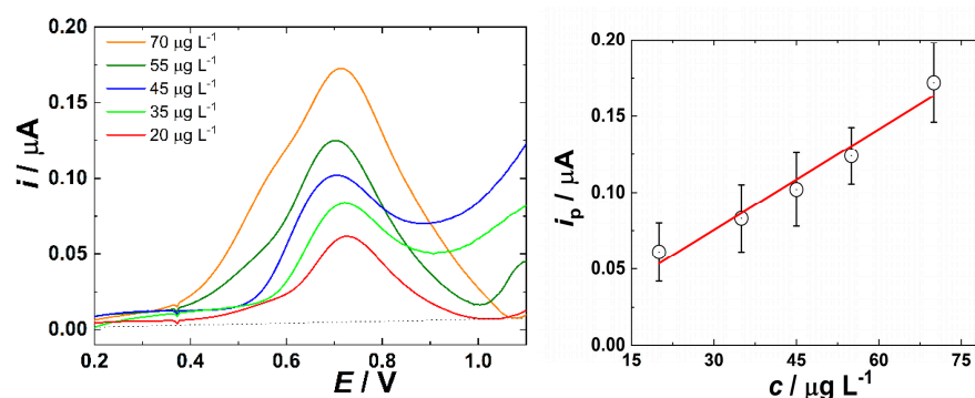
Figure 3. (left) SWVs of wastewater spiked with MET obtained in the 3DP flow cell developed in this work under stationary conditions after subtracting the curve measured without MET (background). (right) Dependence of faradaic peak current on MET concentration after background correction. SWV was performed using a frequency of 60 Hz, at an amplitude of 50 mV. Error bars represent the standard deviation across 3 independent replicate measurements.
