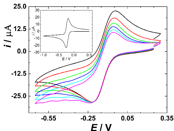
Figure 2. CV scans of 2 mM [\text{Ru}(\text{NH}_3)_6]\text{Cl}_3 in 3DP cell at various flow rates (from black to pink curve: 0.1; 0.7; 1.4; 2.1; 2.8; 3.5 \text{mL s}^{-1} ); scan rate of 0.1 \text{V s}^{-1} . Inset: CV obtained under no flow conditions at 0.1 \text{V s}^{-1} .
