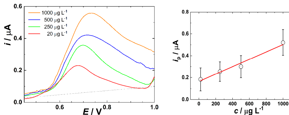
Figure 4. (left) SWVs of wastewater spiked with MET obtained in the 3DP flow cell developed in this work under flow conditions (sample flow rate of 3.5 \text{ mL s}^{-1} ) after subtracting the curve measured without MET (background). (right) Dependence of faradaic peak current on MET concentration after subtracting the curve measured without MET (background). SWV was performed using a frequency of 60 Hz, at an amplitude of 50 mV. Error bars represent the standard deviation across 3 independent replicate measurements.
