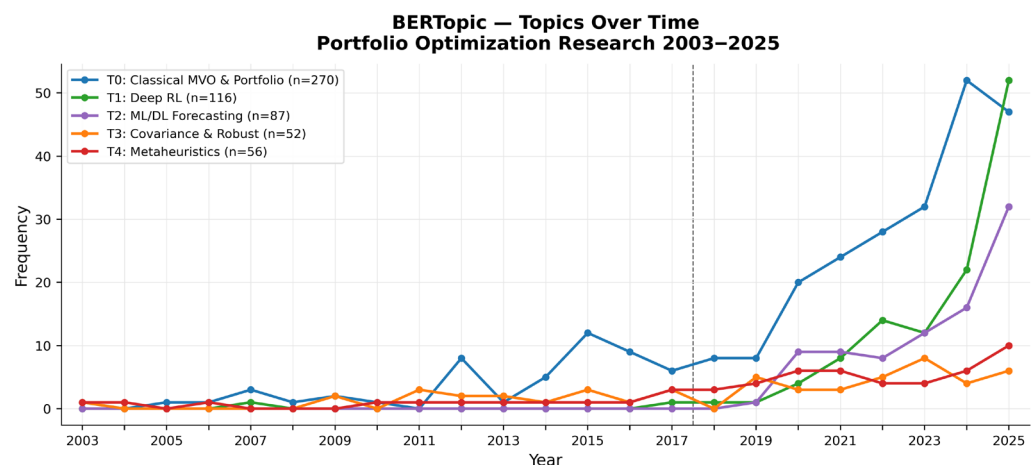
Figure 4. Temporal evolution of BERTopic topics, 2003–2025.
