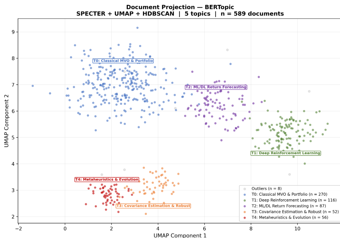
Figure 3. UMAP projection of SPECTER embeddings by topic assignment.
