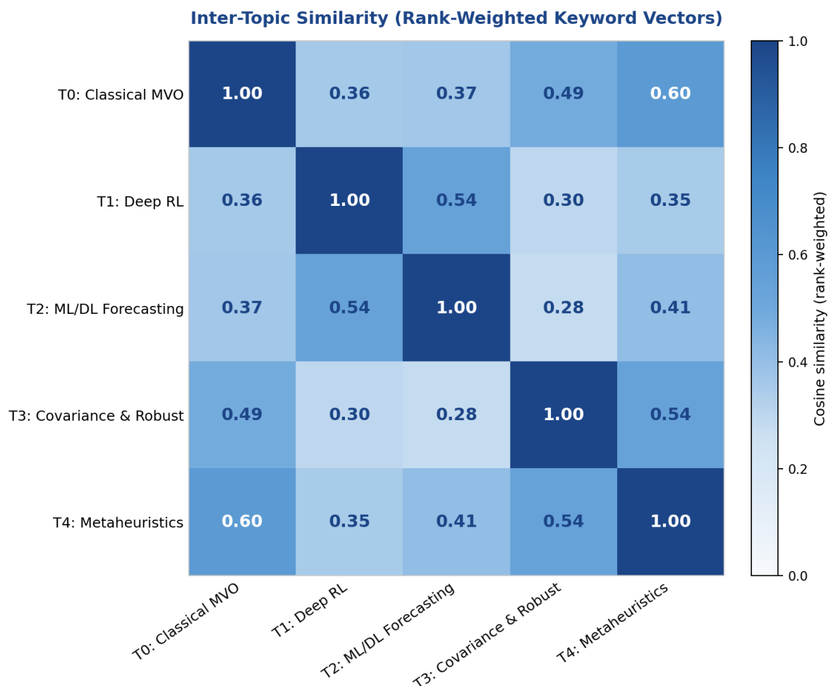
Figure 5. Rank-weighted inter-topic similarity matrix.
