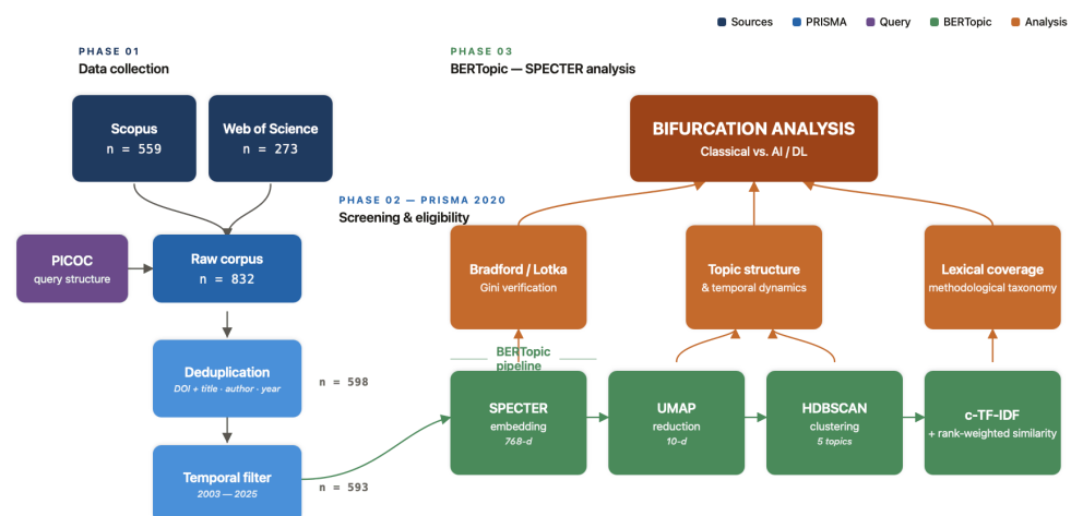
Figure 2. Methodological pipeline overview.
