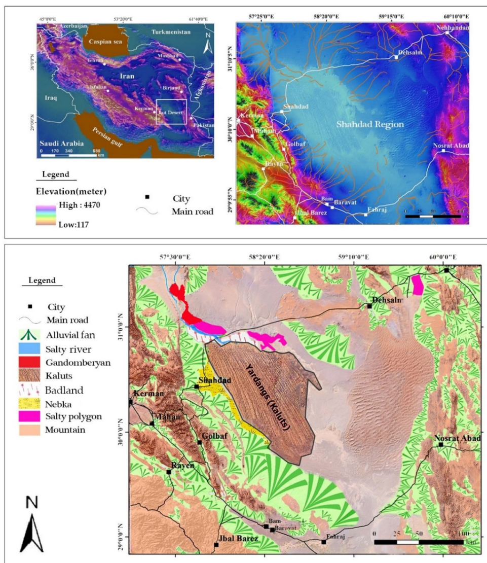
Figure 1. Map showing the position of geosites and geomorphosites in the study of the Shahdad region. In the medallions are satellite images of the position of the Lut Desert in Iran ( top left ) and the Shahdad region in which the study area is located ( top right ). (Source: Authors).
