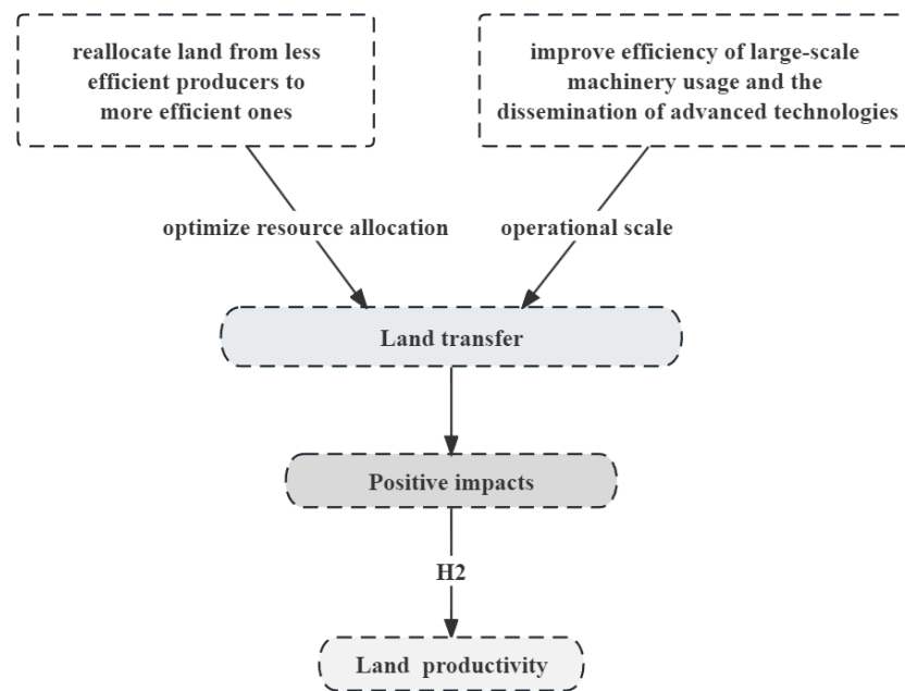
Figure 2. Theoretical mechanism for land transfer affecting land productivity.
