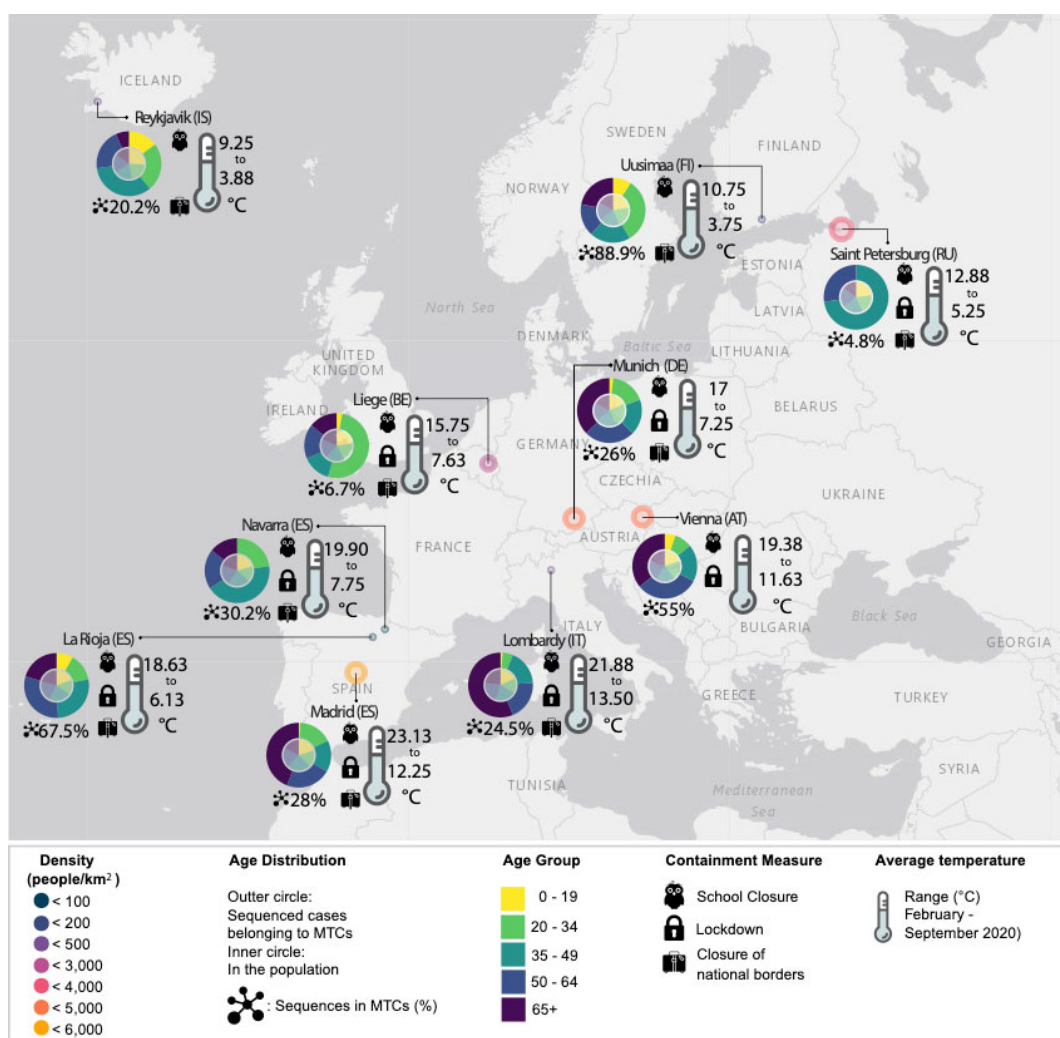
Figure 2. Distribution of total sequenced cases (five-color inner circle) and clustered sequences (belonging to MTCs – outer circle) according to age group. Density of population, containment measures, total levels of clustering and averages temperature range for each geographical region are also presented.
