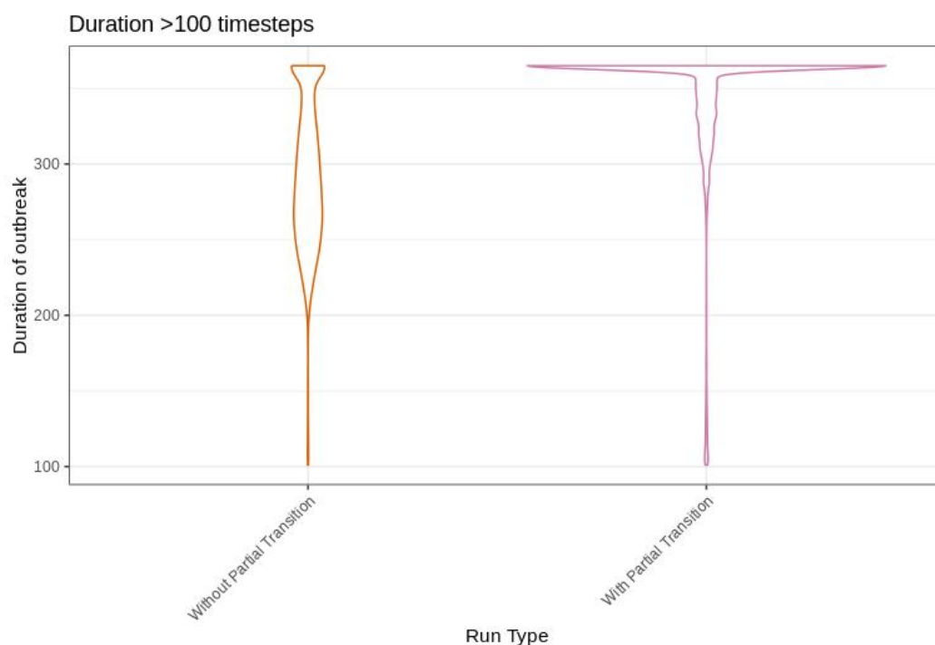
Figure 1. Duration of outbreak simulations with partial transition off (orange, left) and on (pink, right) for outbreaks lasting longer than 100 days.
