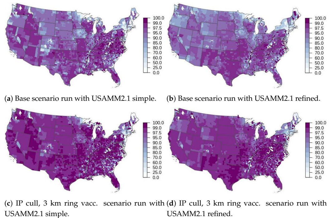
Figure 3. Counties colored by the proportion of focal (non-shipment) transmission for base scenarios (a,b) and cull and 3 km ring vaccination scenarios (c,d) run with USAMMv2.1 simple (a,c) and USAMMv2.1 refined (b,d).
