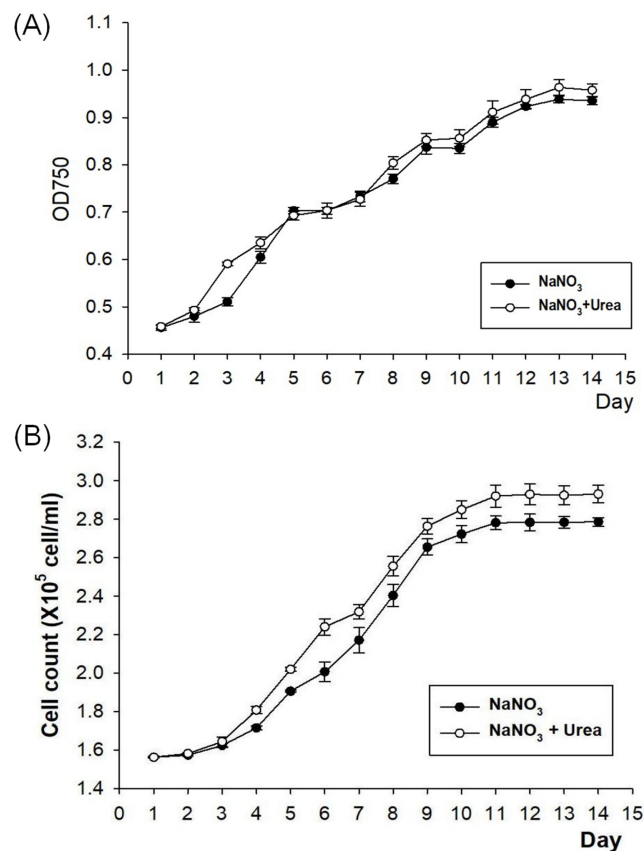
Figure 1. Growth curves of N. oceanica under two different conditions. Optical density (A) and cell count (B) of N. oceanica under two different conditions. Values shown as mean \pm standard deviation (SD) of three biological replicates.
