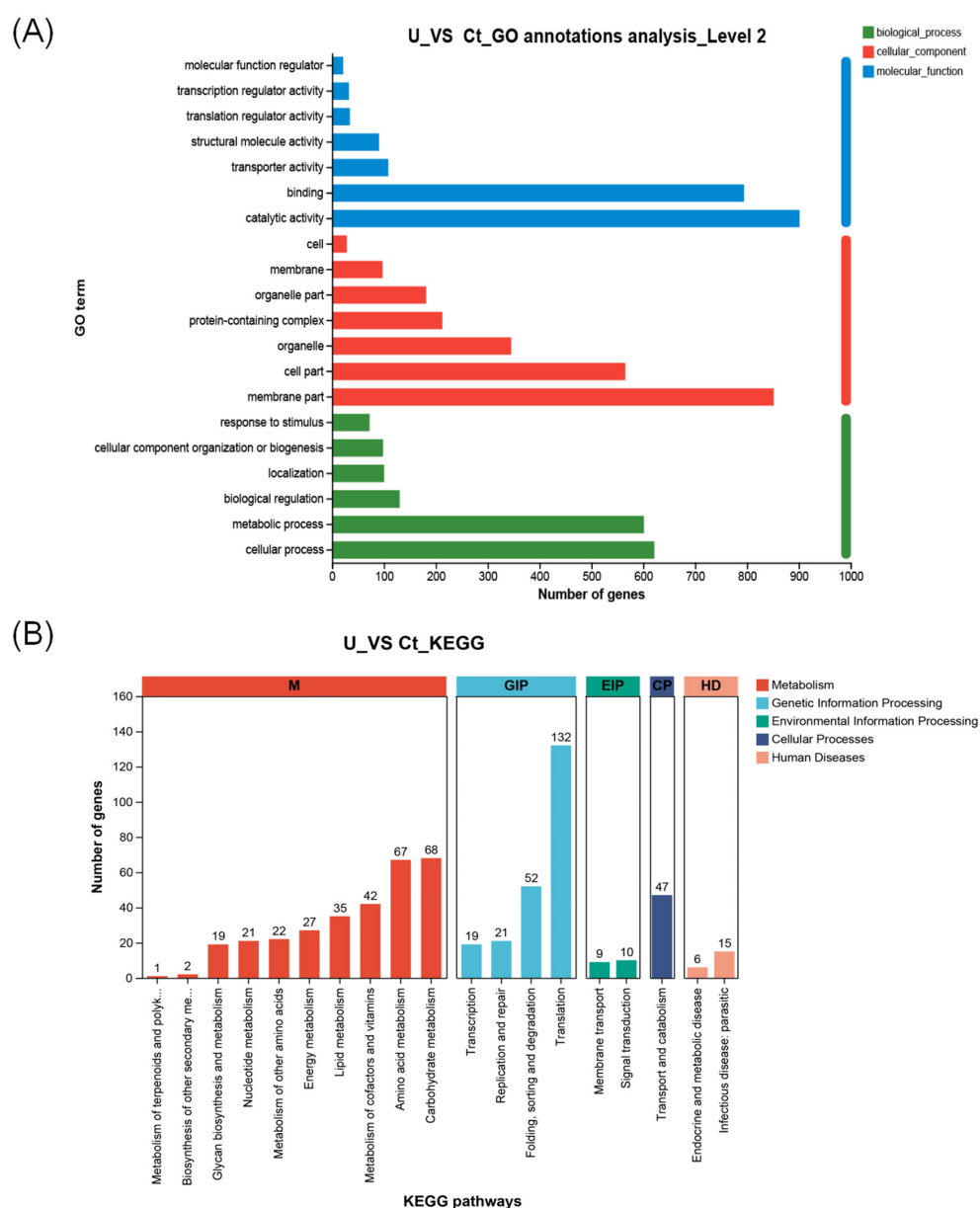
Figure 4. Functional enrichments and classifications of differentially expressed genes in N. oceanica . (A) The N. oceanica genes were systematically categorized into biological process (BP), cellular component (CC), and molecular function (MF) subclasses through Gene Ontology (GO) analysis. The distribution of genes in each class was visualized using a histogram. (B) Additionally, a pathway enrichment analysis of DEGs was conducted using the KEGG.
