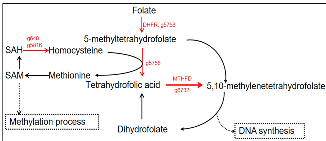
Figure 7. Differential expression analysis of genes related to folate metabolism affected by urea addition in N. oceanica . The folate metabolism pathway was briefly constructed. The “red arrows” represent the upregulation of the urea addition condition.
