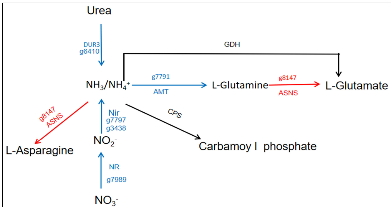
Figure 5. Nitrogen metabolism-related genes differential expression analysis in N. oceanica under urea addition conditions. Brief construction of the nitrogen assimilation pathway and transcriptional level changes in key genes marked with arrows. The different colored arrows represent the transcriptional changes in the gene, the “red arrows” and the “blue arrows” represent the upregulation and downregulation of the urea addition condition, respectively.
