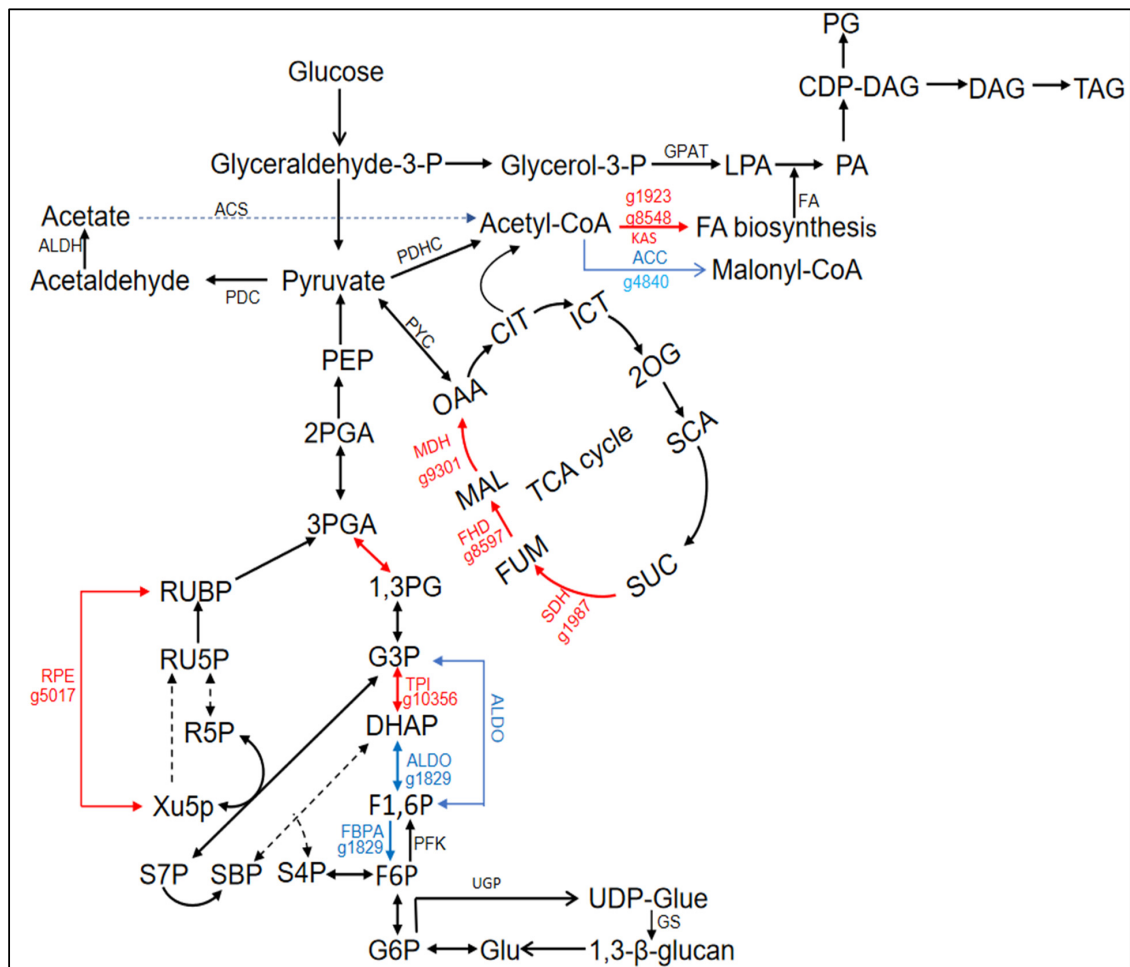
Figure 6. Differential expression analysis of genes related to lipid metabolism and carbon metabolism in N. oceanica under urea addition. The carbon metabolism pathway and lipid metabolism pathway were briefly constructed. The different colored arrows represent the transcriptional changes in the gene, the “red arrows” and the “blue arrows” represent the upregulation and downregulation under Ct vs. U, respectively.
