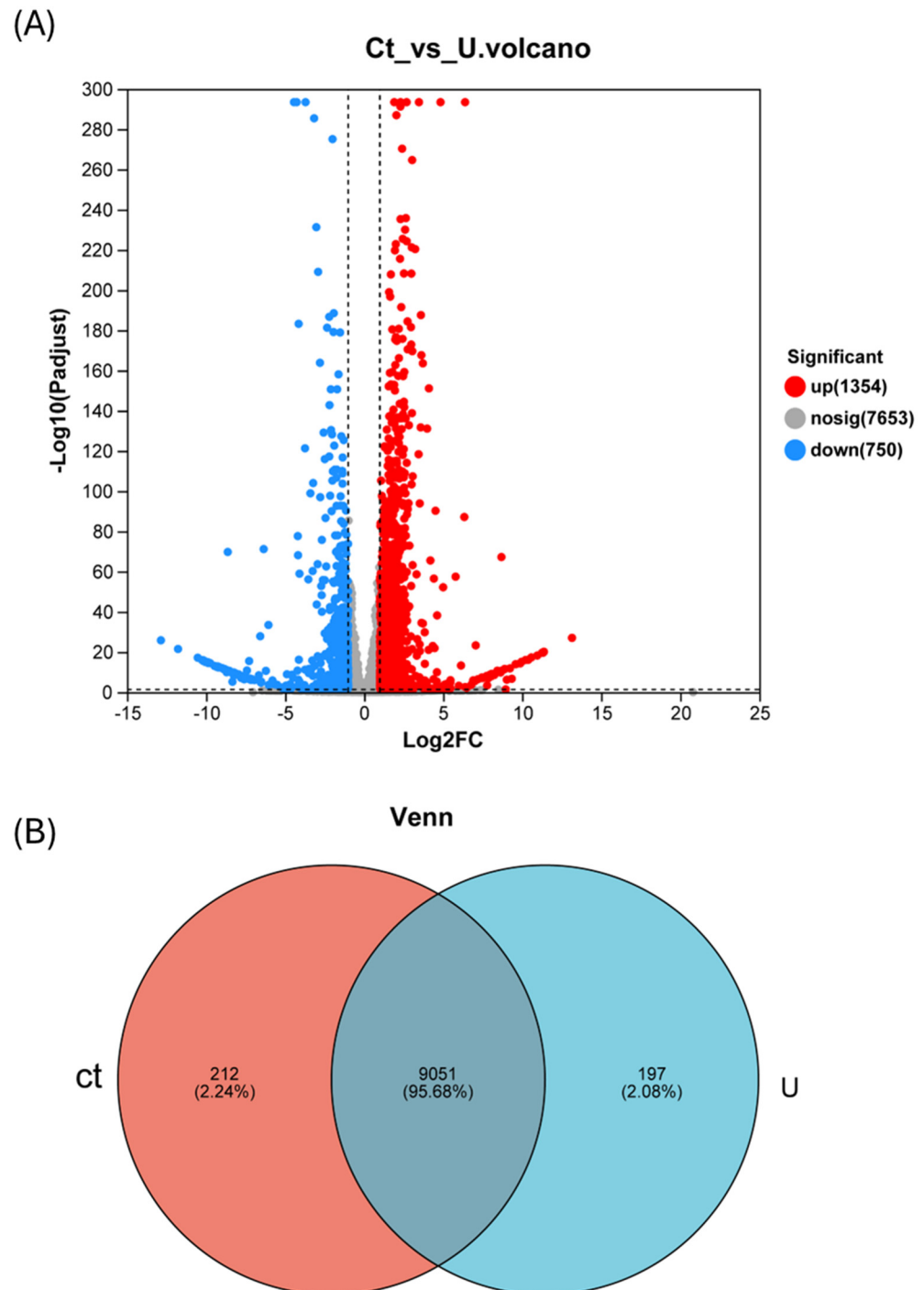
Figure 3. Venn diagram between samples and analysis of differentially expressed genes. (A) Volcano plot illustrating the differential expression pattern of genes between Ct and U conditions. Red dots, blue dots, and gray dots represent upregulated DEGs, downregulated DEGs, and genes with no significant change (Ct), respectively. (B) The red portion represents unique genes from the group without urea addition, the blue portion represents unique genes from the group with urea addition and the region at the intersection of the two parts represents shared genes. Quantification of differentially expressed genes in N. oceanica under U ( \text{NaNO}_3 + urea) and Ct ( \text{NaNO}_3 ) cultivation conditions (at least a 2-fold change under urea addition).
