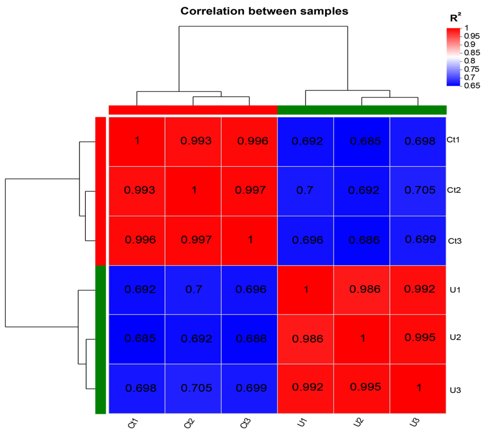
Figure 2. Primary analysis of mRNA-seq data in N. oceanica . Sample correlation analysis heatmap. Note: Red indicates strong correlation, and blue indicates weak correlation.
