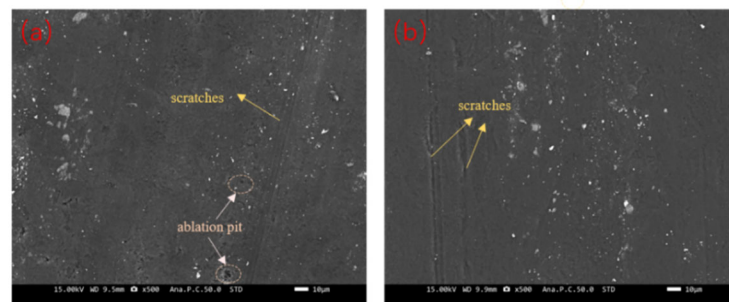
Figure 13. SEM morphology of carbon brush worn on different samples. (a) Collector ring original sample, (b) Cu-GNS composite coating.
