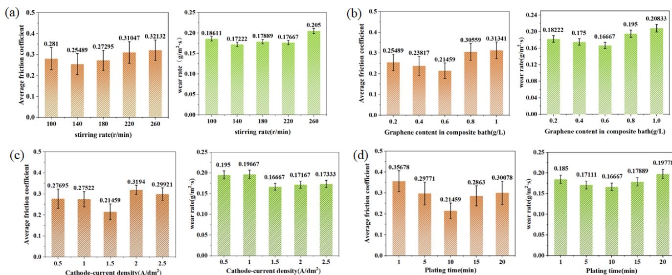
Figure 11. Friction and wear characteristics under different composite electroplating parameters: (a) stirring speed, (b) graphene content, (c) electroplating current density, (d) plating time.
