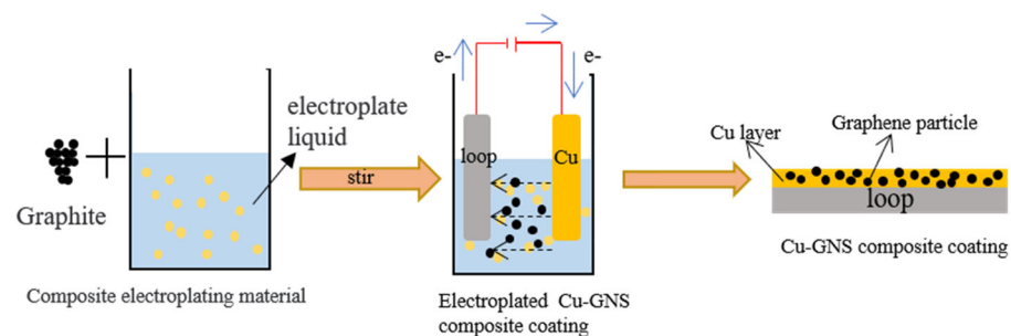
Figure 1. Cu–GNS composite coating process.
