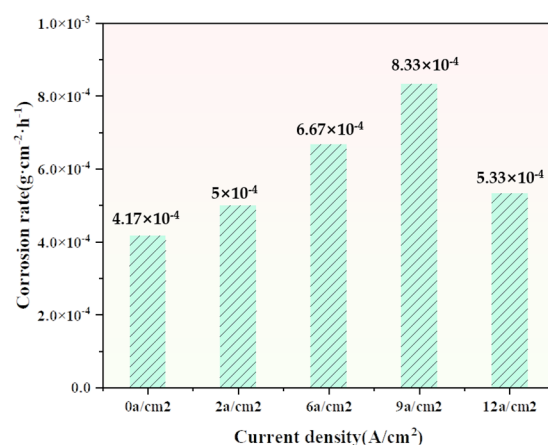
Figure 18. Corrosion rate of collector ring under different current densities at 1 N pressure.
