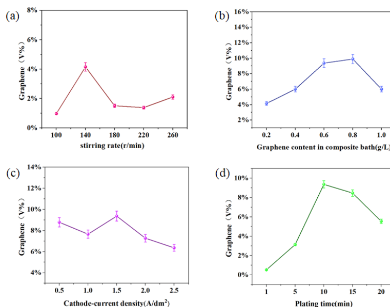
Figure 5. Graphene deposition rates of Cu–GNS composite coatings under different composite plating parameters. (a) Stirring speed, (b) graphene content, (c) electroplating current density, (d) plating time.
