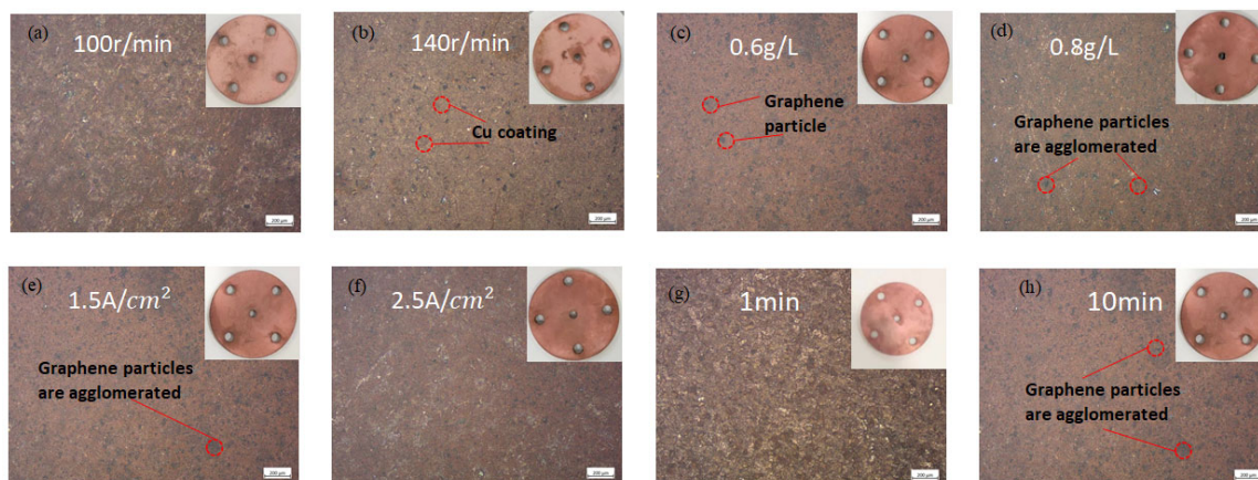
Figure 4. Optical microscope morphology and macroscopic picture of Cu–GNS composite coating with changing. (a,b) Stirring speed 100 r/min and 140 r/min. (c,d) Graphene content 0.6 g/L and 0.8 g/L. (e,f) Electroplating current density 1.5 A/cm 2 and 2.5 A/cm 2 . (g,h) Electroplating time 1 min and 10 min.
