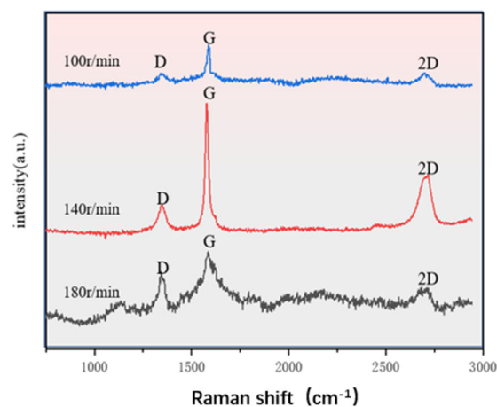
Figure 9. Raman spectra of Cu–GNS composite coatings prepared at different stirring speeds.
