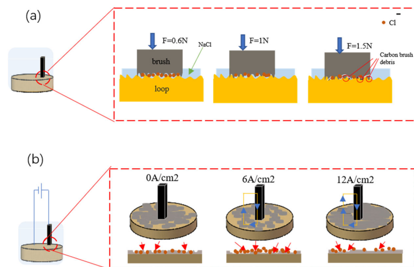
Figure 20. Influence mechanism of corrosion resistance of collector ring. (a) Research on the corrosion resistance of collector rings by pressure. (b) Research on the corrosion resistance of collector rings by current density.
