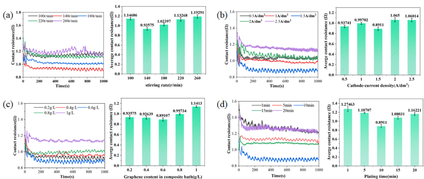
Figure 10. Contact resistance characteristics under different composite electroplating parameters: (a) stirring speed, (b) electroplating current density, (c) graphene content, (d) plating time.
