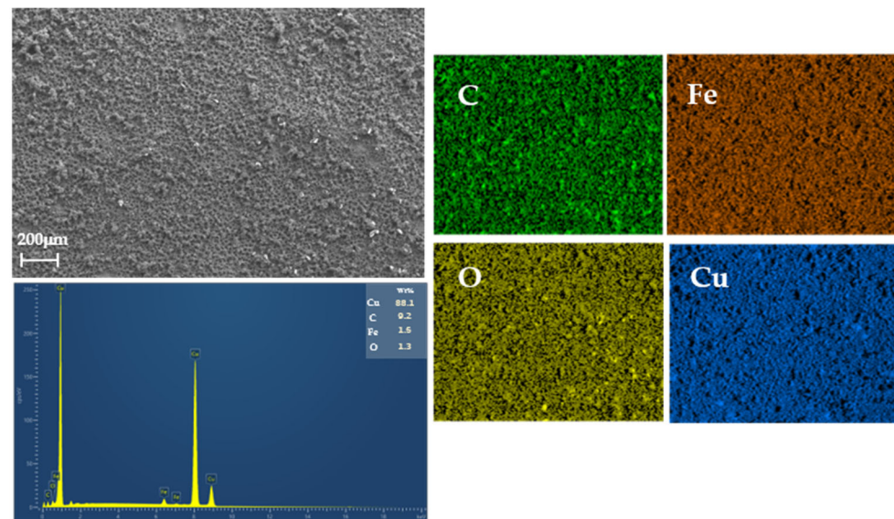
Figure 8. Surface morphology of composite layer under optimum plating parameters.
