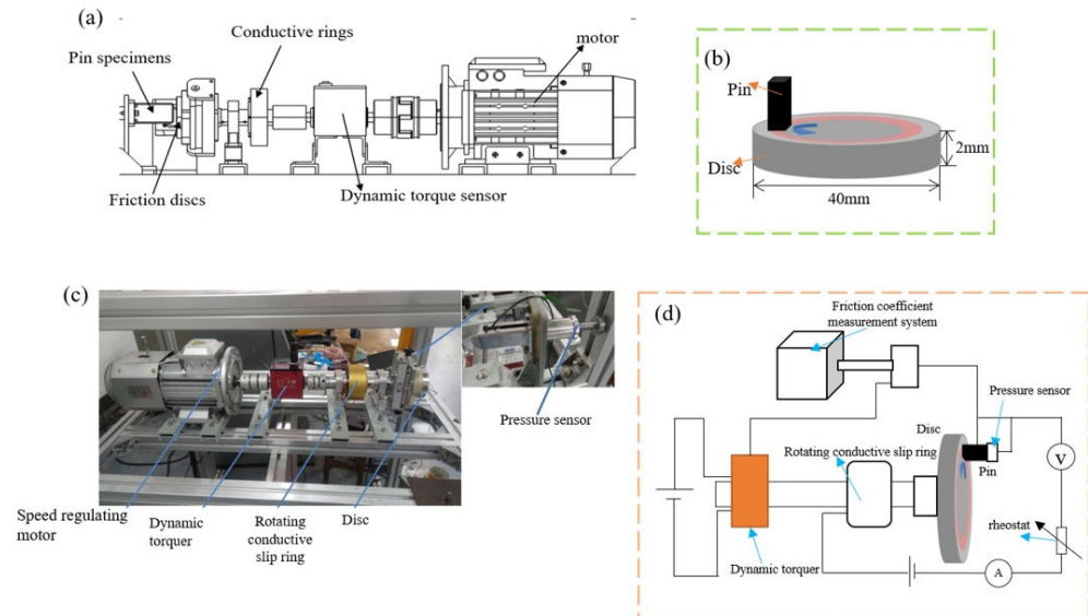
Figure 2. (a) Current-carrying friction and wear testing machine. (b) The test mode is pin–disk contact. (c) Physical diagram of current-carrying friction and wear testing machine. (d) Schematic diagram of the test device.
