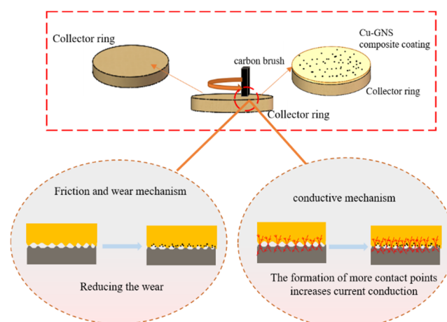
Figure 14. Schematic diagram of current-carrying tribological mechanism of Cu/graphene composite coating.
