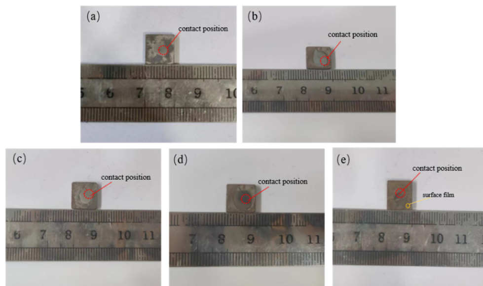
Figure 17. Macroscopic diagram after corrosion with different current densities under 1 N pressure. (a) 0 A/cm 2 , (b) 2 A/cm 2 , (c) 6 A/cm 2 , (d) 9 A/cm 2 , (e) 12 A/cm 2 .
