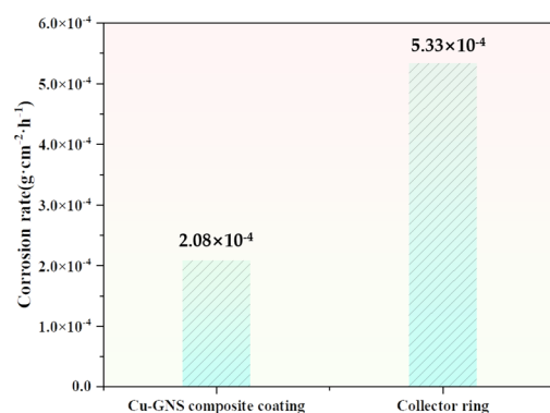
Figure 19. Corrosion rate of collector ring and Cu–GNS composite coating at 1 N pressure 12 A/cm 2 .
