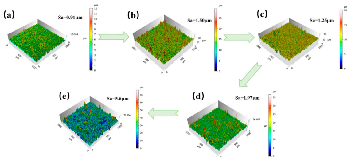
Figure 6. Three-dimensional profiles of Cu–GNS composite coatings prepared at different plating times: (a) 1 min, (b) 5 min, (c) 10 min, (d) 15 min, (e) 20 min.
