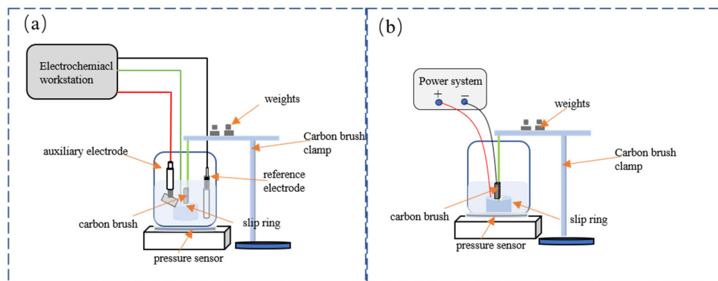
Figure 3. (a) Electrochemical corrosion workstation. (b) Simulated actual corrosion device.
