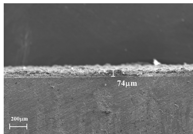
Figure 7. Cross-sectional morphology of composite plating layer under optimal plating parameters.
