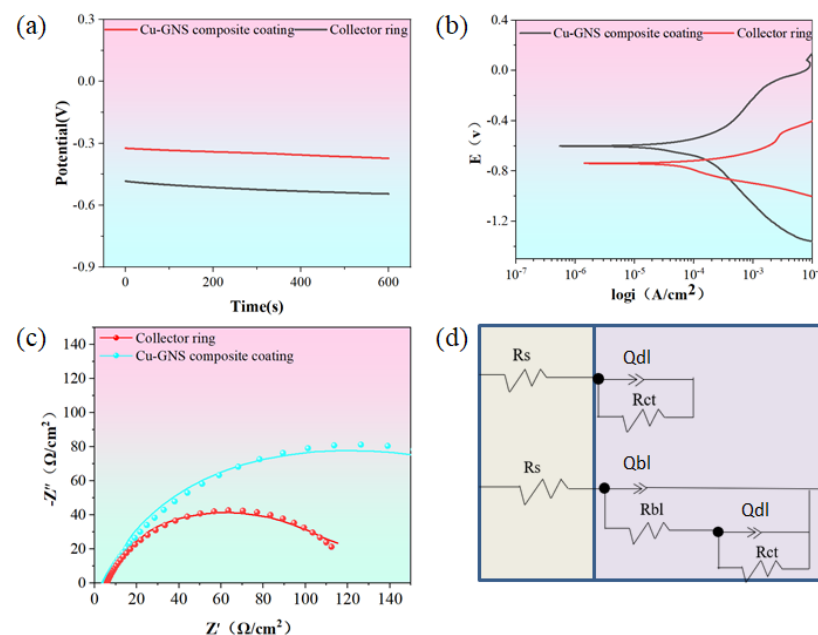
Figure 16. Study on electrochemical corrosion resistance of collector ring and Cu–GNS composite coating under 1 N pressure. (a) Open circuit potential, (b) polarization curve, (c) Nyquist plot, (d) equivalent circuit diagram of EIS spectrum.
