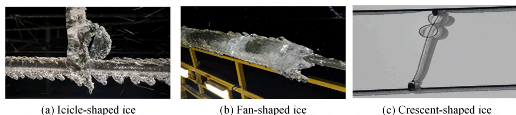
Figure 4. Icing morphology of the overhead contact line.
