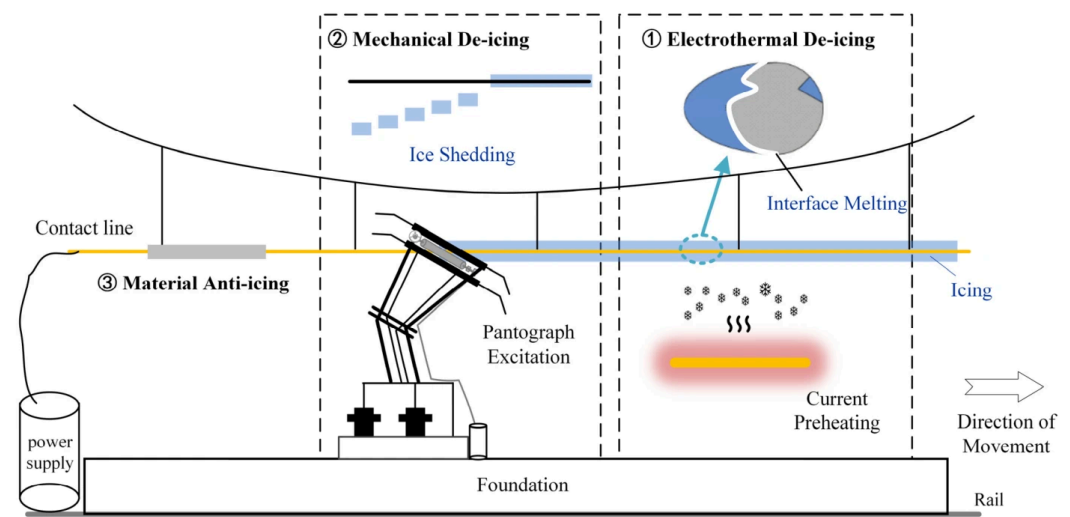
Figure 11. Coupled de-icing design diagram.
