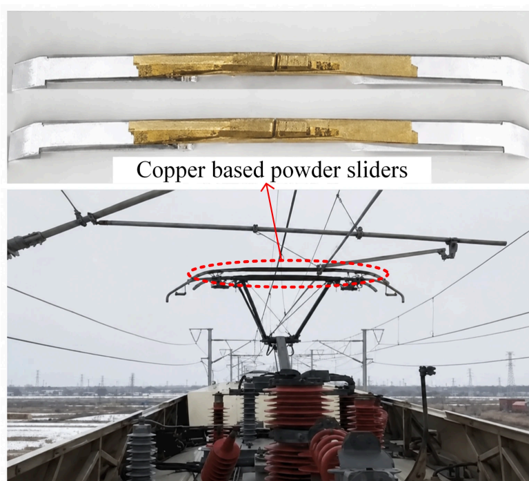
Figure 6. Hot-sliding de-icing method.
