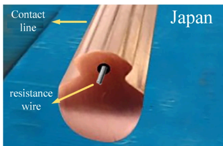
Figure 9. Japanese built-in resistance wire de-icing.
