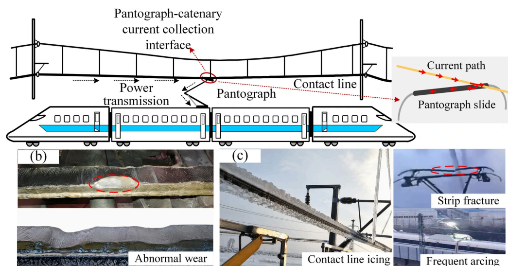
Figure 1. (a) High-speed railway PCSs; (b) abnormal wear in humid/rainy environments; (c) damage in icing environment.
