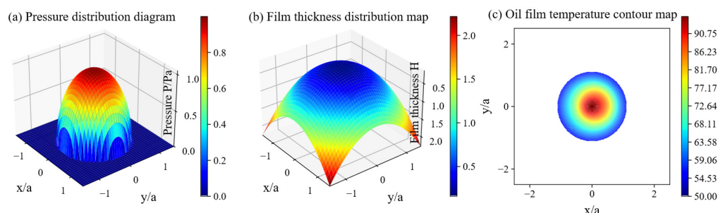
Figure 3. Numerical results of the point-contact TEHL model.
