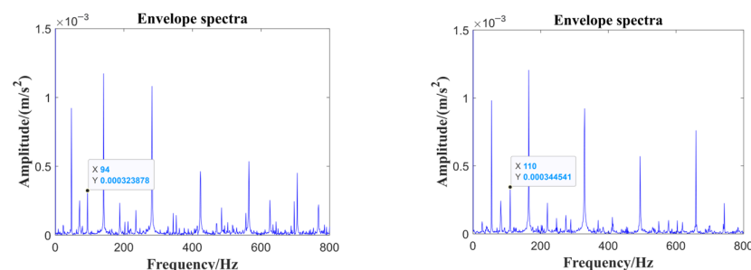
Figure 13. Signal envelope spectra for 1500 rpm and 1750 rpm outer-ring fault experiments with a 0.6 mm spall.
