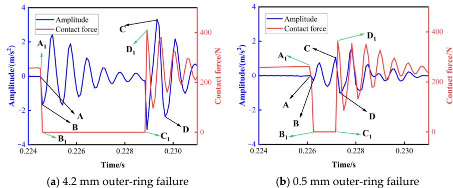
Figure 8. Localized enlargement of rolling-bearing outer-ring fault signals.
