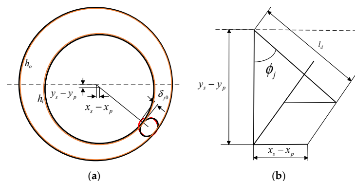
Figure 5. Contact deformation and radial displacement relationship of the rolling element–raceway contact under TEHL conditions: (a) Hertzian contact deformation of the rolling element; (b) geometric relationship of radial displacement, where the orange region denotes the lubricating oil film.
