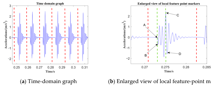
Figure 10. Simulated time-domain response plot at 1500 rpm for a 2 mm outer ring, with the local feature-point markers zoomed in.
