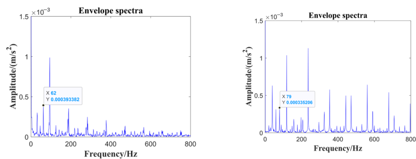
Figure 12. Experimental signals and envelope spectra for 1000 rpm and 1250 rpm outer-ring faults with a 0.6 mm spall.
