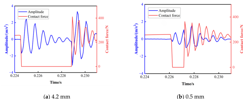
Figure 7. Simulated signals versus Hertzian contact force variation for rolling-bearing defects of different sizes.
