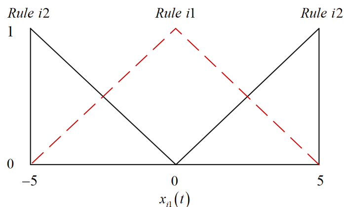
Figure 1. Membership function for Example 1.
