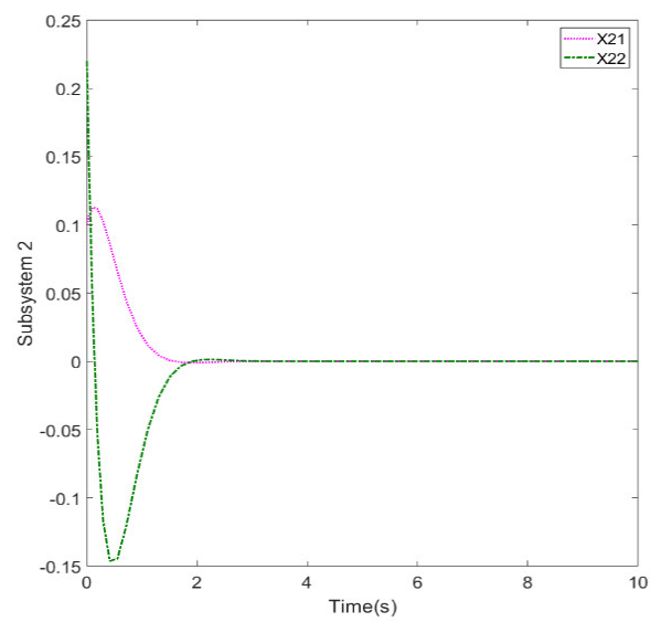
Figure 6. The state responses correspond to subsystem 2 in Example 2.
