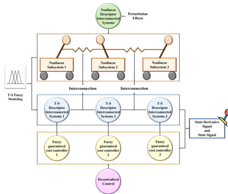
Figure 4. The proposed control method for a nonlinear TIP system.
