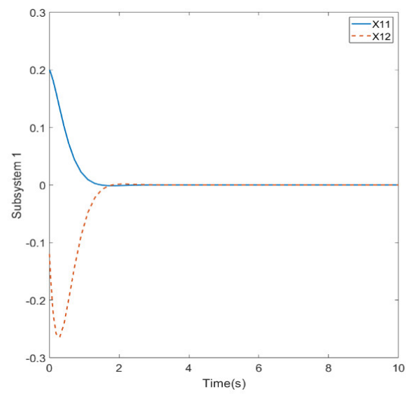
Figure 5. The state responses correspond to subsystem 1 in Example 2.
