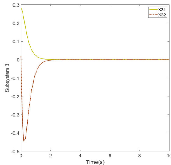
Figure 7. The state responses correspond to subsystem 3 in Example 2.
