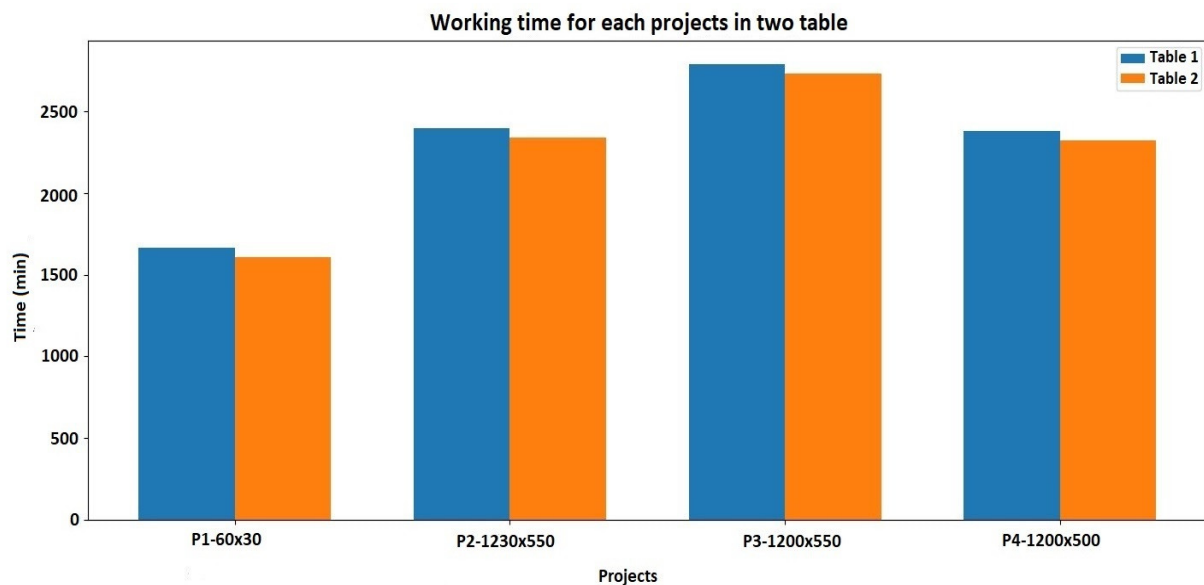
Figure 19. Time optimization after changing the position of the tools in the magazine.
