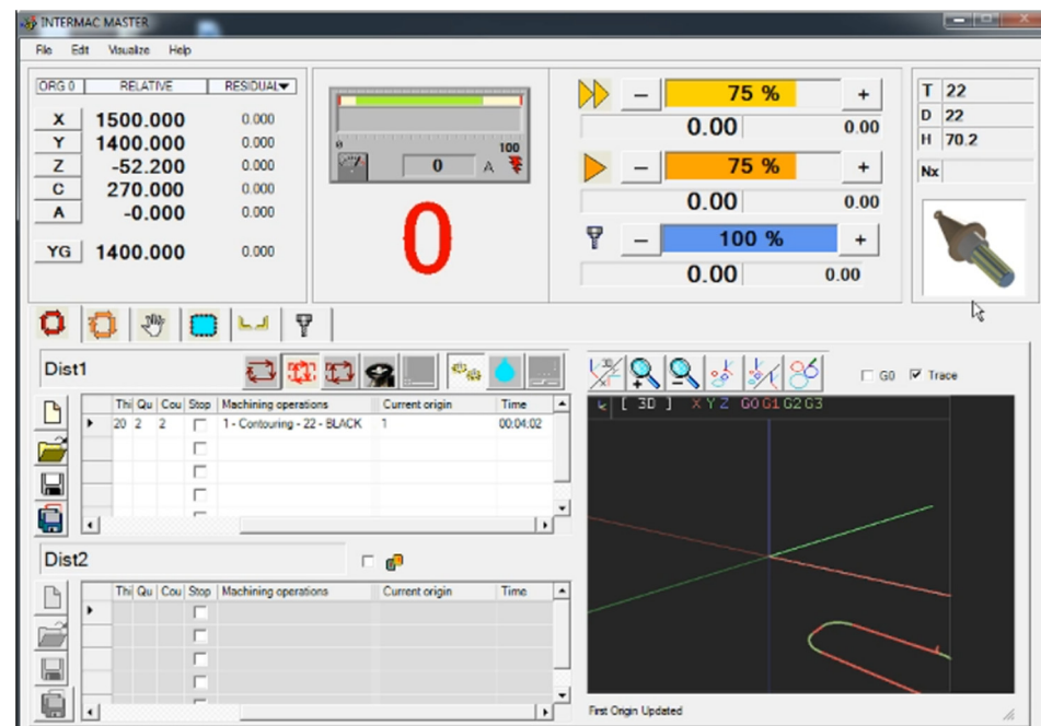
Figure 12. Tool name T22 or end milling.
