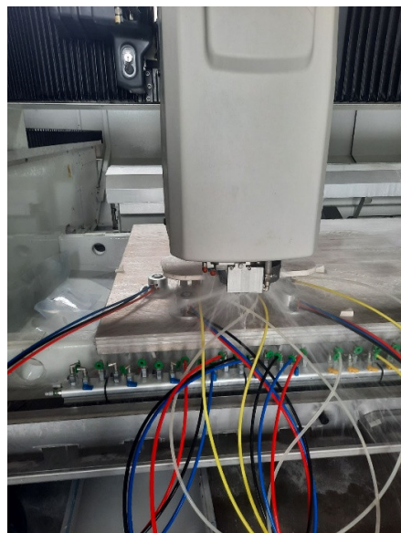
Figure 8. Working process of the CNC machine.
