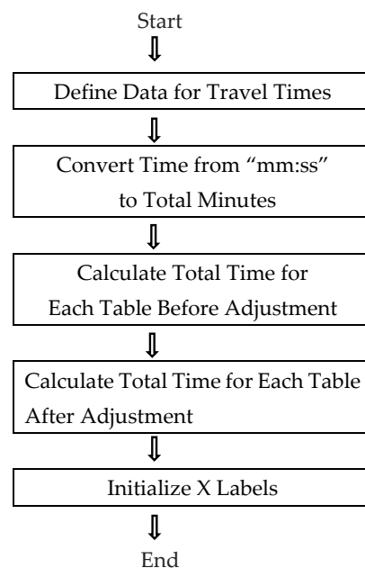
Figure 17. Flow chart for data analysis using the Python programming language-tool of travel time.
