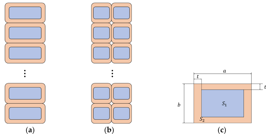
Figure 3. Armature coil winding configurations: (a) single-layer, (b) double-layer. (c) Schematic diagram of the armature coil cross-section.
