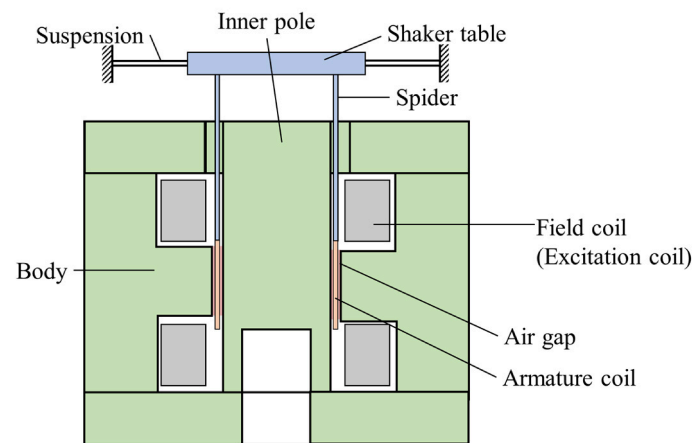
Figure 2. Schematic diagram of the electrodynamic vibrator structure.
