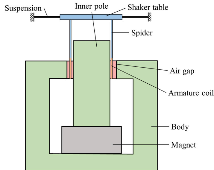
Figure 1. Main structure of electrodynamic vibrator.
