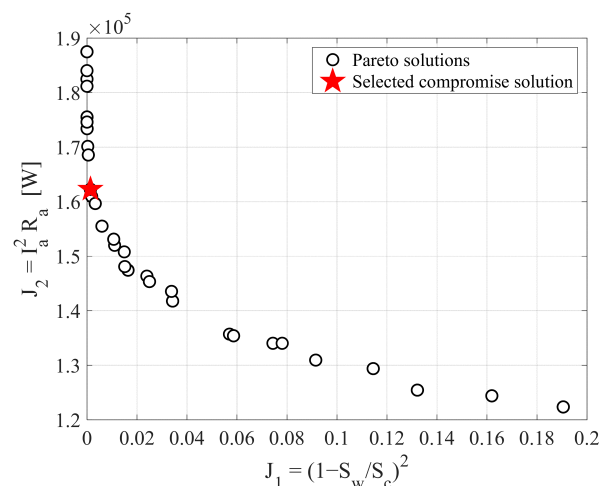
Figure 6. Pareto solutions of armature coil optimization.
