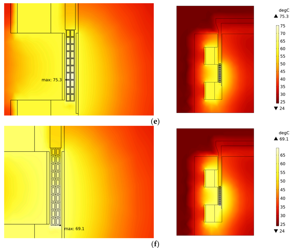
Figure 8. Temperature field inside electrodynamic vibrator for different parameter cases: (a) Case 1, (b) Case 2, (c) Case 3, (d) Case 4, (e) Case 5 and (f) Case 6.
