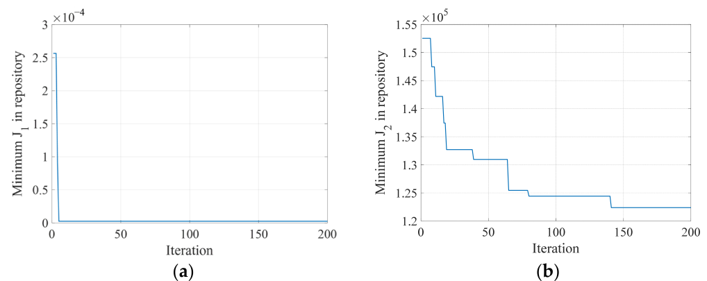
Figure 7. Convergence history curve of (a) J_1 (b) J_2 .
