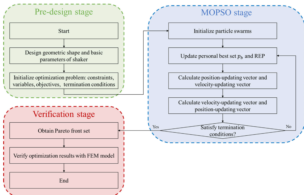
Figure 5. Design optimization procedure of electrodynamic vibrator.
