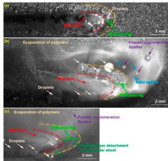
Figure 5. Defects during melting of AlSi10Mg (a) Initial melt-pool formation, with droplet ejection and visible melt-pool lag during laser interaction with the powder sheet, (b) Polymer evaporation intensifies plume formation, promoting powder agglomeration, solid spatter, droplet ejection and melt-pool instability, (c) Powder-layer detachment occurs as melt-pool lag, droplets and agglomerated spatter indicate unstable mass transfer during melting [33].
