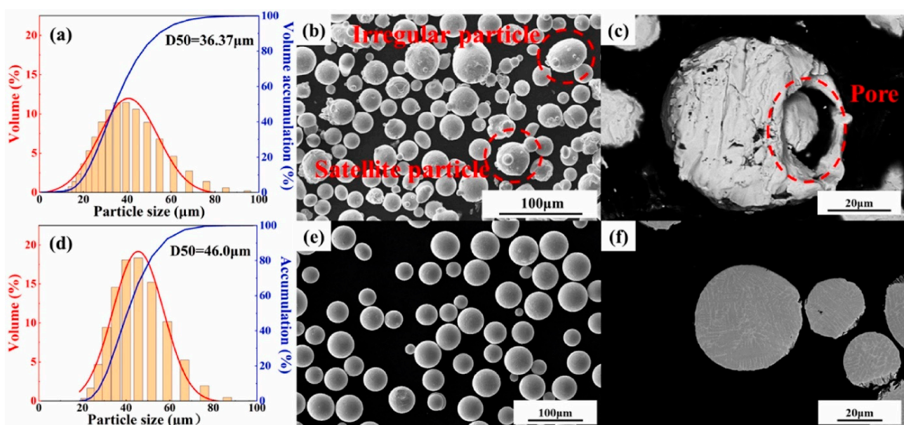
Figure 7. Comparison of particle size distribution (a,d), powder morphology (b,e) and powder cross section (c,f) of GA powder (a–c) and PREP powder (d–f) [53].
