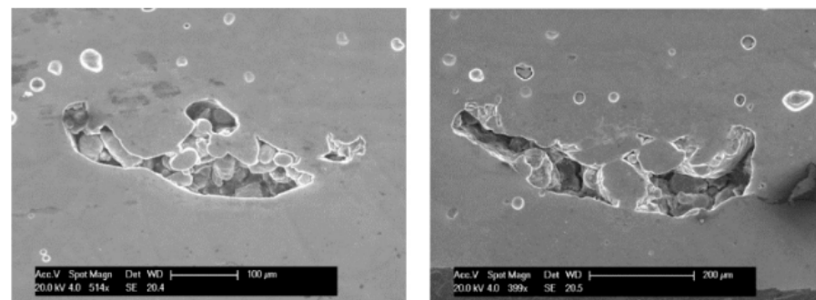
Figure 2. Keyhole pore enclosing non-molten powders [1].
