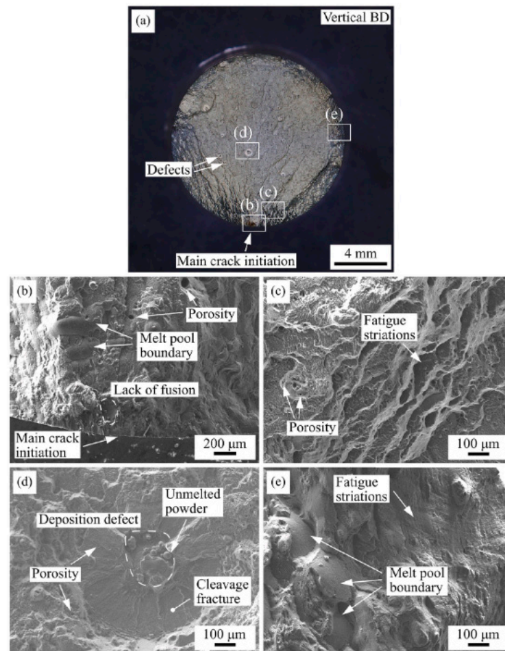
Figure 4. The fracture surface of the vertically built specimen from the performed LCF test with \epsilon_a = 6 \times 10^{-3} . An overview of the entire fracture surface is shown in (a), with a detailed view of the main crack-initiation site presented in (b). The transgranular crack propagation is depicted in (c). The fracture morphology around a deposition defect resulting from the deposition strategy is observed in (d), while cracking along the boundaries of melt pools is documented in (e) [31].
