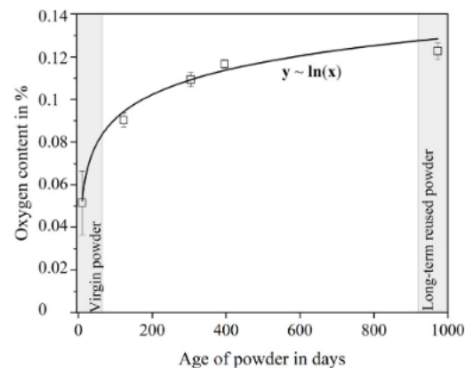
Figure 3. Oxygen content depends on powder age, beginning with virgin and ending with long-term reused powder [21].
