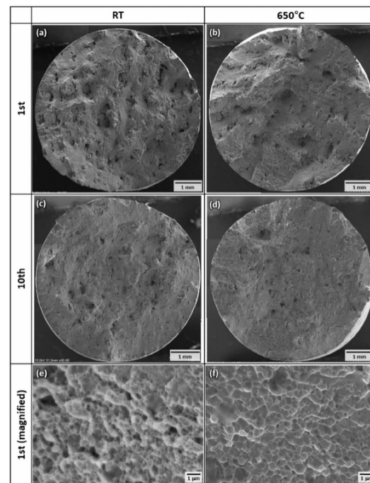
Figure 6. SEM fractographs of the (a,b,e,f) 1st and (c,d) 10th specimens after tensile tests at (a,c,e) 25 and (b,d,f) 650 °C showing voids originating from defects formed during the SLM process. (e,f) are magnified fractographs of (a,b), showing coarser ductile dimples at 650 °C [51].
