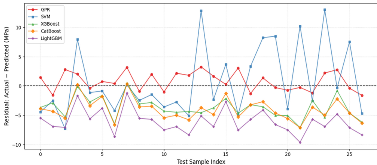
Figure 8. Residual distribution for the blocked-holdout test data set (Actual—Predicted, MPa).
