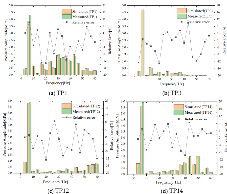
Figure 16. Frequency vs. amplitude of pressure pulsation at four cylinders.
