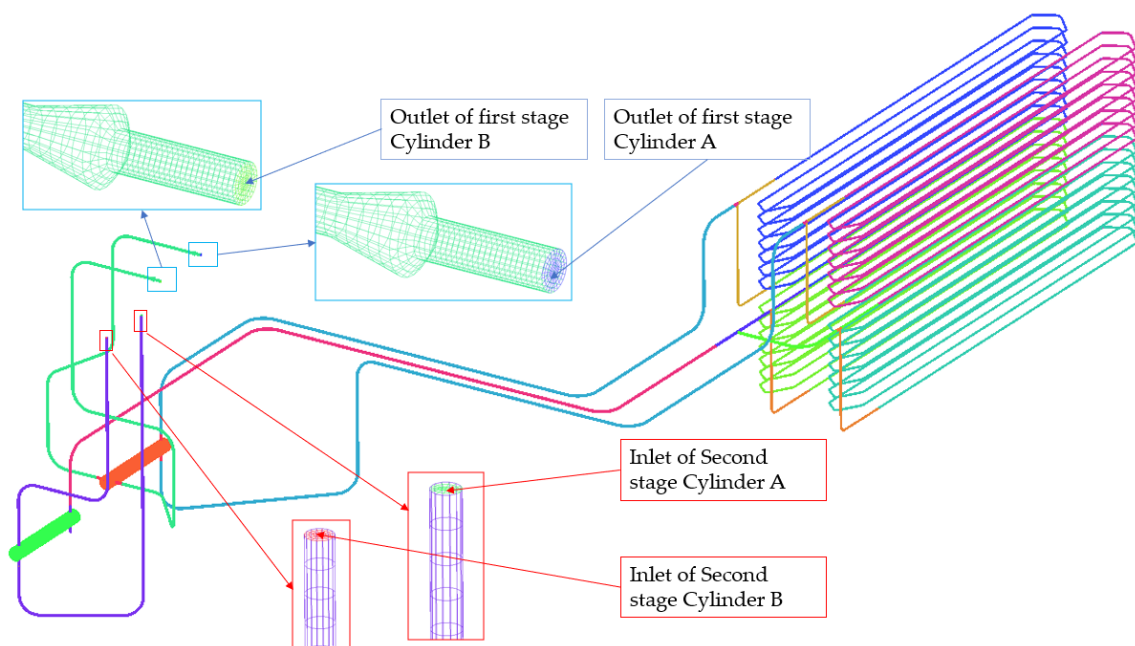
Figure 6. Discrete model of the interstage pipeline.
