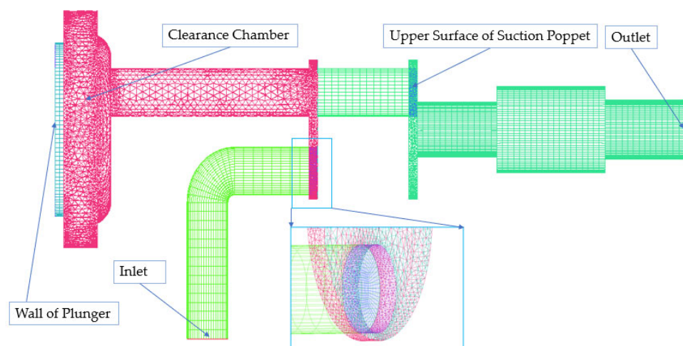
Figure 4. Discrete model for the combined valve and clearance chamber.
