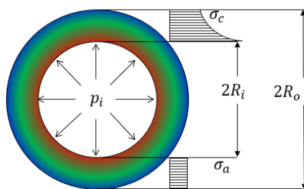
Figure 10. The circumferential and axial stress induced by internal pressure.
