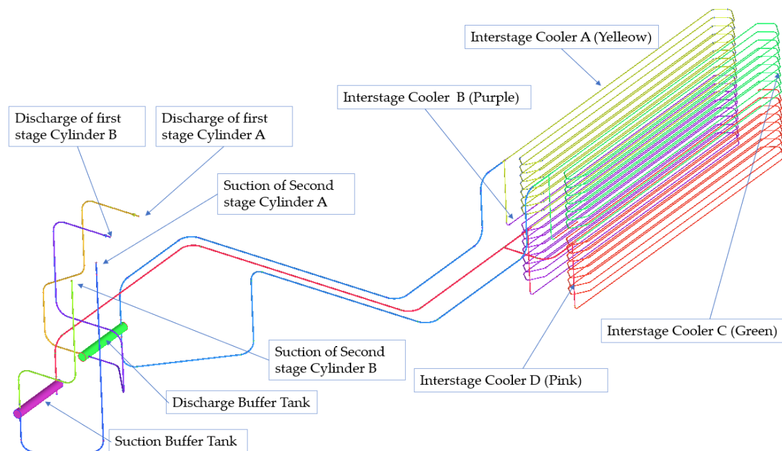
Figure 5. Physical model of the interstage pipeline.
