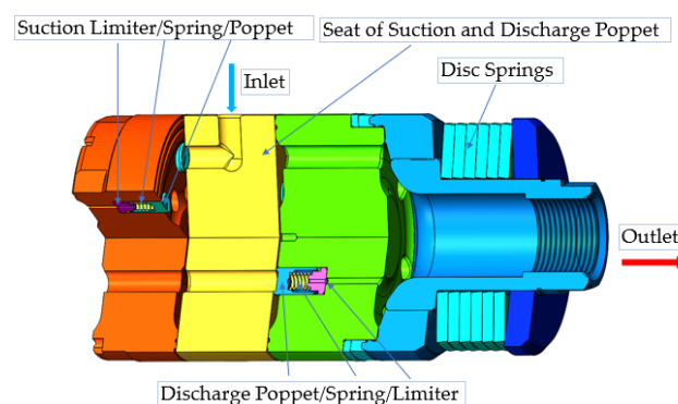
Figure 1. Solid model of the multi-poppet valve.
