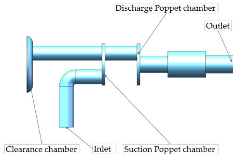
Figure 3. Simplified flow domain of the combined valve in the first stage.
