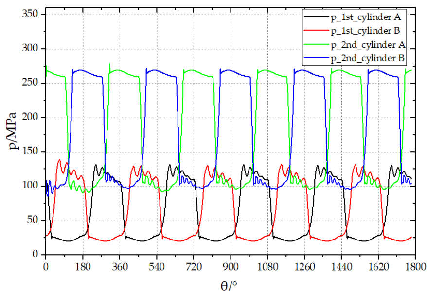
Figure 9. Pressure inside the first and second stages of the cylinders.
