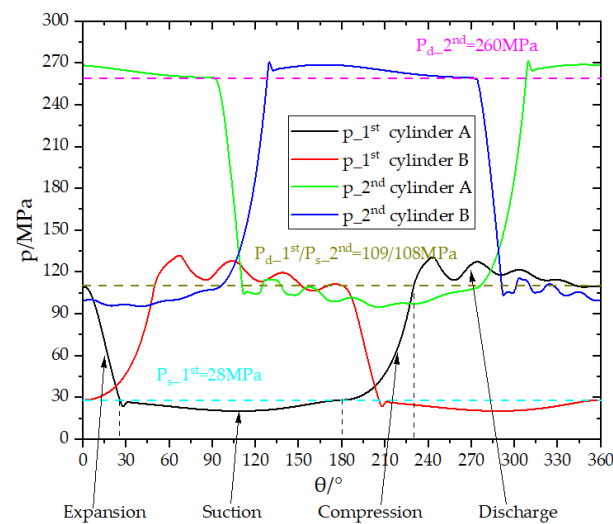
Figure 13. p – \theta diagrams inside the four cylinders.
