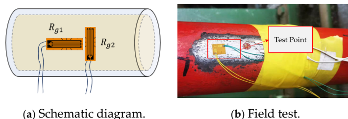
Figure 11. Arrangement of the strain gauges.
