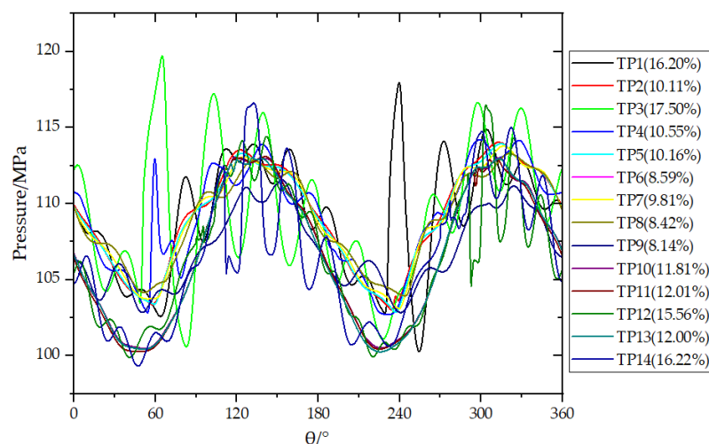
Figure 15. Pressure pulsation of the 14 monitored points inside the interstage pipeline.
