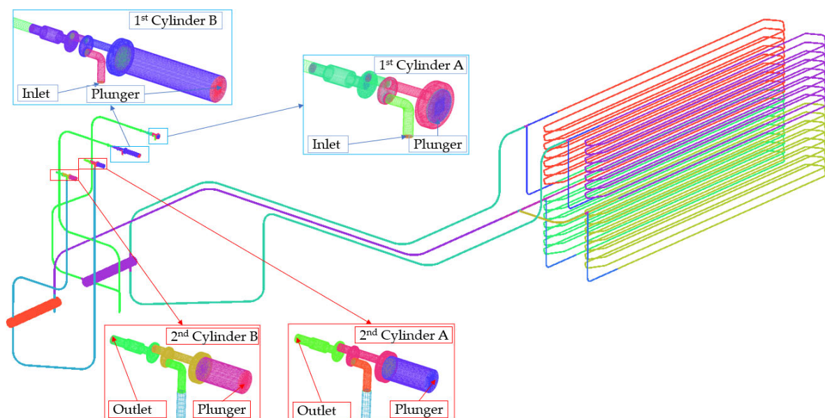
Figure 7. The entire CFD model of the interstage pipeline.
