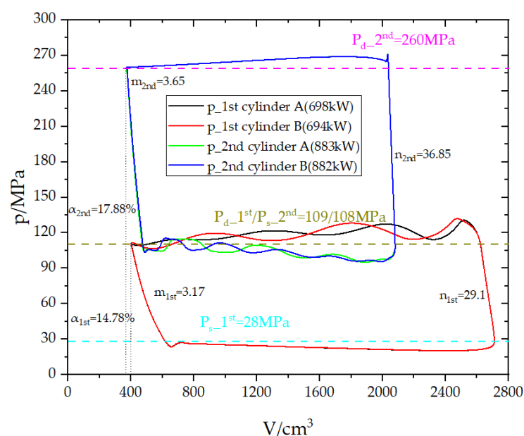
Figure 14. p–V diagrams inside the four cylinders.
