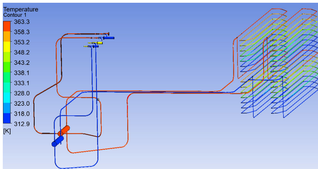
Figure 8. Steady temperature distribution of the interstage pipeline.
