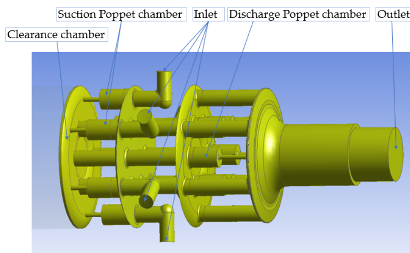
Figure 2. Flow domain of the combined valve in the first stage.
