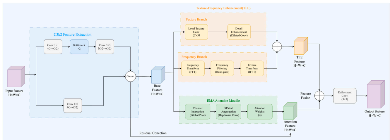
Figure 2. Structural Diagram of the C3k2-TFE-EMA Module.
