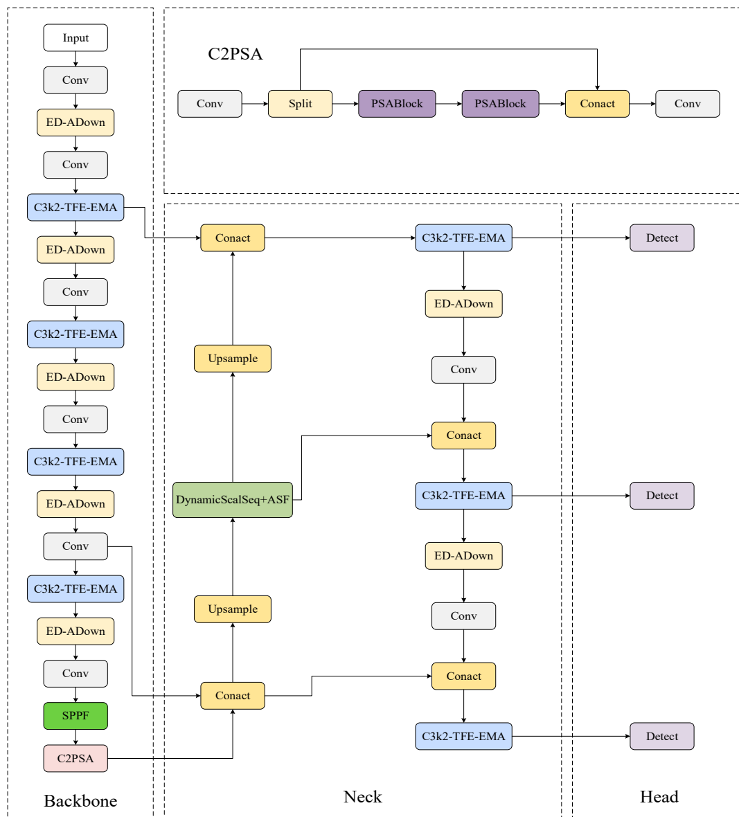
Figure 1. TAD-YOLO11n Network Architecture.
