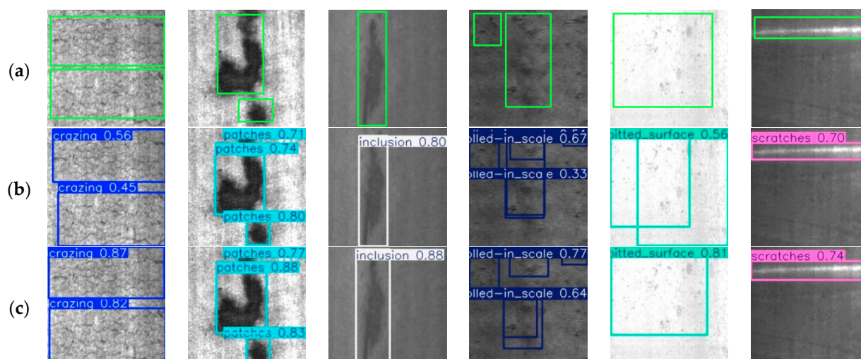
Figure 7. Detection results for six types of defects. (a) Ground truth. (b) YOLO11n. (c) TAD-YOLO.
