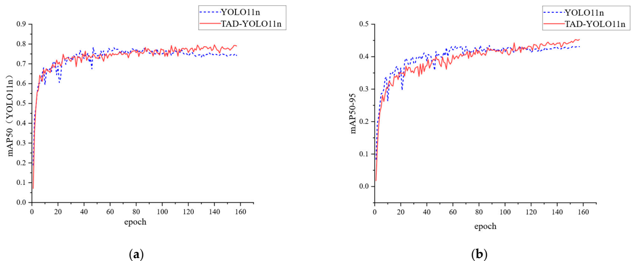
Figure 9. Training convergence curves of YOLO11n and TAD-YOLO11n. (a) mAP50. (b) mAP50–95.
