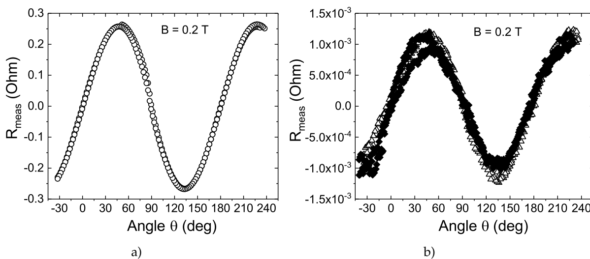
Figure S3. Measured resistance signal vs. angle \theta between the applied field and the c-axis of the graphite samples with thicknesses: (a) 30.6 \mu\text{m} ( \circ ), (b) 6.9 \mu\text{m} ( \triangle ), and 1.2 \mu\text{m} ( \blacklozenge ).
