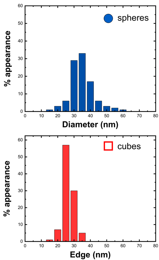
Figure S1. Size distribution of the diameter for spherical core-shell nanoparticles and the edge dimension for the cubic ones.
