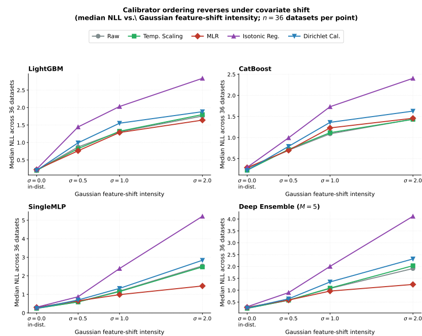
Figure 5. Calibrator ordering reverses under covariate shift. Each panel shows median NLL across the 36 datasets as Gaussian feature-shift intensity \sigma increases from 0 (in-distribution, leftmost) to 2 (heavy shift, rightmost). Five lines per panel correspond to the five calibration methods. The in-distribution point ( \sigma = 0 ) is the per-dataset median across five seeds, and shifted points are at a single seed across the same 36 datasets.
