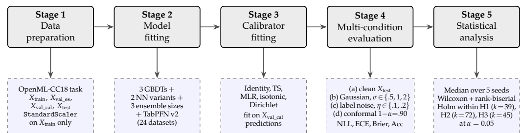
Figure 1. Schematic of the five-stage experimental pipeline. The top row shows the sequential workflow, and the bottom row summarises the principal inputs, configurations, and outputs associated with each stage.
