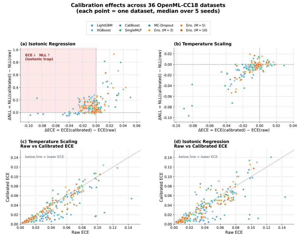
Figure 4. Four-panel diagnostic of calibration effects across 36 OpenML-CC18 datasets (each point = one dataset, median over 5 seeds, with dots coloured by model class). (a) \Delta\text{NLL} vs. \Delta\text{ECE} under isotonic regression. The shaded upper-left quadrant marks the “isotonic trap”. (b) The same for temperature scaling: both metrics move together, near the origin. (c) Raw vs. calibrated ECE under temperature scaling. (d) The same for isotonic regression.
