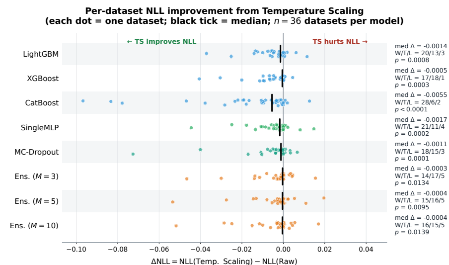
Figure 3. Per-dataset NLL improvement from temperature scaling. Each dot is one dataset (median over 5 seeds). The black tick is the median across datasets, and the annotation panel on the right reports the median \Delta , W/T/L counts, and uncorrected Wilcoxon p .
