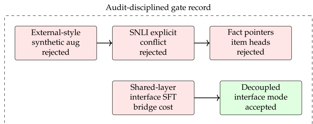
Figure 5. Negative-result map. Plausible additions were tested and rejected when they harmed the targeted slice or damaged the bridge.
