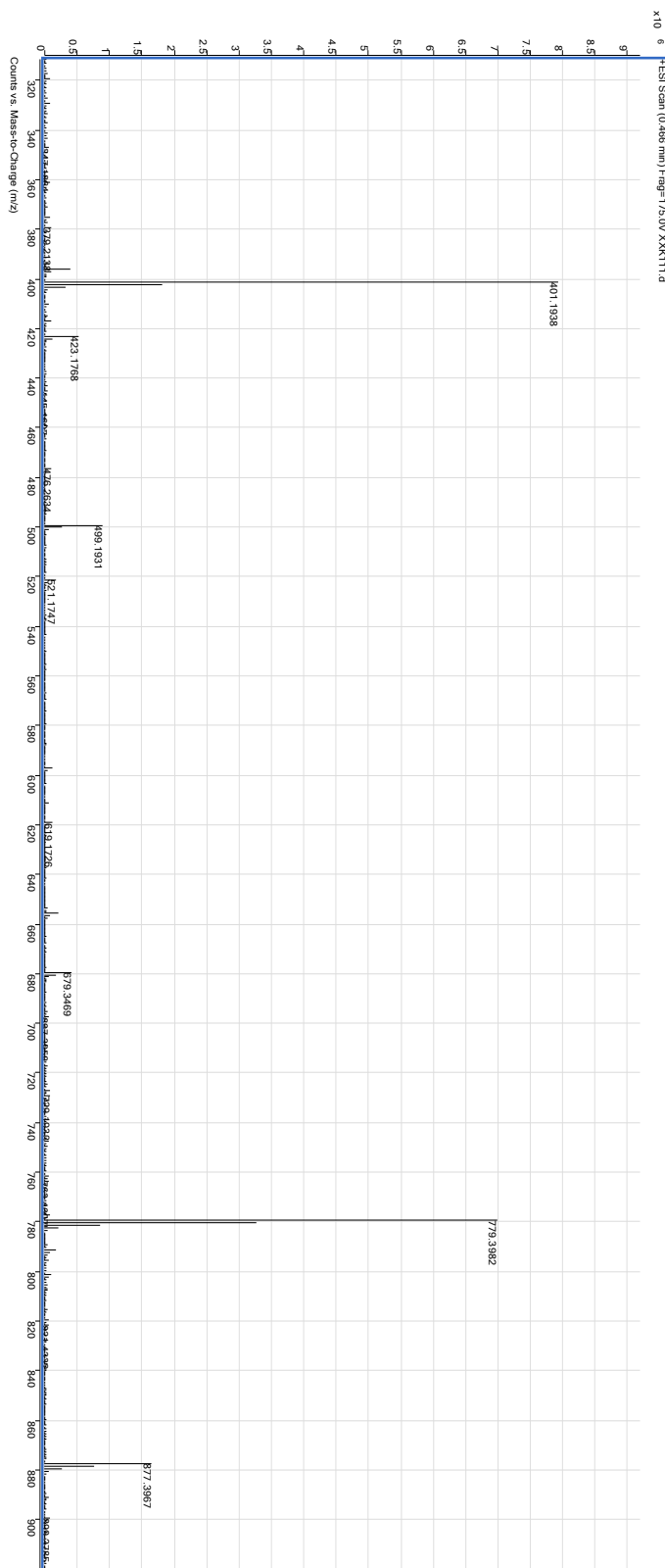
Figure S7. HR-ESI-TOF-MS spectrum of compound 1.
