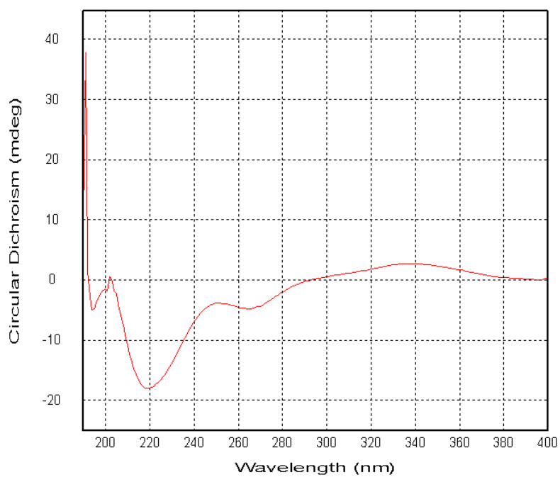
Figure S6. CD spectrum of compound 1 recorded in MeOH at ambient temperature.
