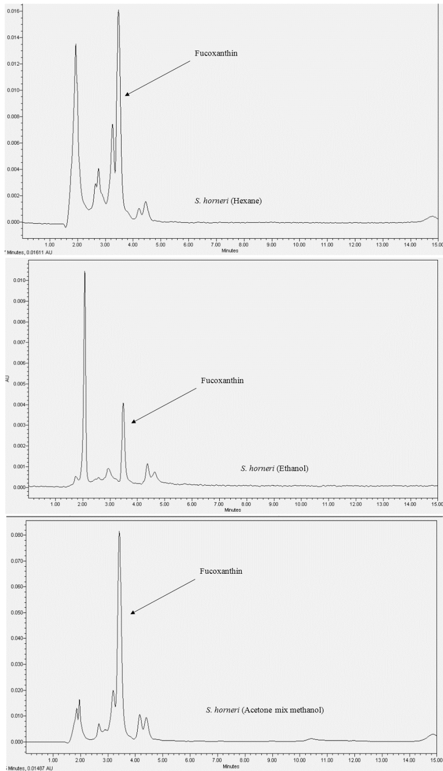
Figure S1. HPLC chromatogram of fucoxanthin content in (a) S. japonica using various solvent extraction and (b) S. horneri using various solvent extraction.
