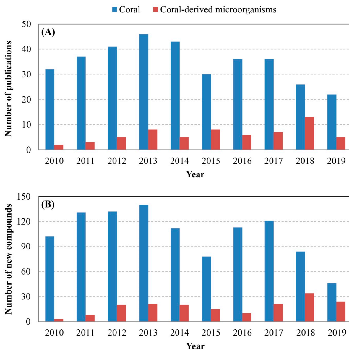
Figure 31. Number of PubMed publications describing natural products from coral and coral-derived microorganisms (A); number of new compounds produced by coral and coral-derived microorganisms (B) covering 2010–March 2019.
