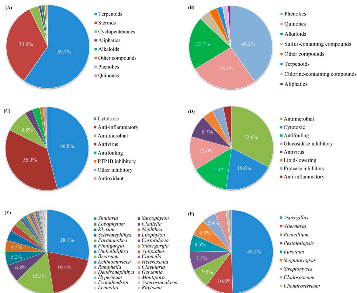
Figure 32. Distribution of the bioactive compounds according to chemical structure for coral (A) and coral-derived microorganisms (B); according to activity type in coral (C) and coral-derived microorganisms (D); according to genera of coral (E) and coral-derived microorganisms (F).
