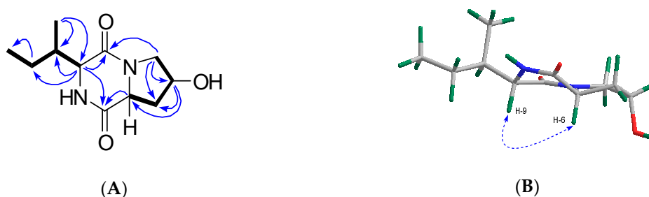
Figure 4. Key COSY (bold) and HMBC correlations H→C (arrows) (A) and key NOESY correlations (dashed line, B) observed for compound 8 .
