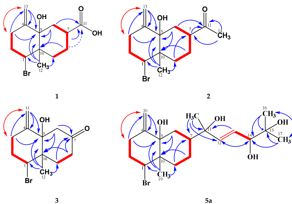
Figure 2. H,H COSY ( ^3J —, ^4J —) and HMBC ( ^2J , ^3J ) correlations of 1 – 3 , 5a .
