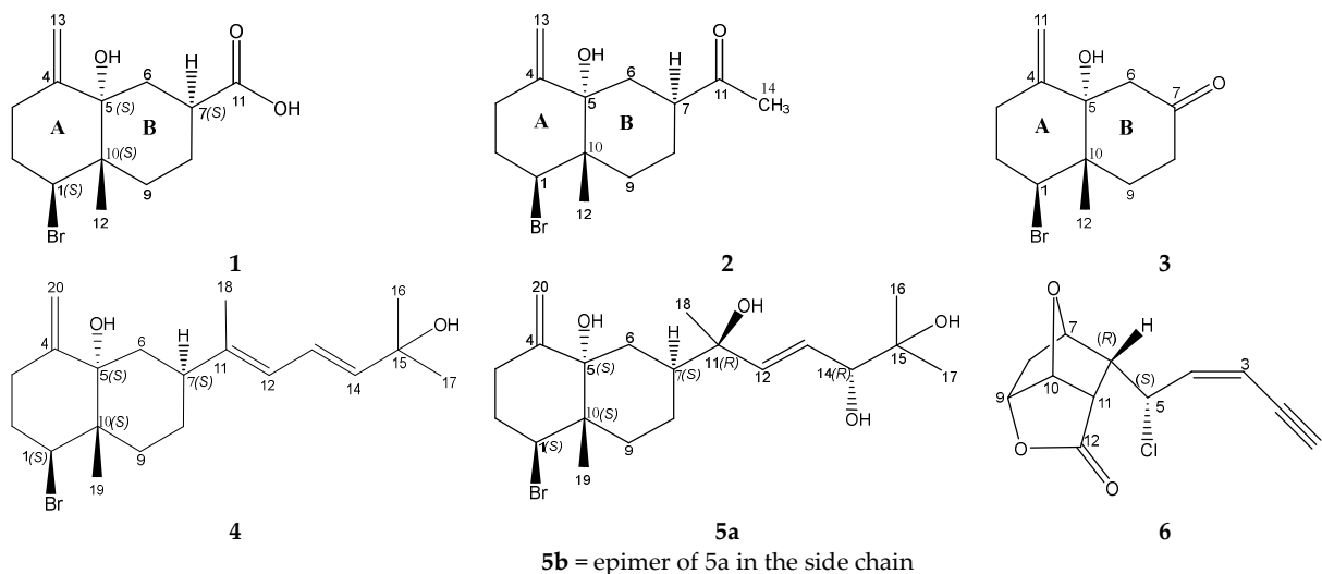
Figure 1. Structures of new haloterpenes 1–3 , 5a , 6 from L. papillosa .
