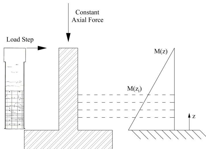
Figure 10. Bending Moment Profile M(z_i) .
