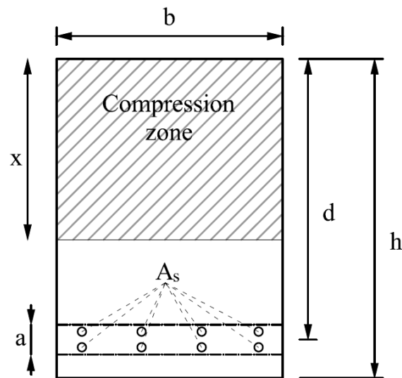
Figure 3. Geometrical parameters used in Equation (4).
