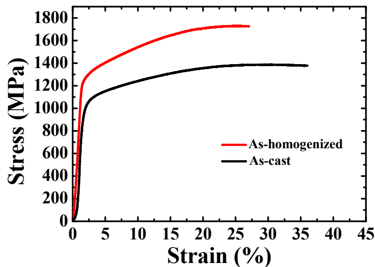
Figure 4. The compressive stress–strain curves of the as-cast and as-homogenized TiZrNbTa alloys.
