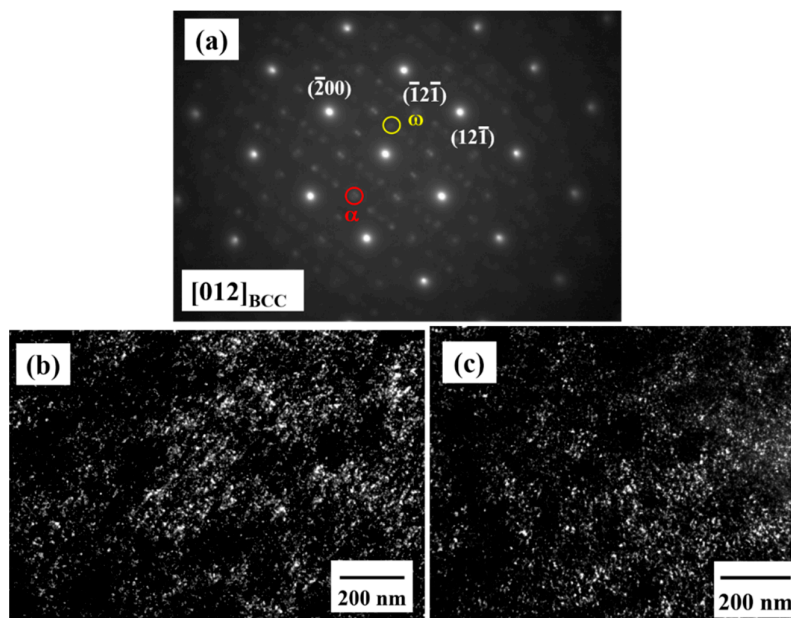
Figure 8. TEM results of the \alpha and \omega precipitates in the as-homogenized alloy: (a) SADP of the [012] BCC zone axis; (b) dark-field image taken from the \alpha spot, as highlighted by the red circle in SADP; and (c) dark-field image taken from the \omega spot, as highlighted by the yellow circle in SADP.
