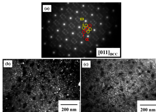
Figure 5. Transmission electron microscopy (TEM) results of the NbTa-rich region in the as-cast alloy: (a) selected area diffraction pattern (SADP) of the [011] BCC zone axis; (b) dark-field image taken from the \alpha spot, as highlighted by the red arrow in SADP; and (c) dark-field image taken from the \omega spot, as highlighted by the yellow arrow in SADP.
