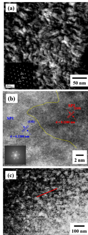
Figure 6. (a) The TEM dark-field images, (b) the corresponding high-resolution TEM images, and (c) the HAADF-STEM image of the interconnected structure in the as-homogenized alloy.
