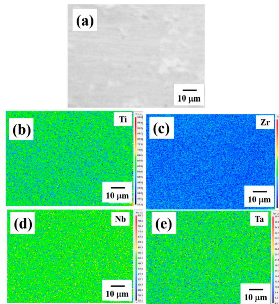
Figure 3. (a) The SEM BEI of the as-homogenized Ti 25 Zr 25 Nb 25 Ta 25 HEA, and the corresponding composition mapping for (b) Ti, (c) Zr, (d) Nb, and (e) Ta.
