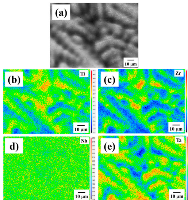
Figure 2. (a) The scanning electron microscope (SEM) back-scattered image (BEI) of the as-cast Ti 25 Zr 25 Nb 25 Ta 25 high-entropy alloy (HEA), and the corresponding composition mapping for (b) Ti, (c) Zr, (d) Nb, and (e) Ta. Note that the Nb mapping does not really expose the dendrites (DRs) and inter-dendrites (IDs) clearly. This may be attributed to the fact that the L\alpha X-ray energy of element Nb (~2.169 eV) is slightly larger than the M absorption edge energy of element Ta (~1.804 eV). Therefore, in the dendrite regions, the L\alpha X-ray energy of element Nb would be significantly absorbed, resulting in an underestimated amount of the element Nb.
