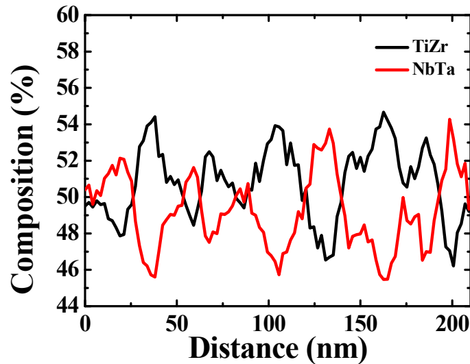
Figure 7. STEM-EDS line scan result of the spinodal interconnected structure along the red line of Figure 6c in the as-homogenized alloy.
