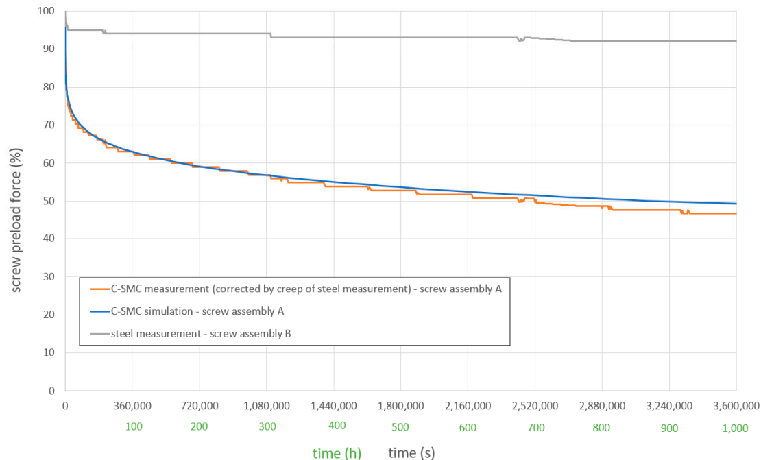
Figure 7. Loss of screw force over time.
