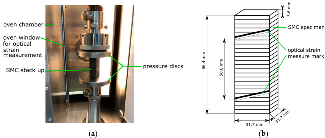
Figure 3. (a) C-SMC stackup between pressure discs in the universal testing machine; (b) C-SMC stackup in close-up view.
