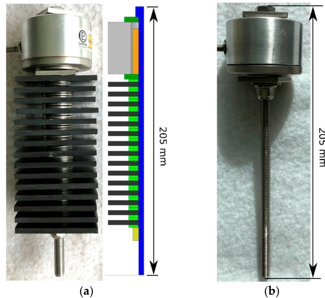
Figure 6. Screw assemblies for measurement of pretension loss; screw assembly (a) with 15 C-SMC specimens; screw assembly (b) with only steel clamped.
