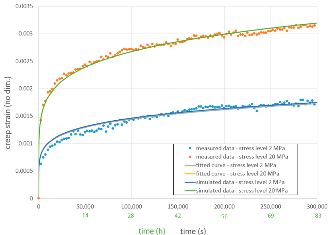
Figure 5. Measured, simulated (Section 4.1) and curve fitted creep strain–time graphs at different stress levels in z direction for “Polynt SMCarbon 80 CF60-3K/2” at 120 °C.
