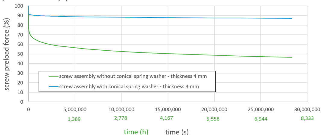
Figure 10. Simulated screw preload force over time of application-oriented screw assemblies.
