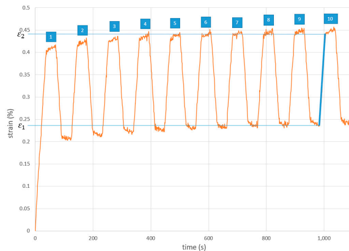
Figure 4. Alternating strains for determination of transverse modulus in z direction.
