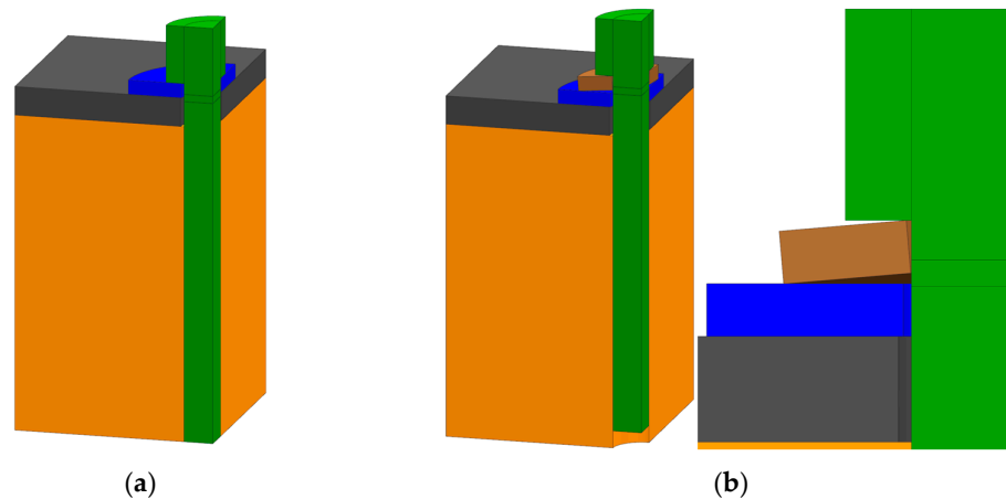
Figure 9. Application-oriented screw assemblies. (a) without conical spring washer. (assembly view); (b) with conical spring washer (assembly and detail view).
