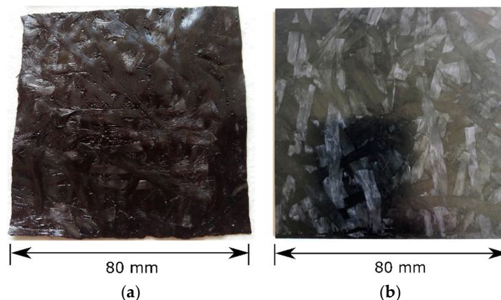
Figure 1. As-delivered (a) and pressed (b). C-SMC (carbon-fiber sheet molding compound) sheet: carbon-fiber sheet mold compound “Polynt SMCarbon 80 CF60-3K/2” [16].
