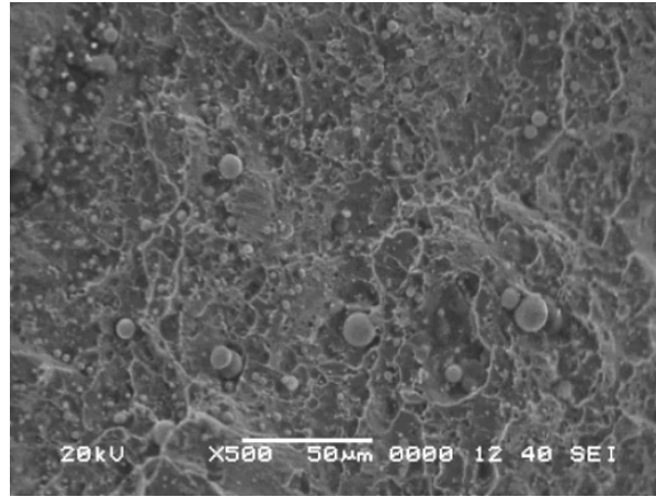
Figure 9. The fracture morphology of the experimental sample.
