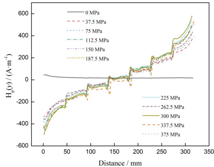
Figure 5. H_p(y) signals corresponding to different stresses.
