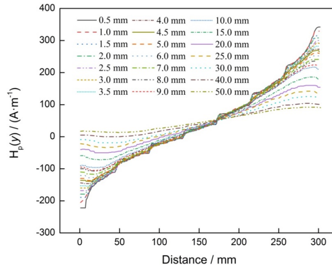
Figure 3. H_p(y) signal corresponding to different lift-offs of sensor probe.
