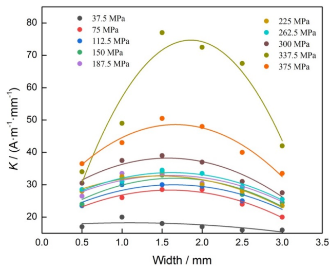
Figure 6. Relation of K and width of groove.
