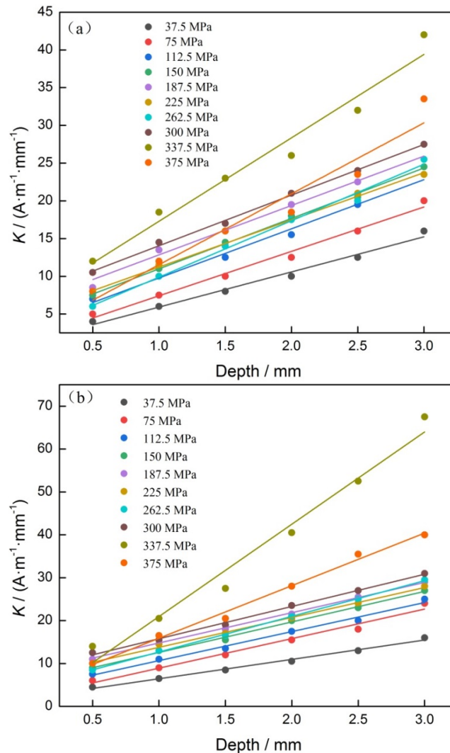
Figure 7. Relationship of K and groove depth. (a) 2.0 mm, (b) 3.0 mm.
