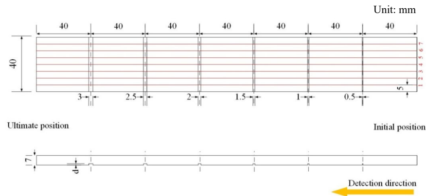
Figure 1. The sketch map of the experimental sample with regular rectangular groove.
