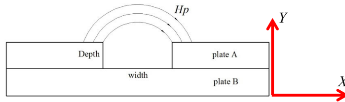
Figure 10. The leakage magnetic field model of finite depth slit.
