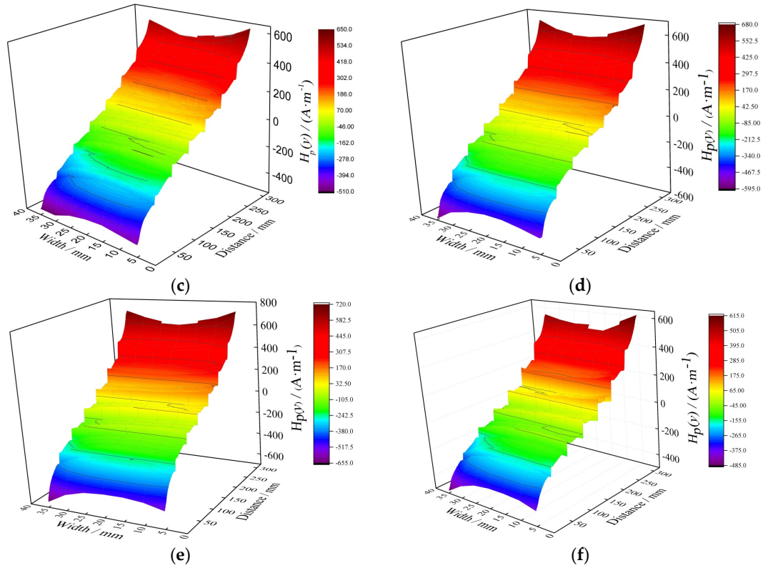
Figure 4. H_p(y) signals under different tensile loads. (a) 0 MPa, (b) 75 MPa, (c) 150 MPa, (d) 225 MPa, (e) 337.5 MPa, (f) 375 MPa.
