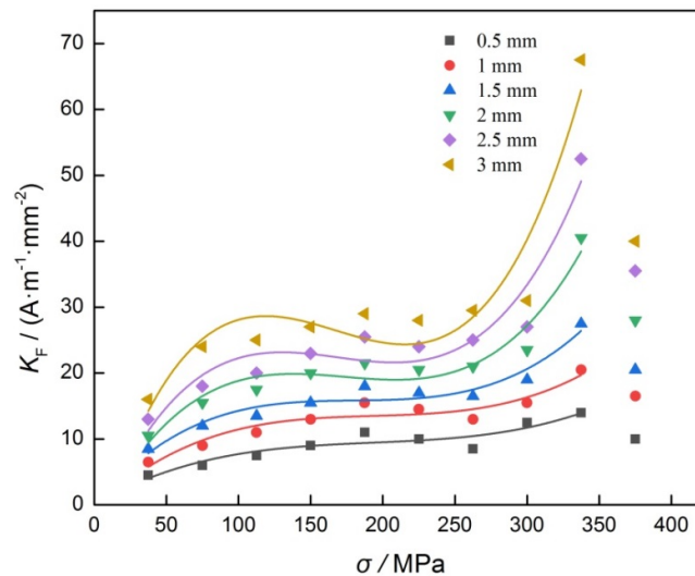
Figure 8. Result of K_F and tensile stress.
