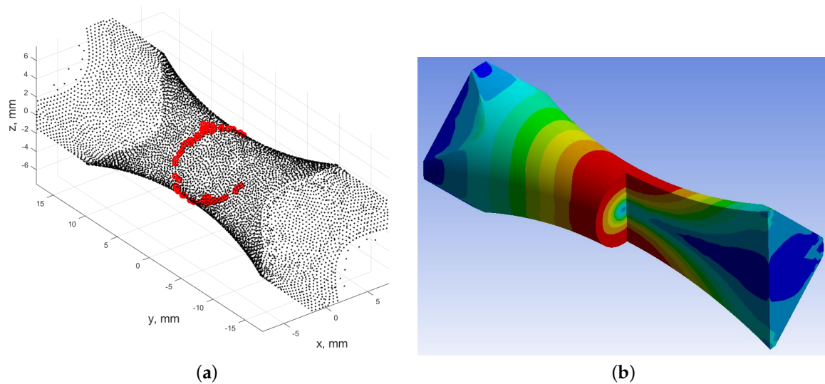
Figure 19. (a) Distribution of the most stressed mesh nodes calculated according to the von Mises criterion for in-phase kinematic loading; (b) Area of occurrence of plastic strains FEM calculated for the Chaboche cyclic plasticity model for out-of-phase kinematic loading.
