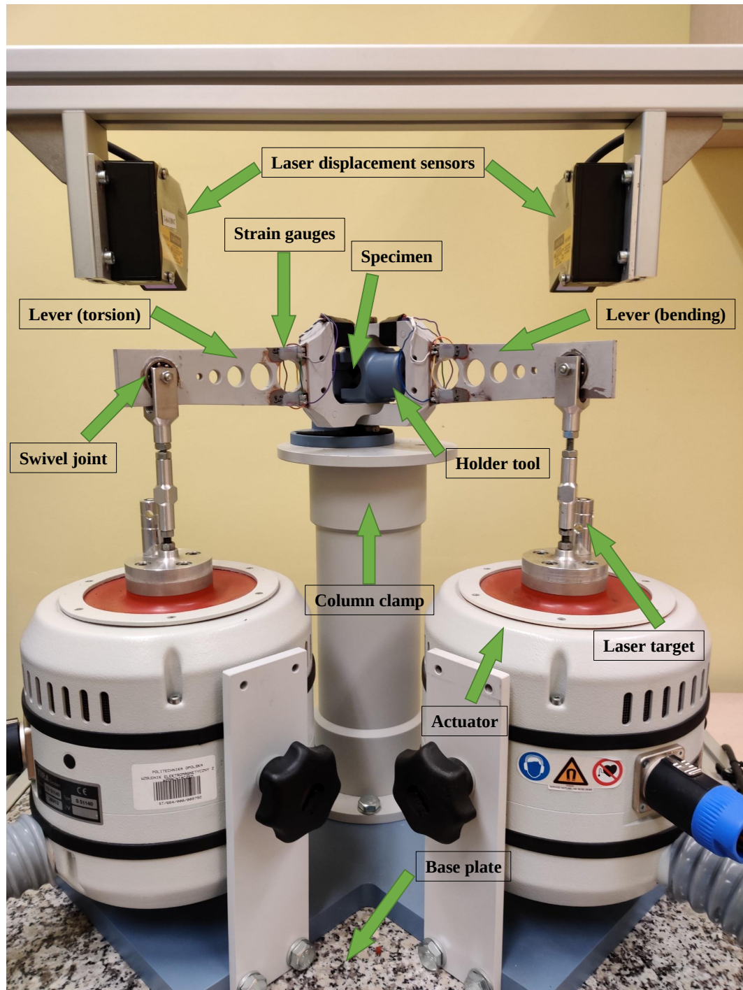
Figure 2. Fatigue testing machine.
