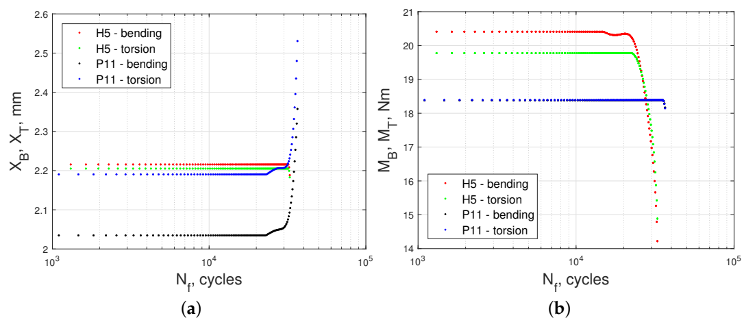
Figure 17. (a) Change in the fatigue testing machine lever displacement throughout the entire duration of the specimen test. Red and green correspond to the specimen subjected to kinematic loading, whereas black and blue correspond to the fatigue testing machine lever displacement for the specimen subjected to dynamic loading, (b) The moments load the specimen throughout the entire test period. Red and green correspond to the specimen subjected to kinematic loading, whereas black and blue correspond to the specimen subjected to dynamic loading.
