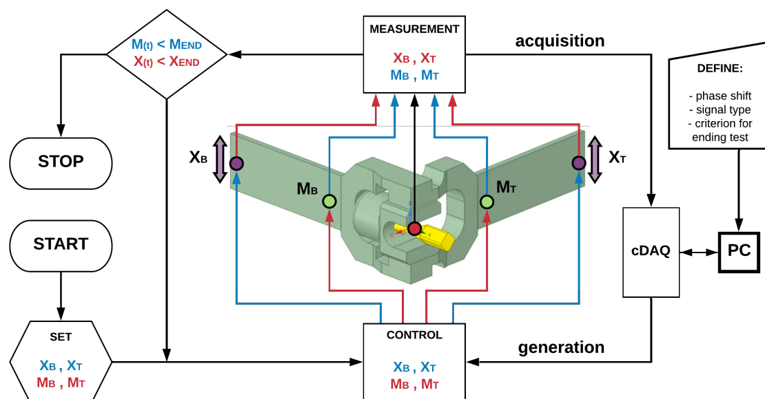
Figure 3. Fatigue machine control and conditioning system.
