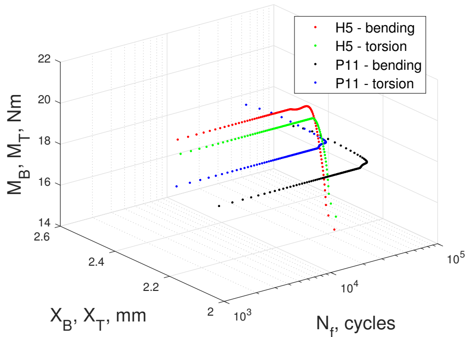
Figure 16. Change in recorded values of bending and torsional moments of specimen No. H5 during the entire test period under kinematic load (red and green) and change in the value of the machine lever displacement for dynamic load for specimen no. P11, black and blue.
