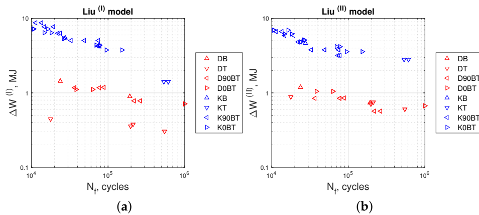
Figure 14. (a) Liu (I) model (7), (b) Liu (II) model (8). Tests at kinematic load: K90BT, out of phase; K0BT, in phase; KB, bending; KT, torsion. Dynamic loads: D90BT, out of phase; D0BT, in phase; DB, bending; DT, torsion.
