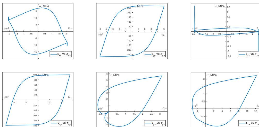
Figure 6. Numerical obtained hysteresis loops for in-phase kinematic load.
