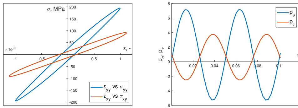
Figure 12. Stabilized calculated hysteresis loops for dynamic out-of-phase load and calculated instantaneous power (bending) p_\sigma and torsion p_\tau .
