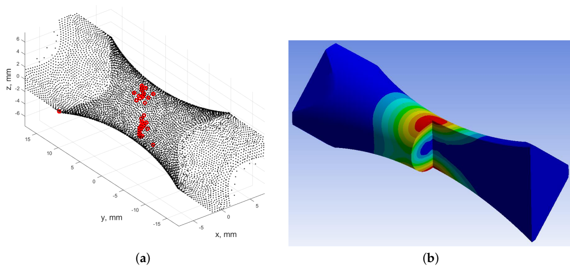
Figure 18. (a) Distribution of the most stressed mesh nodes calculated according to the von Mises criterion for in-phase kinematic loading; (b) Area of occurrence of plastic strains finite element method (FEM) calculated for the Chaboche cyclic plasticity model for in-phase kinematic loading.
