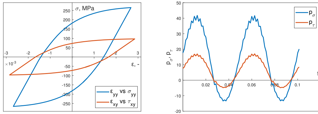
Figure 9. Stabilized calculated hysteresis loops for kinematic in-phase load and calculated instantaneous power (bending) p_\sigma and torsion p_\tau .
