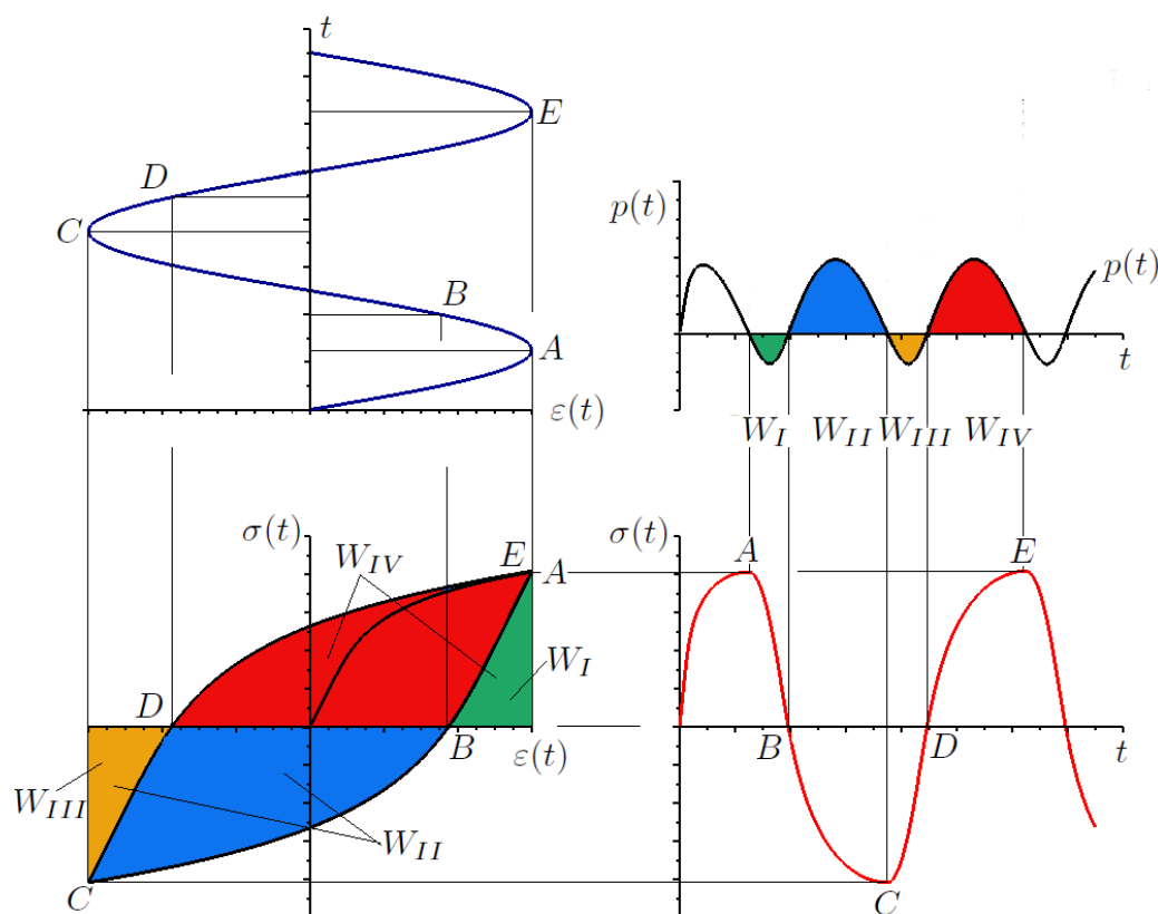
Figure 8. Method of calculating the elastic-plastic strain energy density by integrating the time course of instantaneous power.
