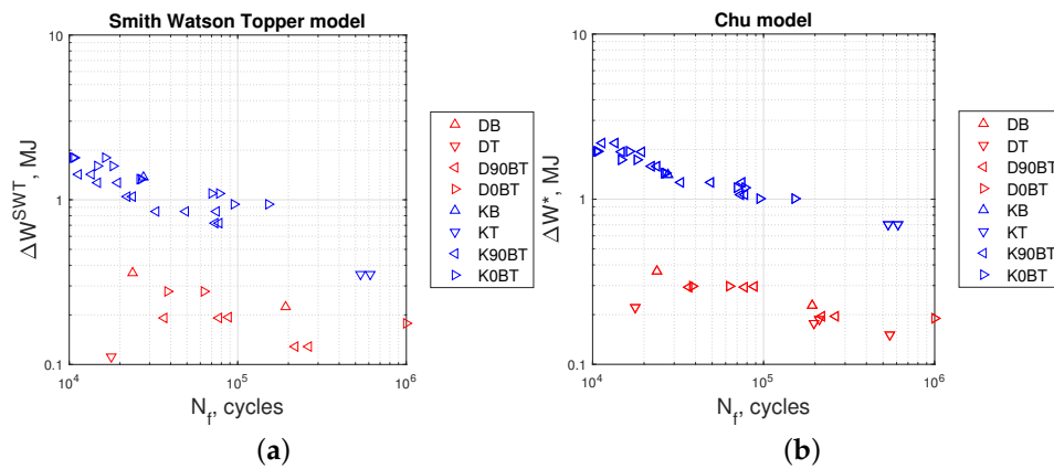
Figure 13. (a) Smith Watson Topper model in Equation(5), (b) Chu model in Equation (6). Tests at kinematic load: K90BT, out of phase; K0BT, in phase; KB, bending; KT, torsion. Dynamic loads: D90BT, out of phase; D0BT, in phase; DB, bending; DT, torsion.
