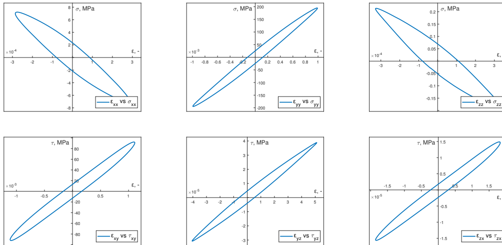
Figure 7. Numerically calculated hysteresis loops for out-of-phase dynamic load.
