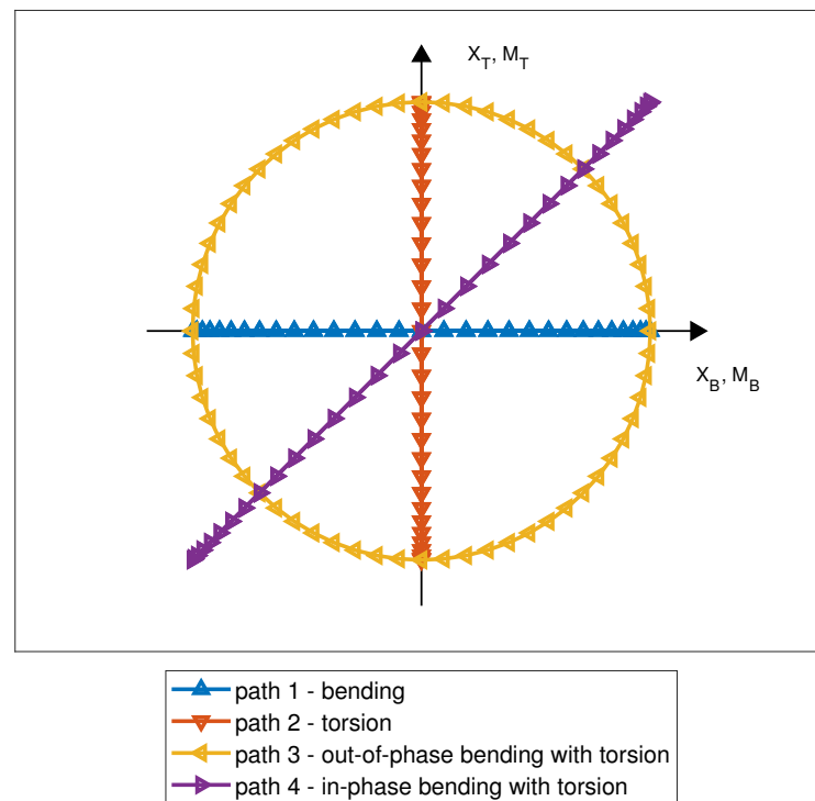
Figure 4. Loading paths.
