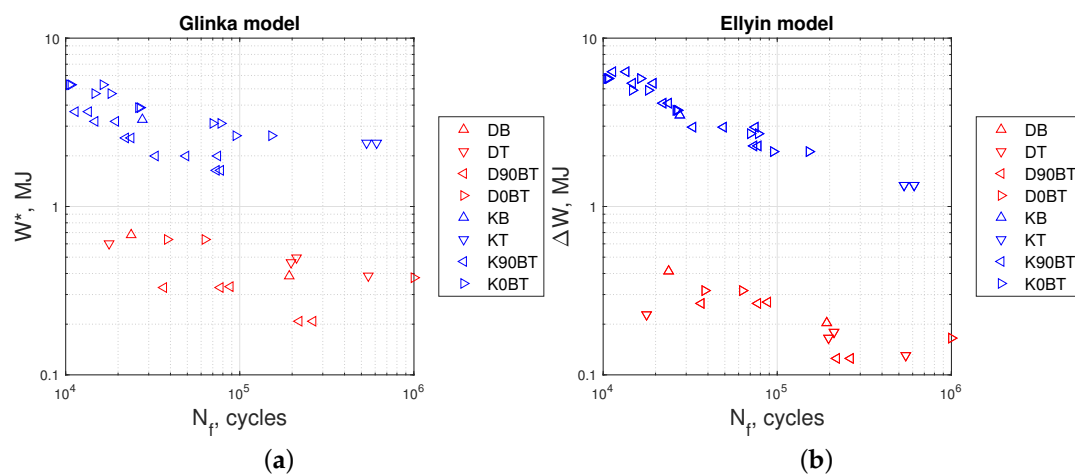
Figure 15. (a) Glinka parameter in Equation (9), (b) Ellyin energy parameter in Equation (11). Tests at kinematic load: K90BT, out of phase; K0BT, in phase; KB, bending; KT, torsion. Dynamic loads: D90BT, out of phase; D0BT, in phase; DB, bending; DT, torsion.
