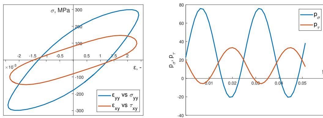
Figure 10. Stabilized calculated hysteresis loops for kinematic out-of-phase load and calculated instantaneous power (bending) p_\sigma and torsion p_\tau .
