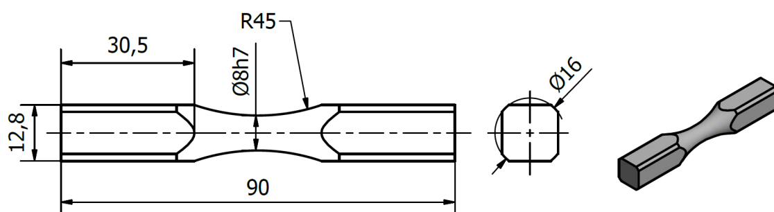
Figure 1. Test specimen. All dimensions are provided in millimeters.
