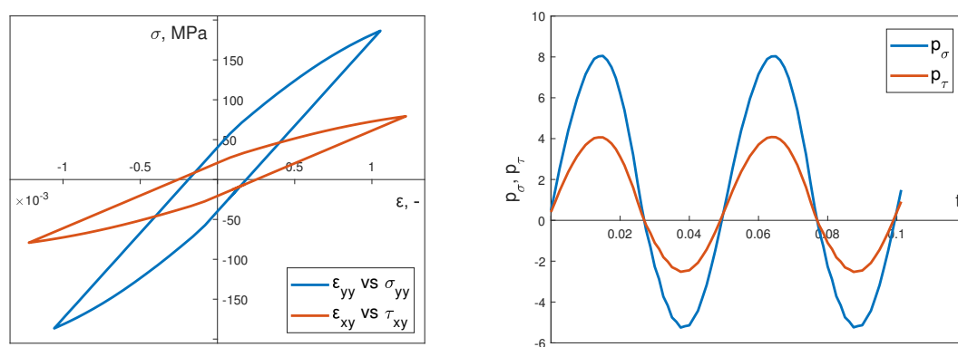
Figure 11. Stabilized calculated hysteresis loops for dynamic in-phase load and calculated instantaneous power (bending) p_\sigma and torsion p_\tau .
