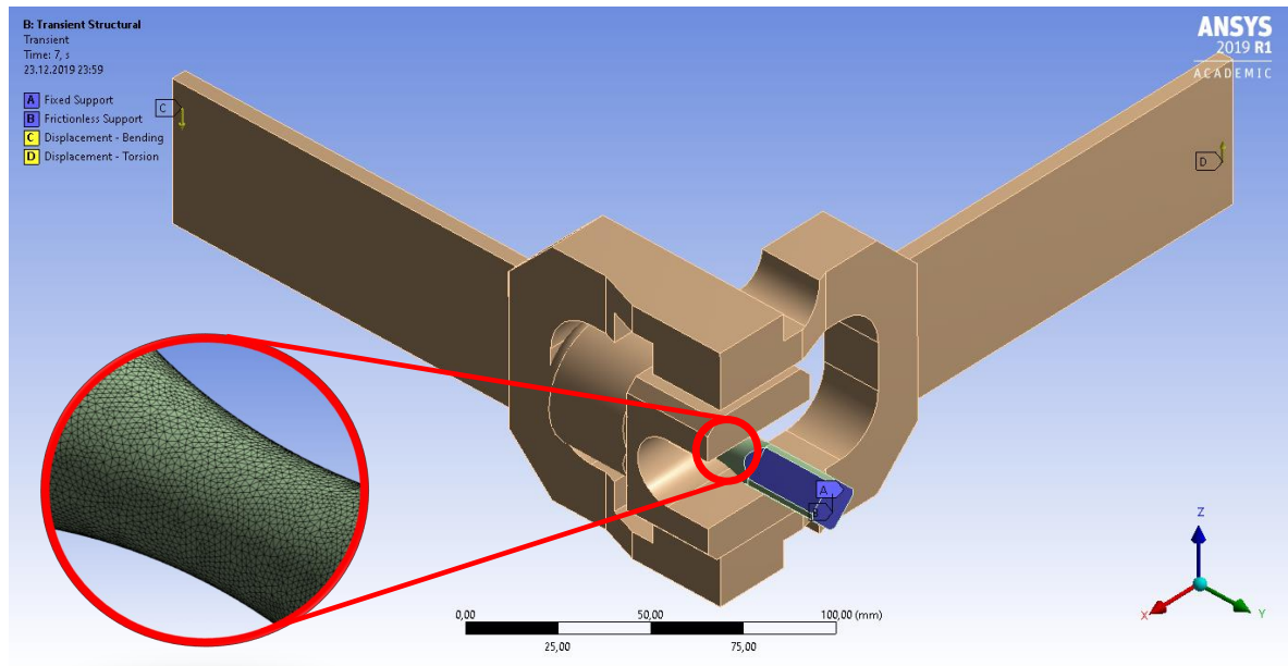
Figure 5. Numerical model of clamping/loading system of the fatigue machine.
