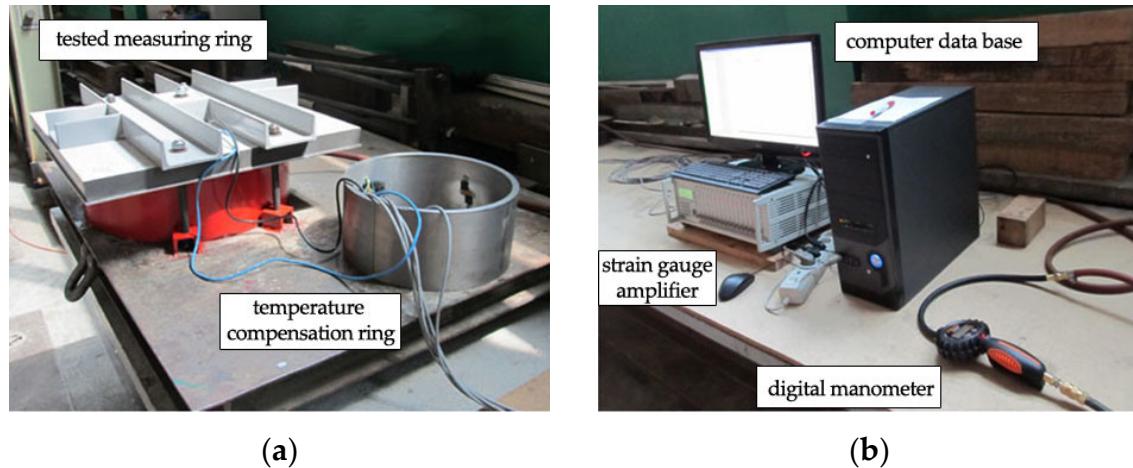
Figure 4. Components of the calibration system: (a) measuring rings during the test; (b) registration of the strain and air pressure.
