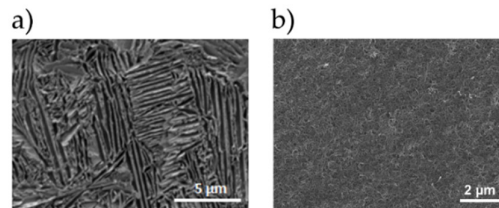
Figure 3. SEM images of Ti13Nb13Zr alloy before laser treatment. (a) MR; (b) MR with MWCNTs coatings.
