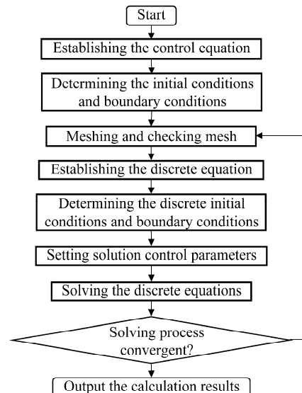
Figure 5. Flow chart of computational fluid dynamics (CFD) calculation.
