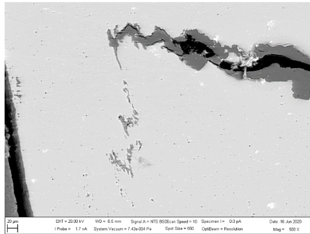
Figure 14. Details of cracks and mixing of materials.
