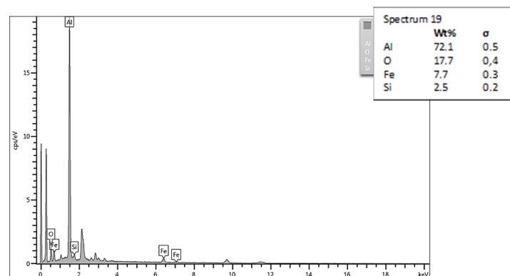
Figure 19. Energy dispersive X-ray (EDS)—spectrum 19.
