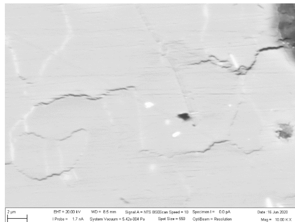
Figure 16. Details of small cracks.
