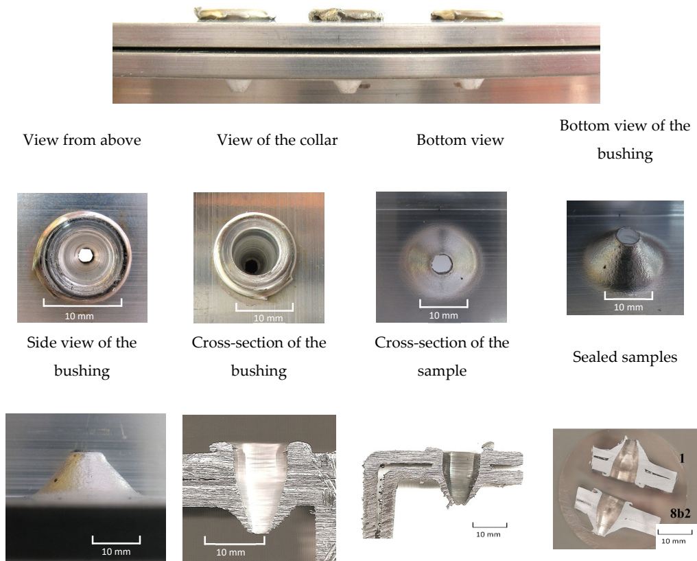
Figure 7. Visuals evaluation of the collar and bushing created from double layers of the AL alloy—Al Mg Si.
