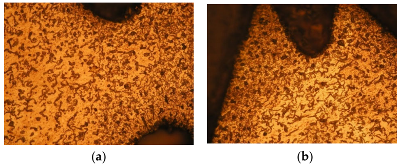
Figure 10. Details of the microstructures of the tapped threads, Magn. 200×. (a) Collar deformation and thread. (b) End of thread.
