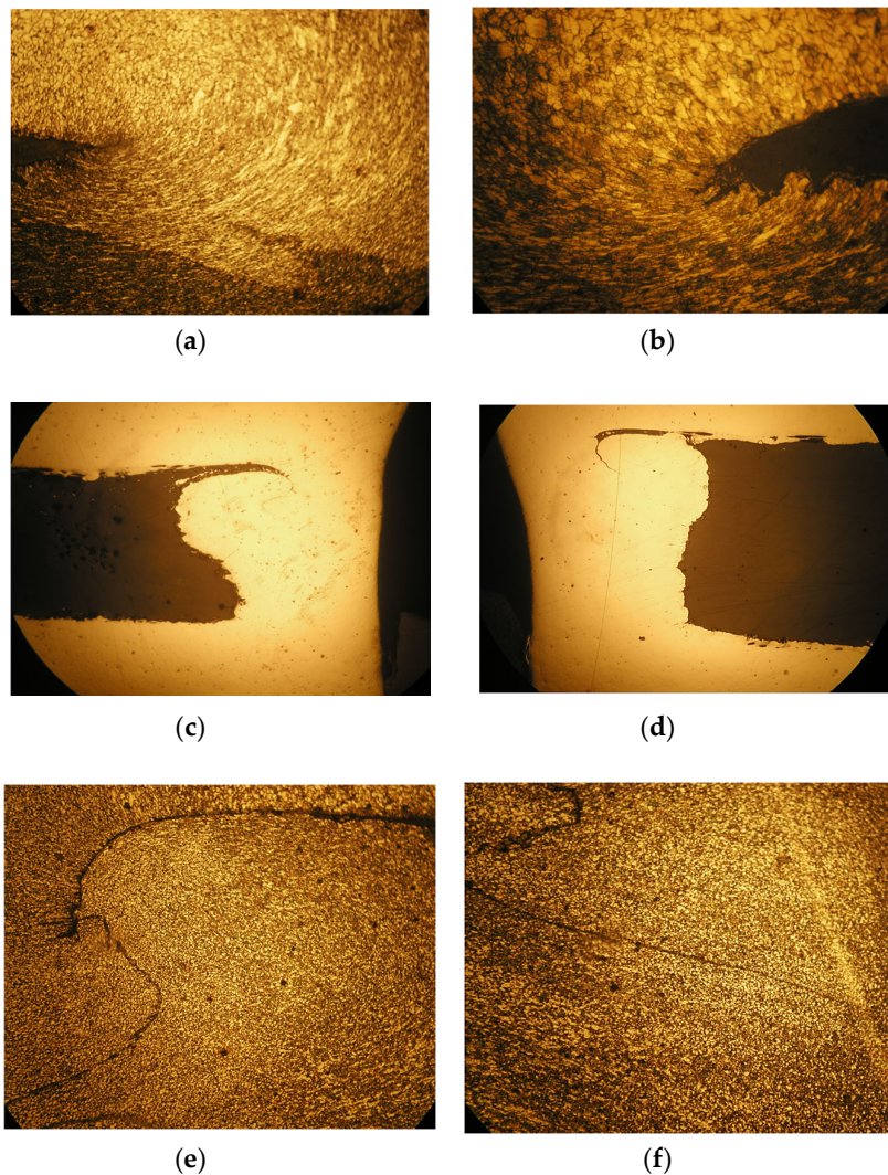
Figure 11. Macrostructures and microstructures of the created collar and bushing from two layers of the testing material. (a) Microstructure of collar – left part, Mag. 200×. (b) Microstructure of collar – right part, Mag. 200×. (c) Macrostructure of bushing left part, Mag. 50×. (d) Macrostructure of bushing right part, Mag. 50×. (e) Microstructure of bushing left part, Mag. 200×. (f) Microstructure of bushing right part, Mag. 200×.
