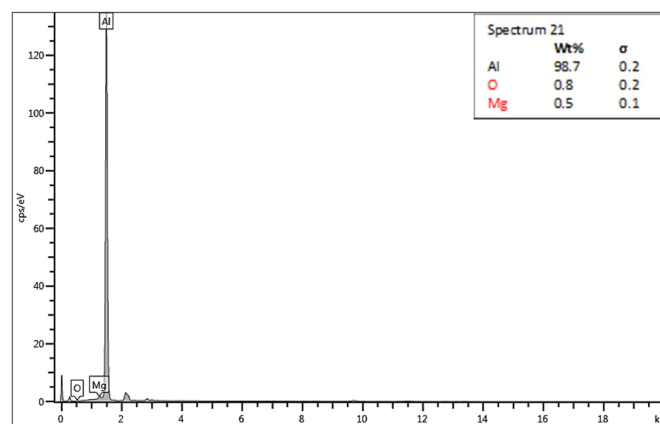
Figure 21. Energy dispersive X-ray (EDS)—spectrum 21
