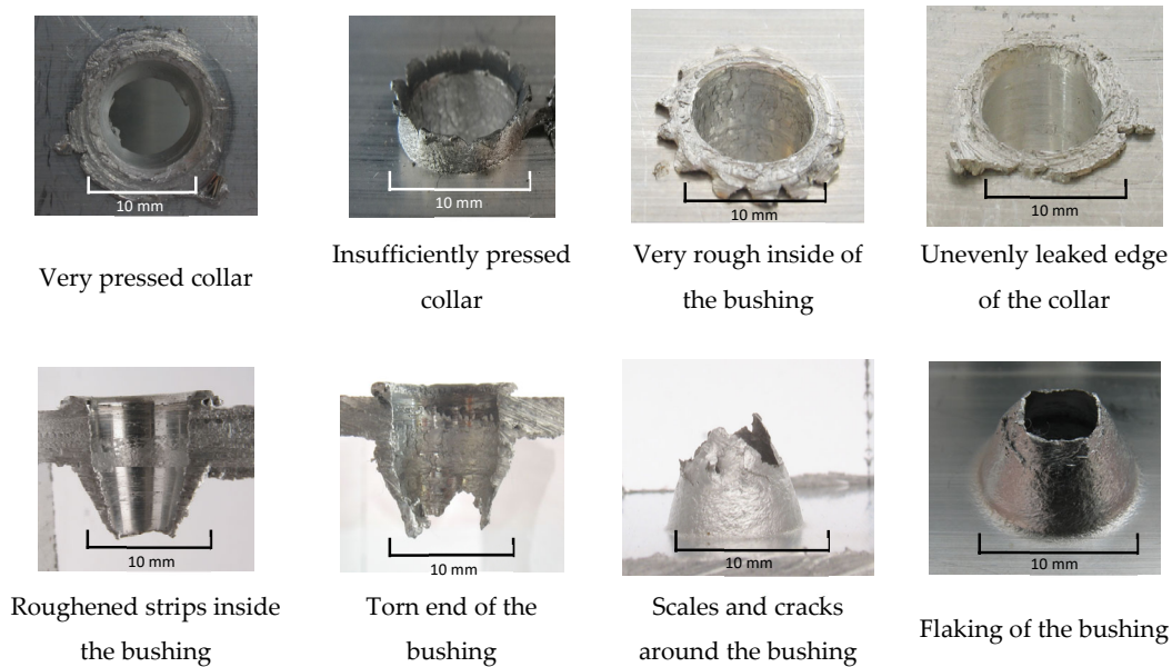
Figure 8. The possible imperfections during the creation of samples.
