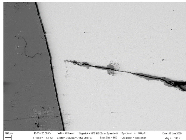
Figure 13. Creation of the crack in the joint.
