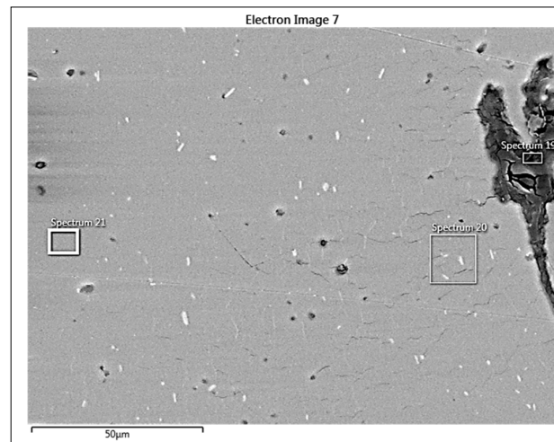
Figure 18. The chosen places for EDS evaluation.
