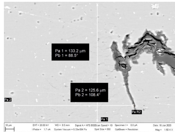
Figure 17. The measured area of the determined place with small cracks.
