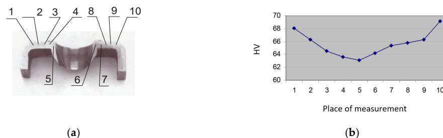
Figure 22. Microhardness: (a) Measuring places 1 and 10—basic material; 2, 3 and 8, 9—heat-affected material; 4 and 7—deformed material under the collar; and 5 and 6—deformed material in bushing. (b) Measured values.
