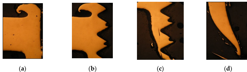
Figure 9. Visual evaluation of the macrostructure of the tested sample, Magn. 50×. (a) Collar and part of the polygon-shaped bushing. (b) Collar and cut threads in the polygon. (c) Cross-cut of the end of the bushing with threads. (d) Cross-cut of the end of the bushing.
