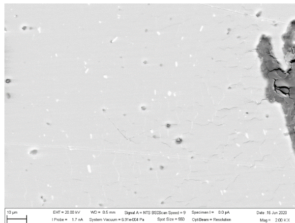
Figure 15. Creation of small cracks in front of the division of the material into two layers.
