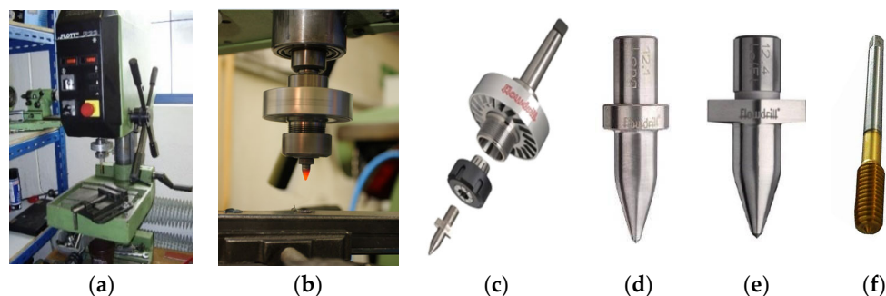
Figure 3. The used drilling machine and tools: (a) Flott P2; (b) details of the fastened friction drilling (FD) tool; (c) the FD tool with a cooling disc; (d) FD tool short; (e) FD tool short with a milling cutter; (f) tapping tool.
