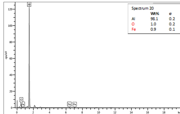
Figure 20. Energy dispersive X-ray (EDS)—spectrum 20.
