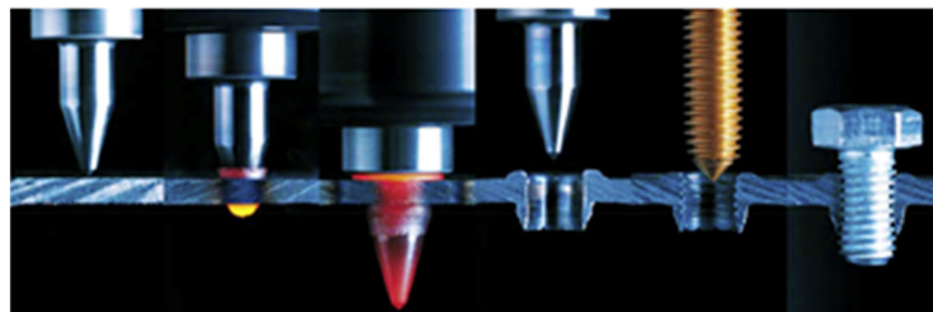
Figure 2. Thermal drilling and tapping processes [23].
