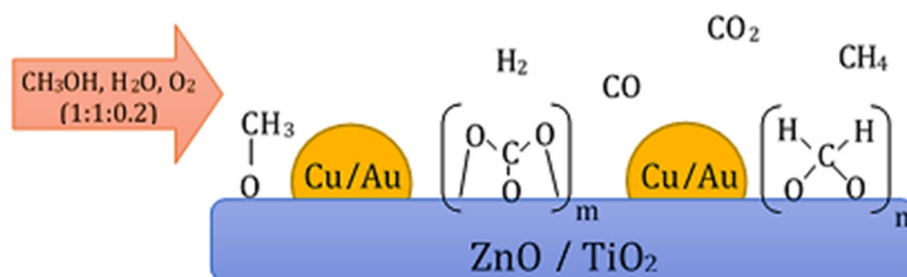
Figure 10. The species formed during the combined reforming of methanol process [117].
