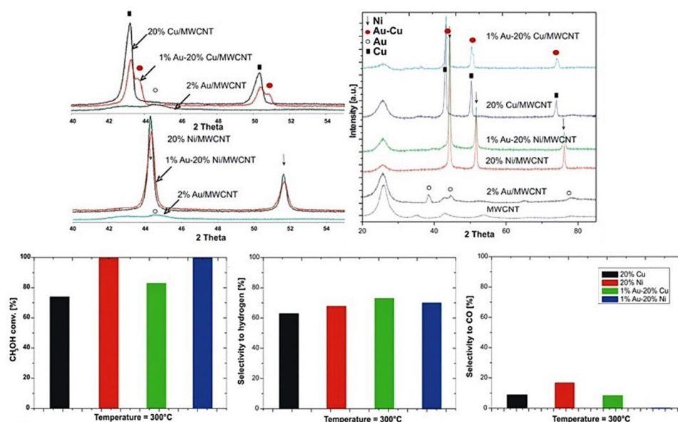
Figure 9. Phase composition studies of spent catalysts and reactivity results of bimetallic Au–Cu and Au–Ni system in the OSRM process [17].
