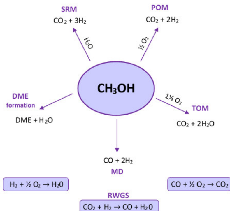
Figure 3. The possible reactions for the autothermal reforming of methanol process [24].
