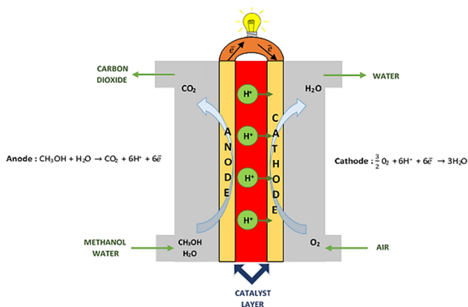
Figure 2. Direct methanol fuel cells (DMFC).
