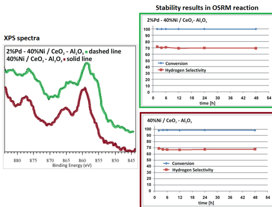
Figure 7. XPS and stability results during 48 h of the OSRM reaction performed at 250 °C after reduction 1 h at 300 °C [23].
