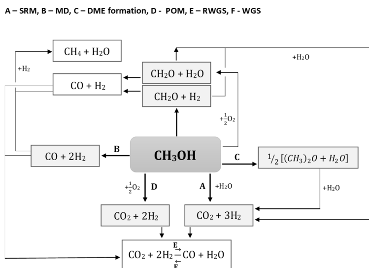
Figure 5. The reaction network taking place during oxidative steam-reforming of methanol (OSRM) process [48].
