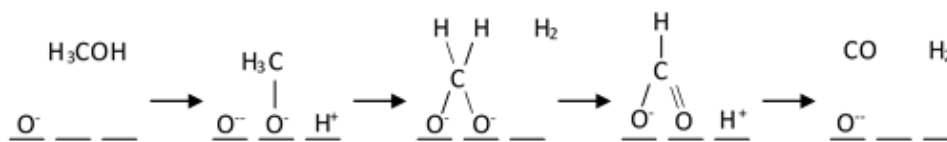
Figure 6. The methanol decomposition (MD) mechanism [60].
