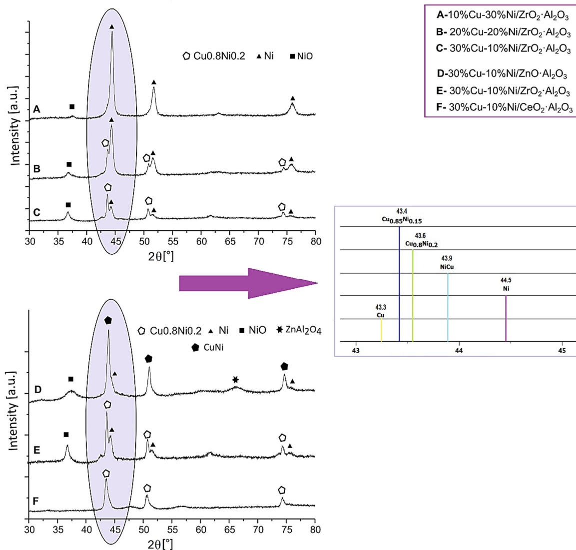
Figure 11. XRD patterns of spent bimetallic Cu–Ni systems [4].
