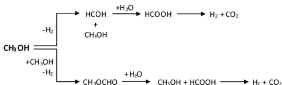
Figure 4. The reaction steps taking place during the steam-reforming of methanol process [69].
