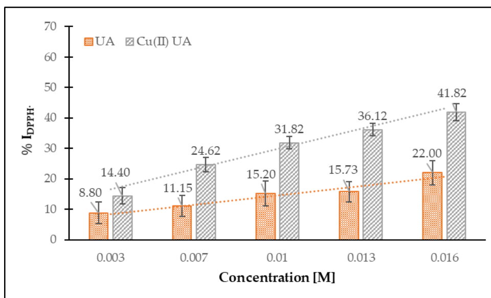
Figure 9. Percent of inhibition of DPPH• radicals by ursolic acid (UA) and Cu (II) complex of ursolic acid (Cu (II) UA), depending on their concentration (0.003–0.016 M).
