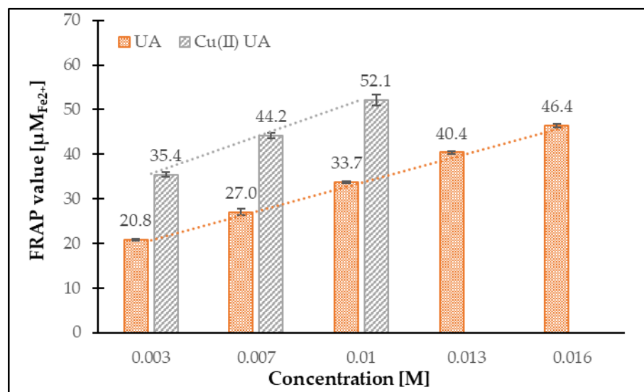
Figure 12. The ferric-reducing antioxidant activity of UA and Cu (II) UA in the concentration range 0.003–0.016 M.
