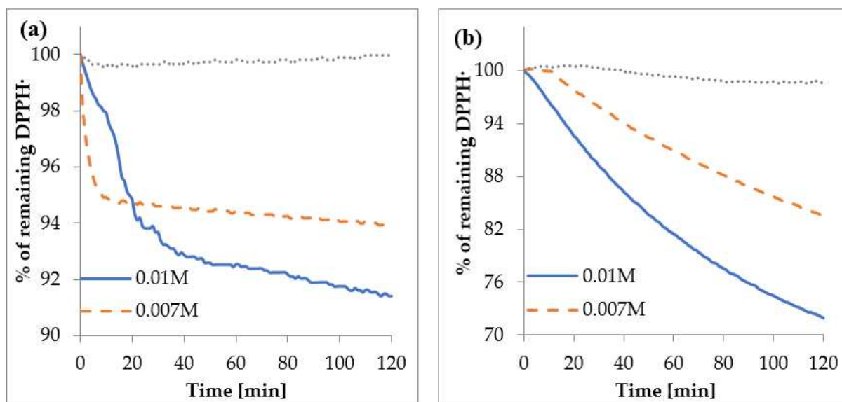
Figure 10. The percent of remaining DPPH• vs. time in the presence of (a) UA and (b) Cu (II) UA.
