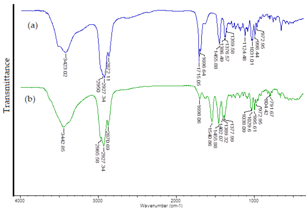
Figure 8. The FTIR spectra of ursolic acid (a) and Cu (II) complex of ursolic acid (b) registered for solid samples in the KBr matrix pellet.
