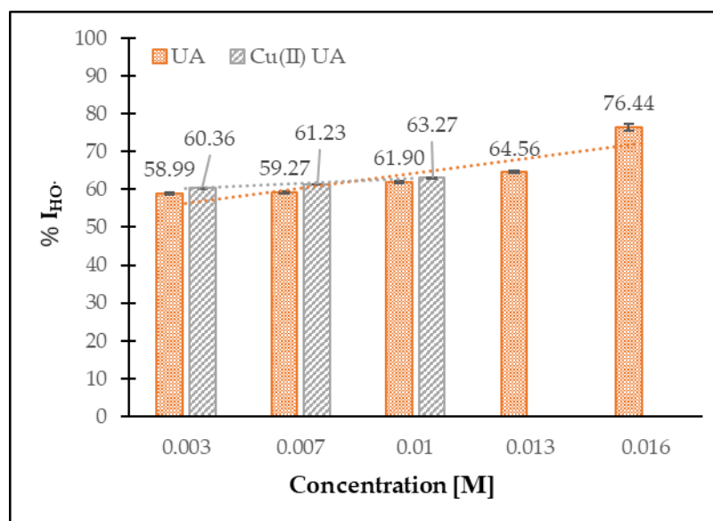
Figure 11. The percentage of HO• inhibition by UA and Cu (II) UA at the concentration range of 0.003–0.016 M.
