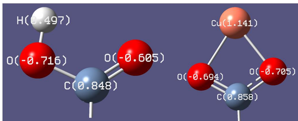
Figure 3. The distribution of NBO atomic charges in the carboxyl group in ursolic acid and carboxylate anion in metal complex calculated at B3LYP/6-31G(d) level.
