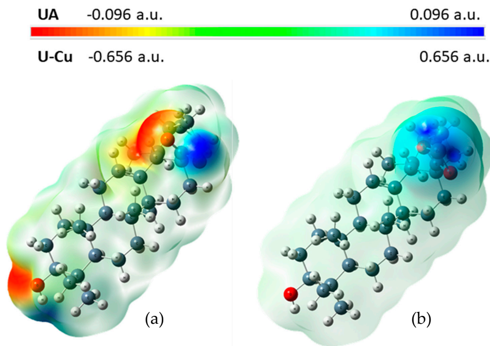
Figure 5. Molecular electrostatic potential map (MEP) for UA (a) and Cu (II) UA (b).
