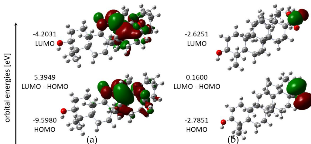
Figure 4. HOMO and LUMO energy orbitals of UA (a) and Cu(II) UA (b).
