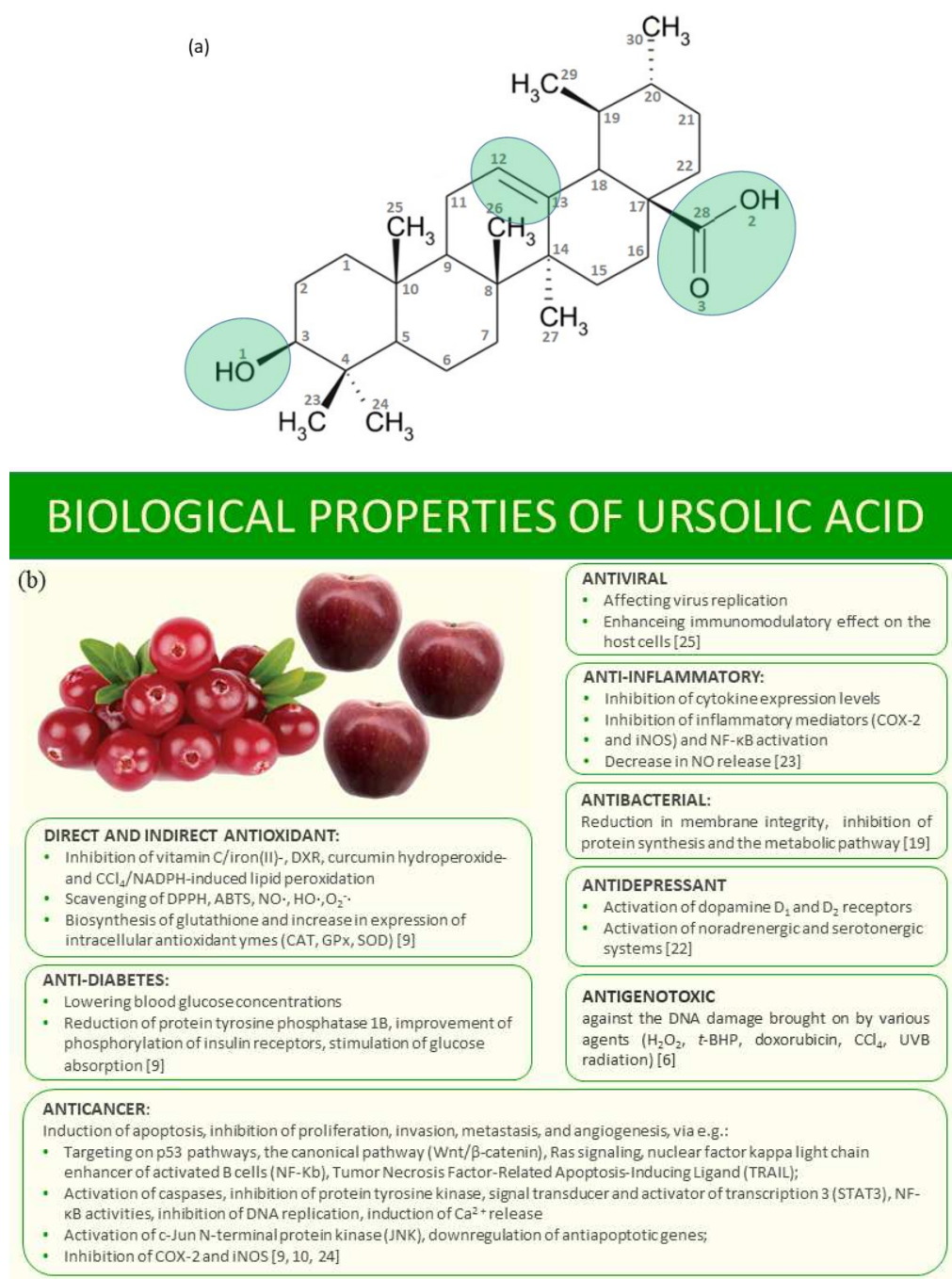
Figure 1. The scheme of ursolic acid, with marked active sites (a) and its biological properties (b).
