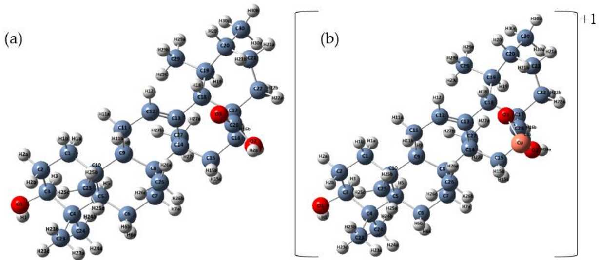
Figure 2. Optimized structures of ursolic acid (a) and cation (+1) complex of Cu (II) (b) calculated at B3LYP/6–31G (d) level.
