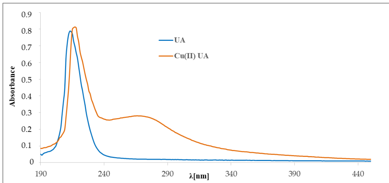
Figure 6. The UV spectra of ursolic acid and Cu (II) UA complex (0.05 mM).
