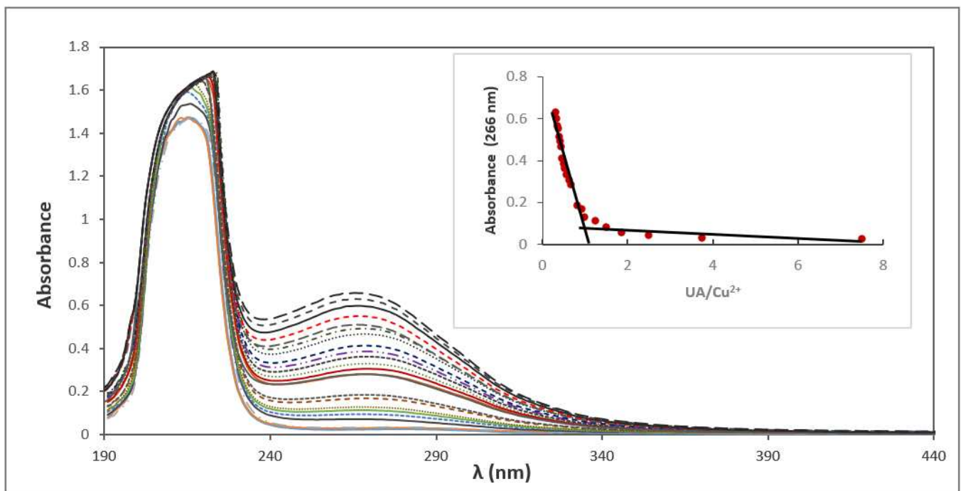
Figure 7. Spectrophotometric titration of methanolic solution of ursolic acid by Cu (II). Inset: complex absorbance at 266 nm versus [\text{UA}]/[\text{Cu (II)}] .
