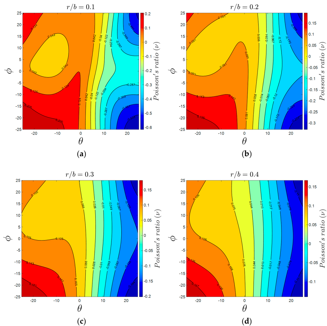
Figure 13. Variations of Poisson's ratio with respect to \theta and \phi : (a) r/b = 0.1 , (b) r/b = 0.2 , (c) r/b = 0.3 , and (d) r/b = 0.4 .
