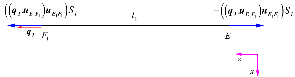
Figure 6. Deformation of strut EF due to q_1 = 1 .
