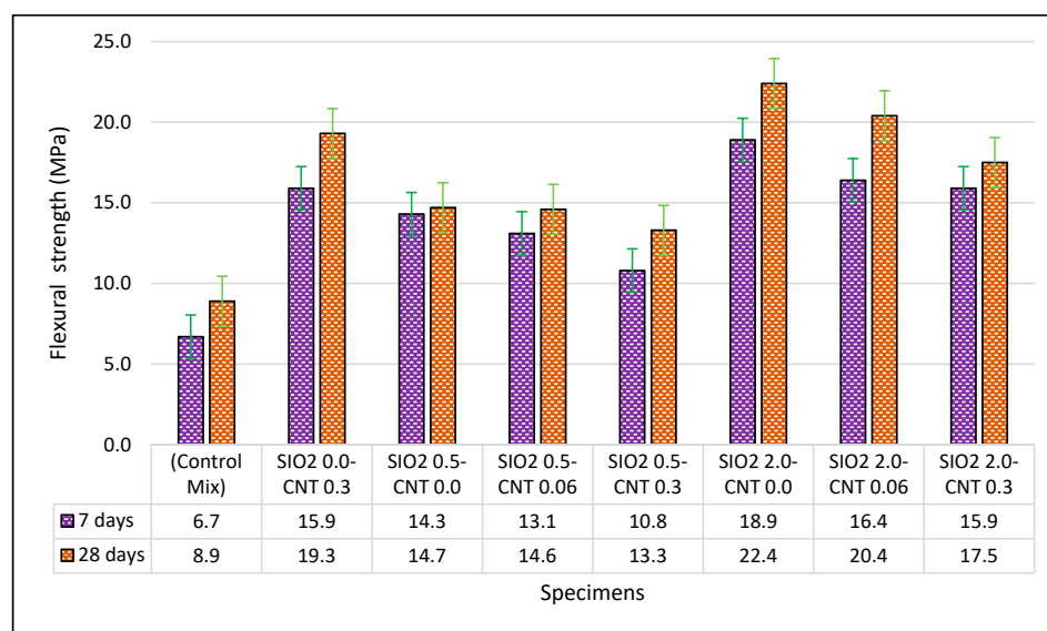
Figure 4. Flexural strength of cement paste specimens at the ages of 7 and 28 days.
