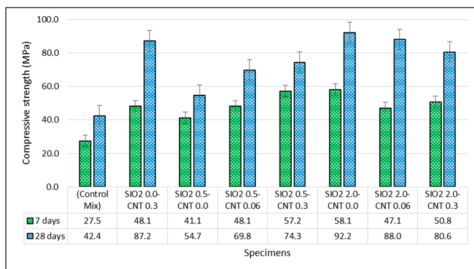
Figure 3. Compressive strength of cement paste specimens at the ages of 7 and 28 days.
