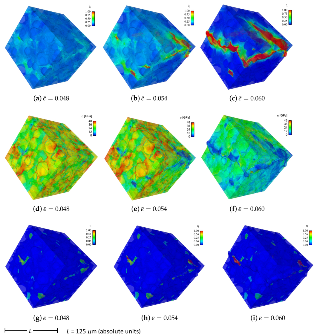
Figure 4. Stress and order parameter fields for simulation a.1.y (70% diamond, mixed SiC grains and matrix, SiC GB layers): (a) fracture order parameter \zeta , \bar{\epsilon} = 0.048 , (b) fracture order parameter \zeta , \bar{\epsilon} = 0.054 , (c) fracture order parameter \zeta , \bar{\epsilon} = 0.060 , (d) effective stress \sigma , \bar{\epsilon} = 0.048 , (e) effective stress \sigma , \bar{\epsilon} = 0.052 , (f) effective stress \sigma , \bar{\epsilon} = 0.060 , (g) twinning order parameter \eta , \bar{\epsilon} = 0.048 , (h) twinning order parameter \eta , \bar{\epsilon} = 0.052 , (i) twinning order parameter \eta , \bar{\epsilon} = 0.060 .
