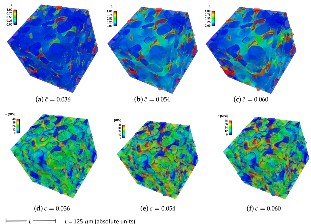
Figure 13. Stress and fracture order parameter fields for simulation c.6.x (70% diamond, mixed SiC grains and matrix, defective SiC GB layers, MD distributions for intergranular fracture energies, v_g = 0.4 , \varphi = 0.4 , total graphite fraction 5%, total porosity 8%): (a) fracture order parameter \bar{\xi} , \bar{\epsilon} = 0.036 , (b) fracture order parameter \bar{\xi} , \bar{\epsilon} = 0.054 , (c) fracture order parameter \bar{\xi} , \bar{\epsilon} = 0.060 , (d) effective stress \sigma , \bar{\epsilon} = 0.036 , (e) effective stress \sigma , \bar{\epsilon} = 0.054 , (f) effective stress \sigma , \bar{\epsilon} = 0.060 .
