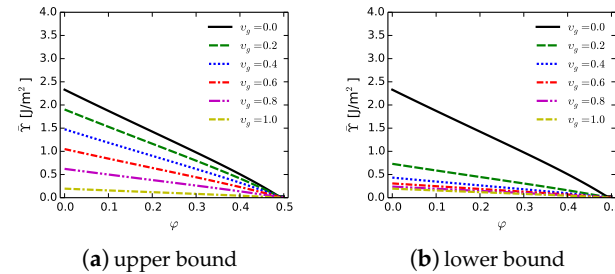
Figure 12. Effective fracture surface energy for GB phase consisting of nanocrystalline SiC, graphite ( v_g ), and/or pores ( \varphi ): (a) upper bound on \bar{Y} from (40) (b) lower bound on \bar{Y} from (40). Part (a) reproduced from [23].
