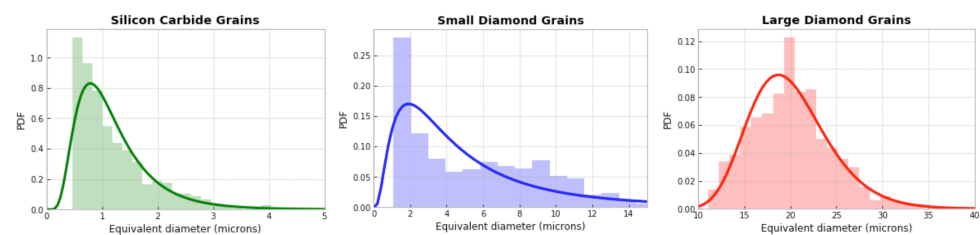
Figure 2. Grain size probability distribution functions (PDFs) for experimental diamond-SiC sample, with diamond split into two slightly overlapping sets. Curves are lognormal fits.
