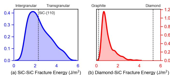
Figure 7. Sampled fracture energy distributions for (a) SiC-SiC grain boundaries and (b) diamond-SiC interfaces.
