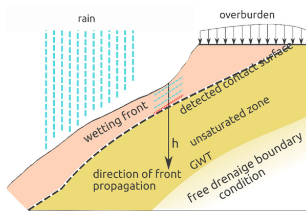
Figure 11. The task scheme (GTW—ground water table).
