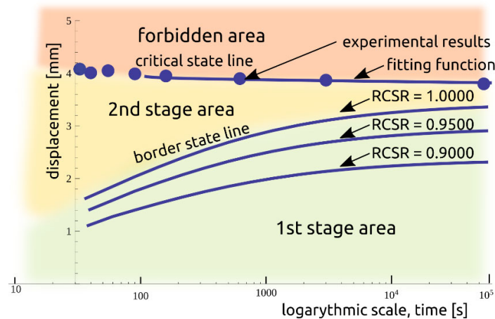
Figure 10. The contour map of creep phenomenon areas.
