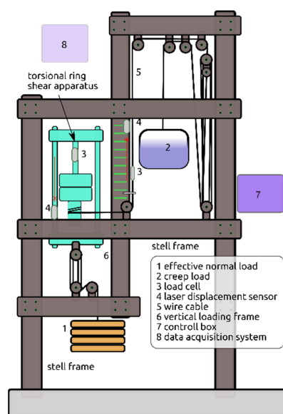
Figure 1. Structural features of creep test apparatus.
