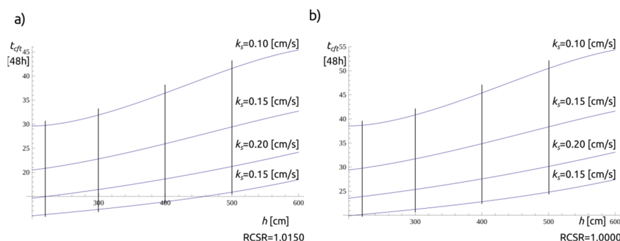
Figure 14. Values of t_{crit} at selected RCSR values and profiles (a) for RCSR = 1.0150 and (b) RCSR = 1.0000.
