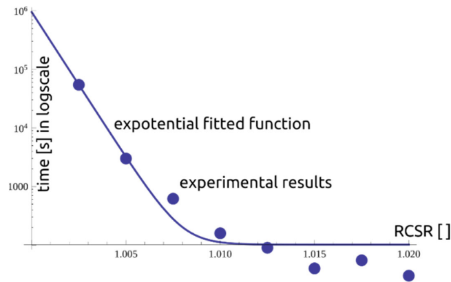
Figure 9. The dependency of RCSR vs. time.
